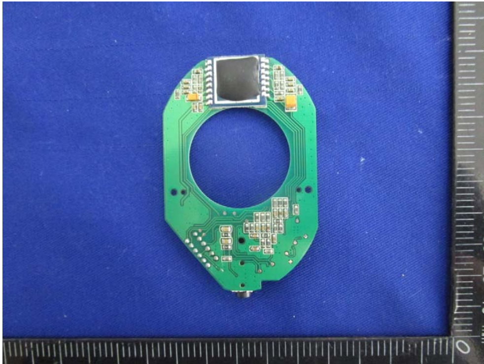
EUT –Main Board 1 Bottom View
