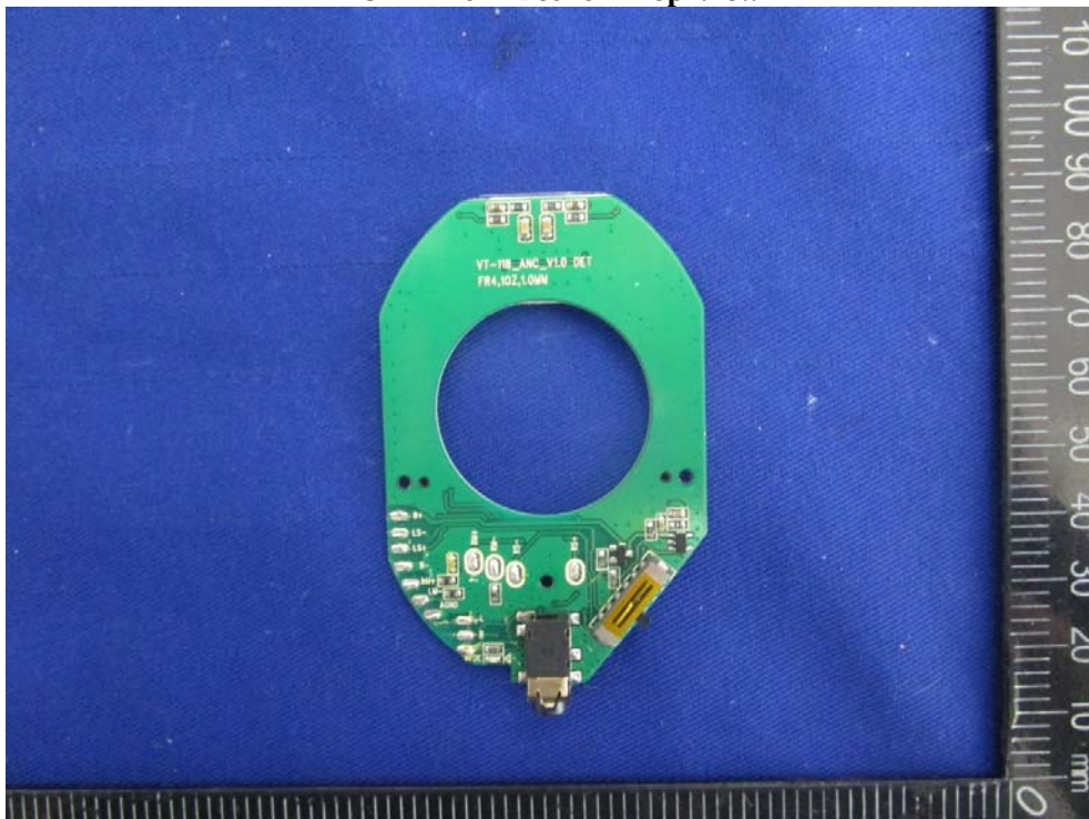
EUT – Main Board 1 Top View
