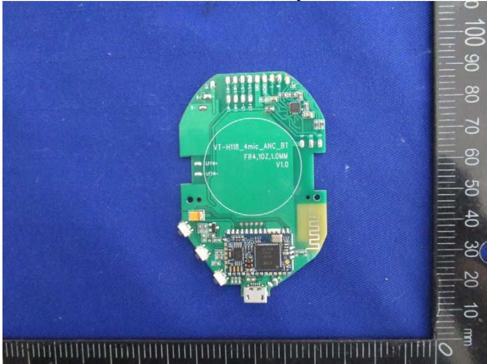
EUT –Main Board 2 Top View
