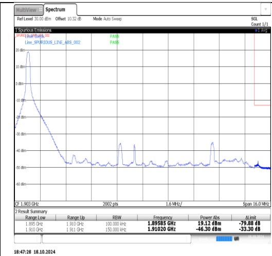
Band2-15MHz-16QAM-19125-1RB#74-PASS
