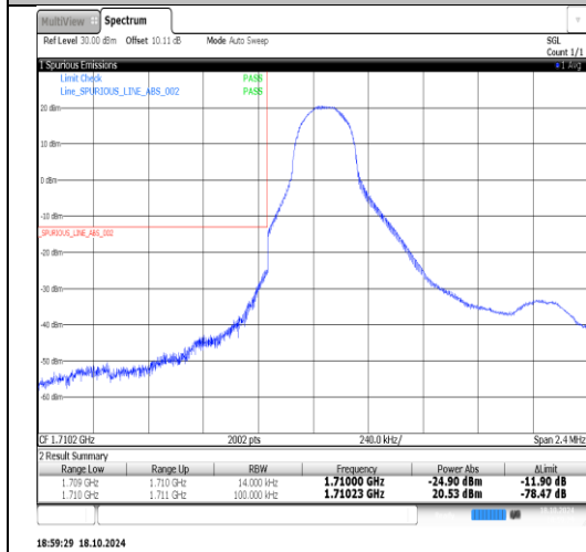
Band4-1.4MHz-QPSK-19957-1RB#5-PASS
