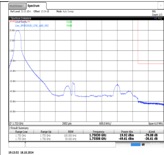
Band4-5MHz-QPSK-20375-1RB#24-PASS
