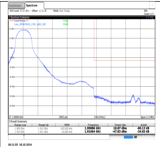
Band2-1.4MHz-16QAM-19193-1RB#5-PASS
