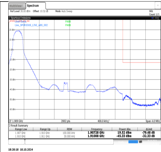
Band2-3MHz-16QAM-19185-1RB#14-PASS
