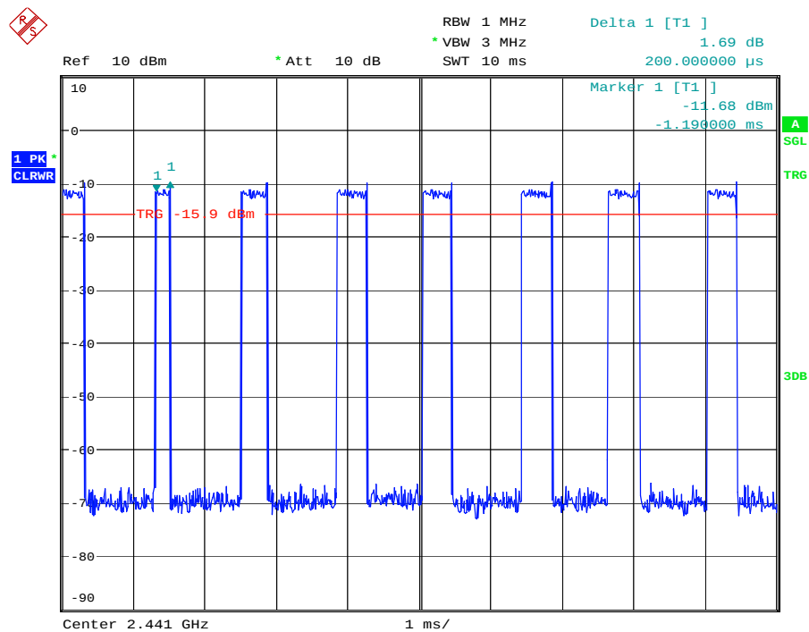
Dwell Time_3DH1_2441
