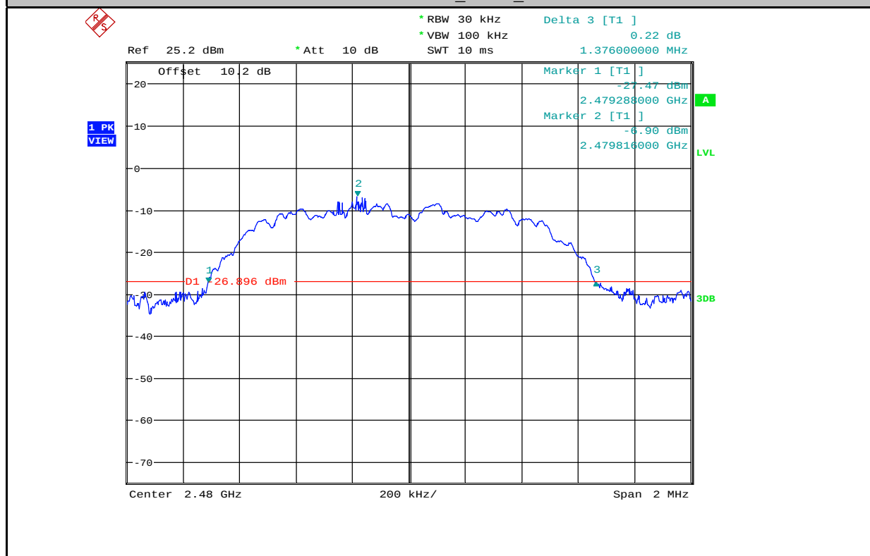
20 dB Bandwidth_3DH5_2480
