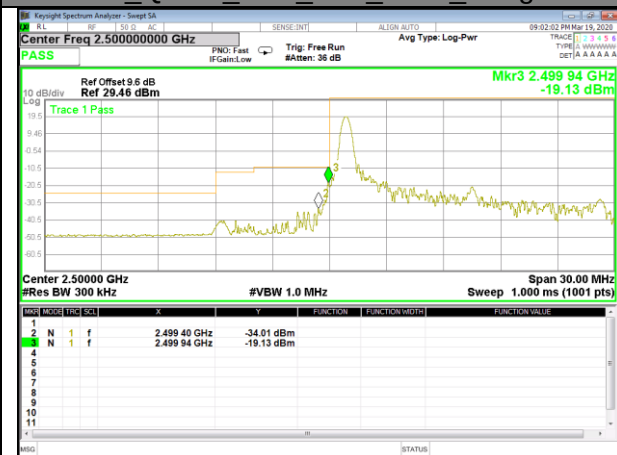
B7_QPSK_15M_Low_1-RB_Bedge
