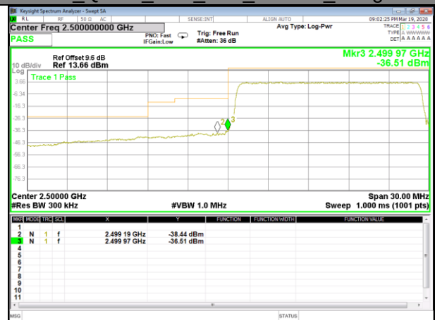
B7_QPSK_15M_Low_Full-RB_Bedge
