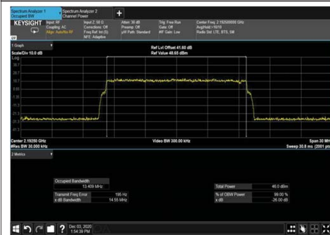
Figure 362: 16QAM 15MHz B.W; 2192.5MHz – 4G OUTPUT
