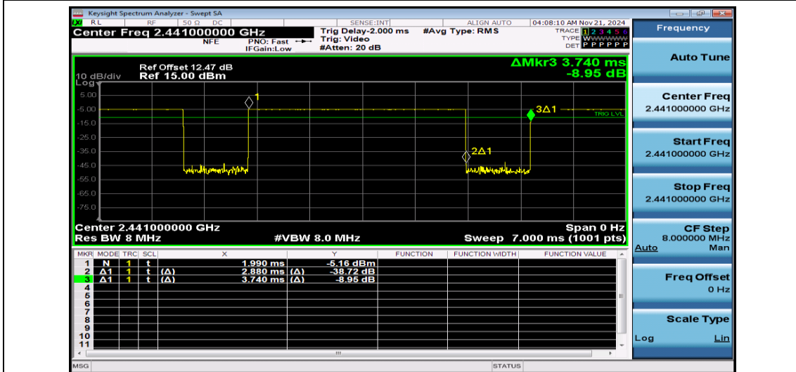
NTNV-DH5-Ant1-2441
