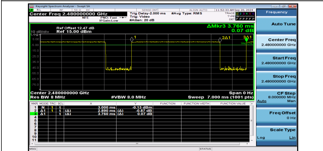
NTNV-3DH5-Ant1-2480
