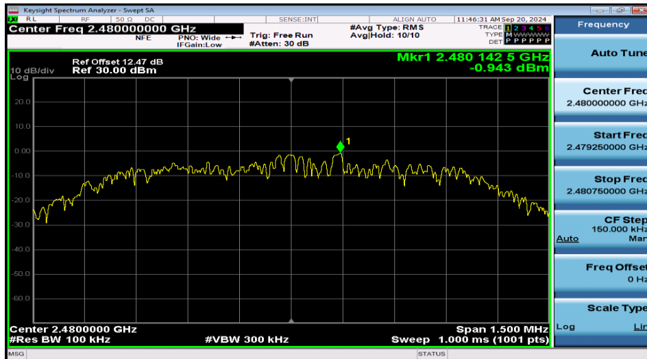
2DH5-Ant1-2480-0~Reference-PASS
