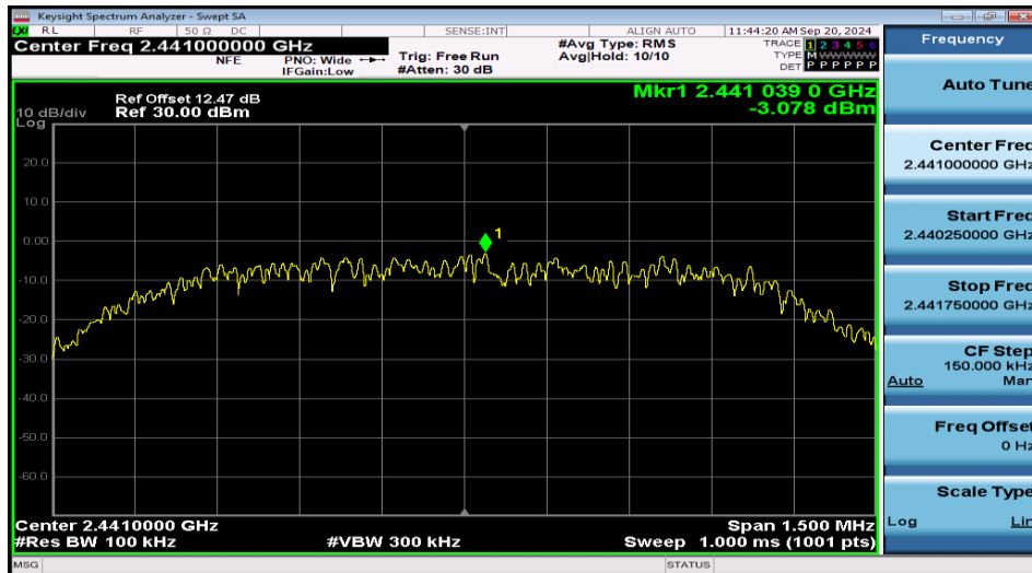
2DH5-Ant1-2441-0~Reference-PASS
