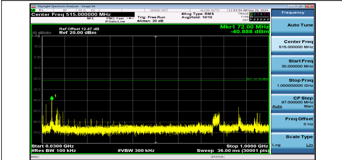
3DH5-Ant1-2480-30~1000-PASS
