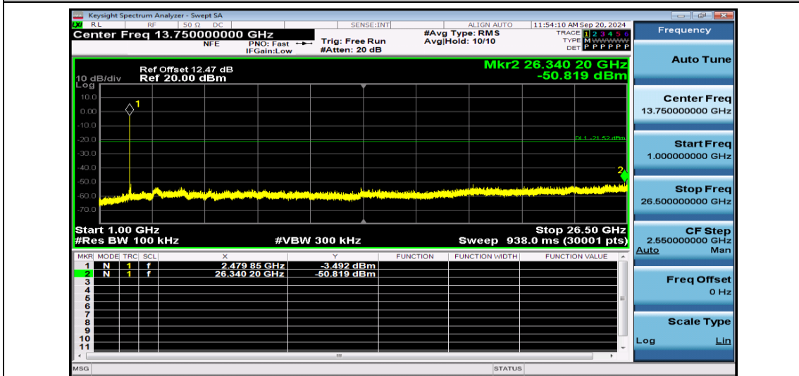
3DH5-Ant1-2480-1000~26500-PASS
