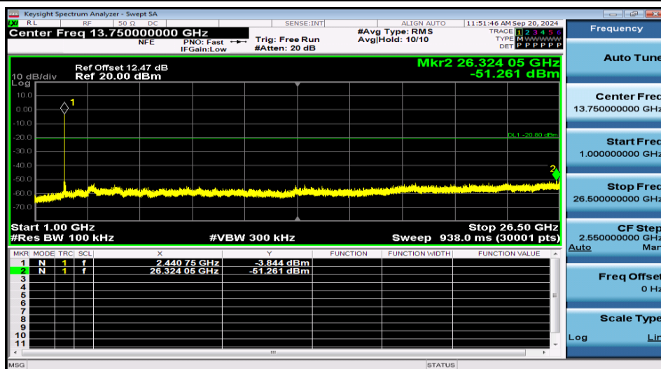
3DH5-Ant1-2441-1000~26500-PASS
