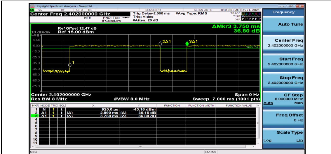
NTNV-3DH5-Ant1-2402
