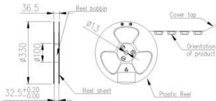
Figure 37: Reel Dimensions
