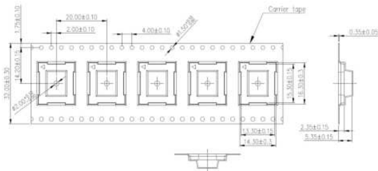
Figure 36: Tape Dimensions
