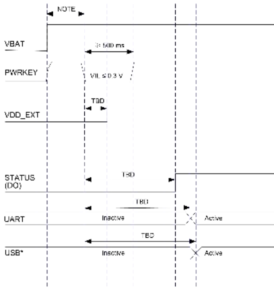
Figure 7: Power-up Timing
