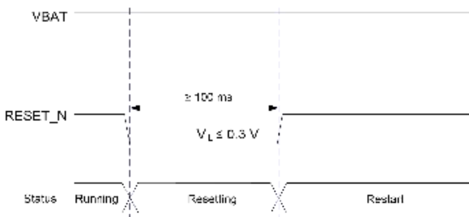
Figure 9: Reset Timing
