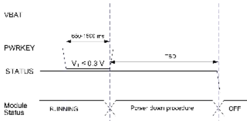
Figure 8: Power-down Timing
