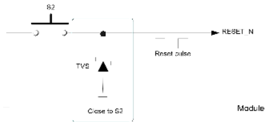
Figure 11: Reference Circuit of RESET_N by Using Button
