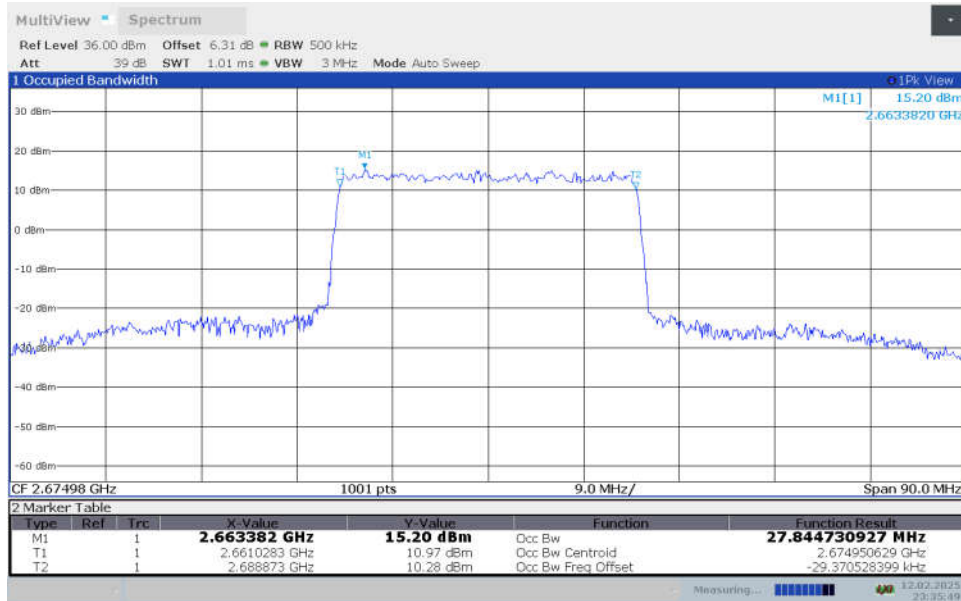
n41,30MHz Bandwidth,CP-64QAM (99% OBW)
