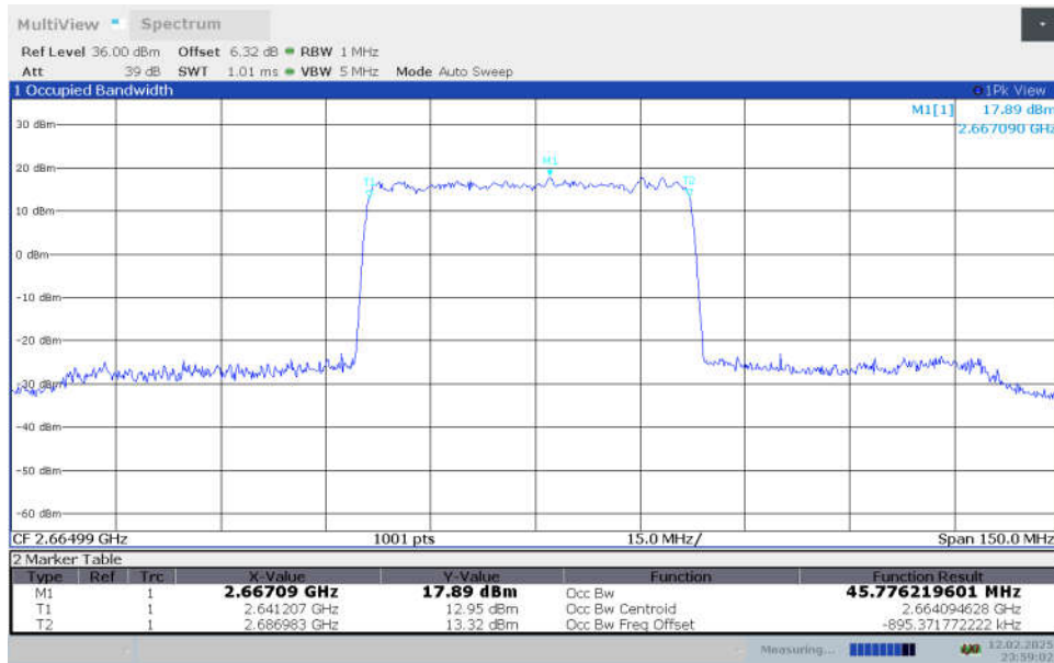
n41,50MHz Bandwidth,DFT-s-64QAM (99% OBW)
