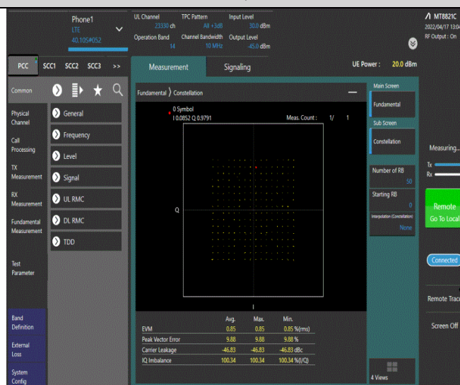
Band14-10MHz-256QAM-23330-50RB#0
