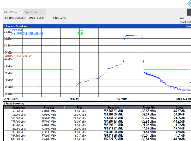
Band14-5MHz-QPSK-23305-25RB#0
