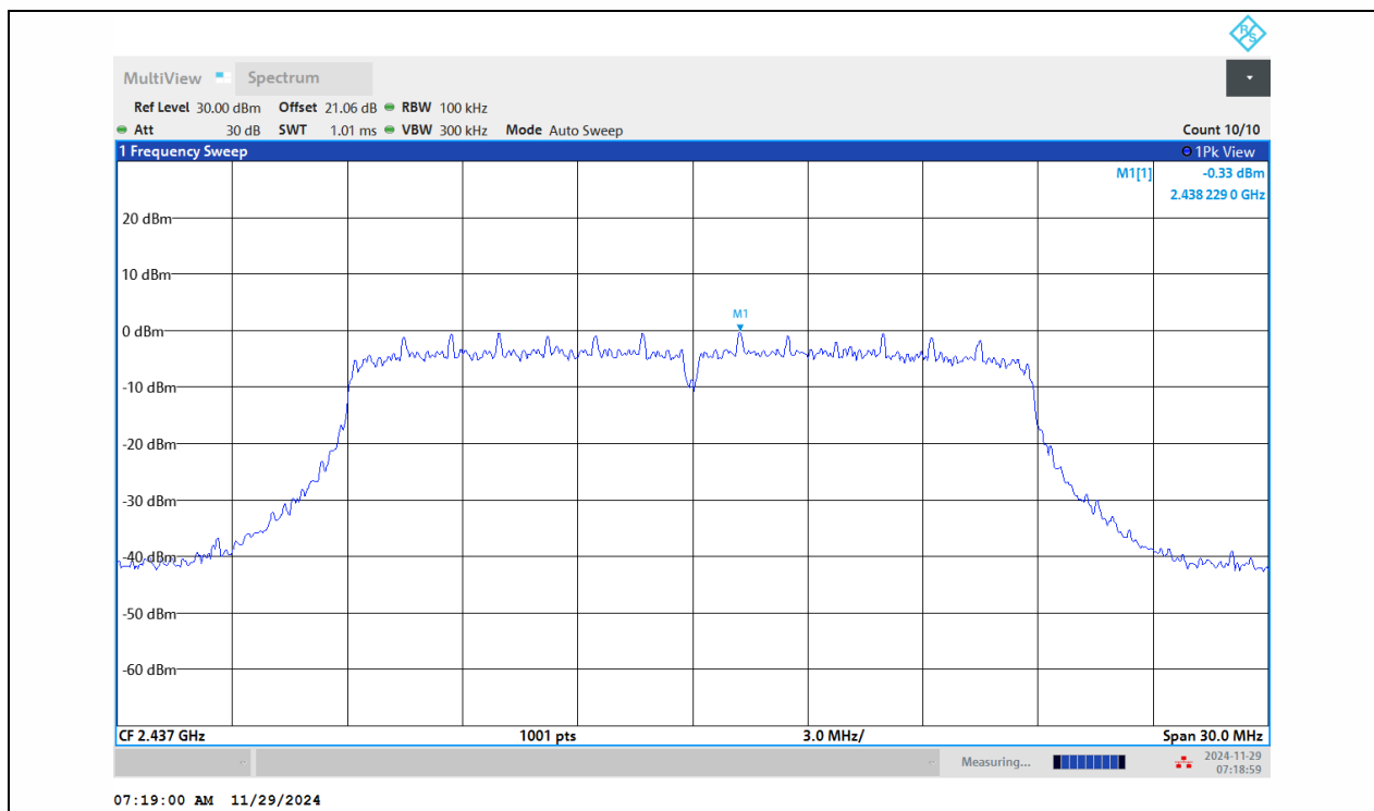
11N20MIMO-Ant1-2437-0-Reference-PASS
