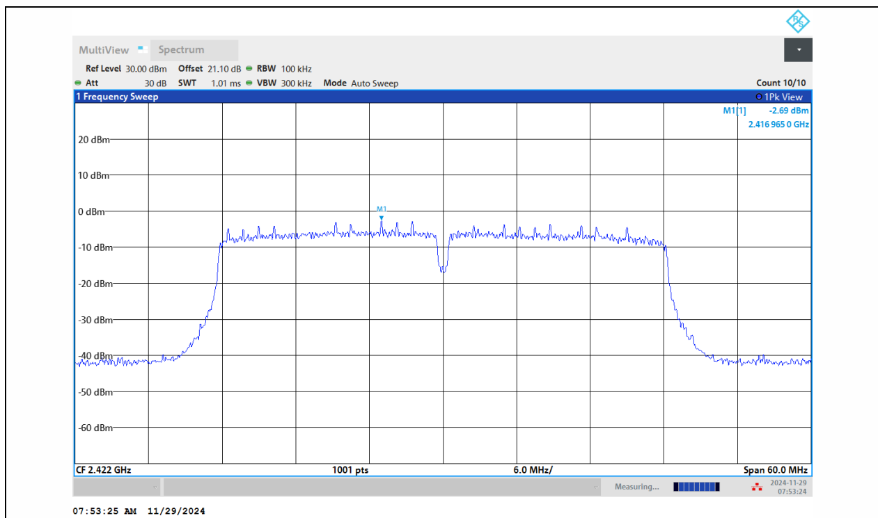
11N40MIMO-Ant1-2422-0-Reference-PASS
