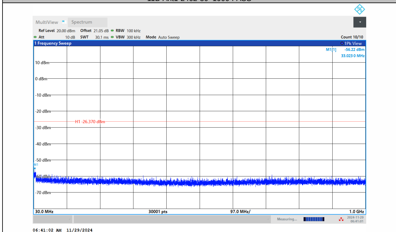
11B-Ant2-2462-30~1000-PASS
