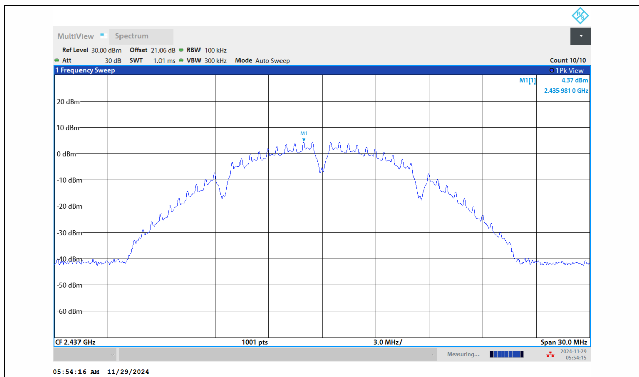
11B-Ant1-2437-0-Reference-PASS
