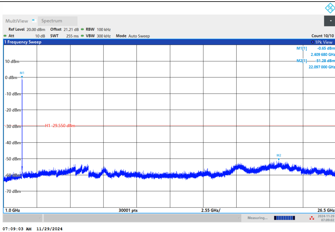
11N20MIMO-Ant1-2412-1000~26500-PASS
