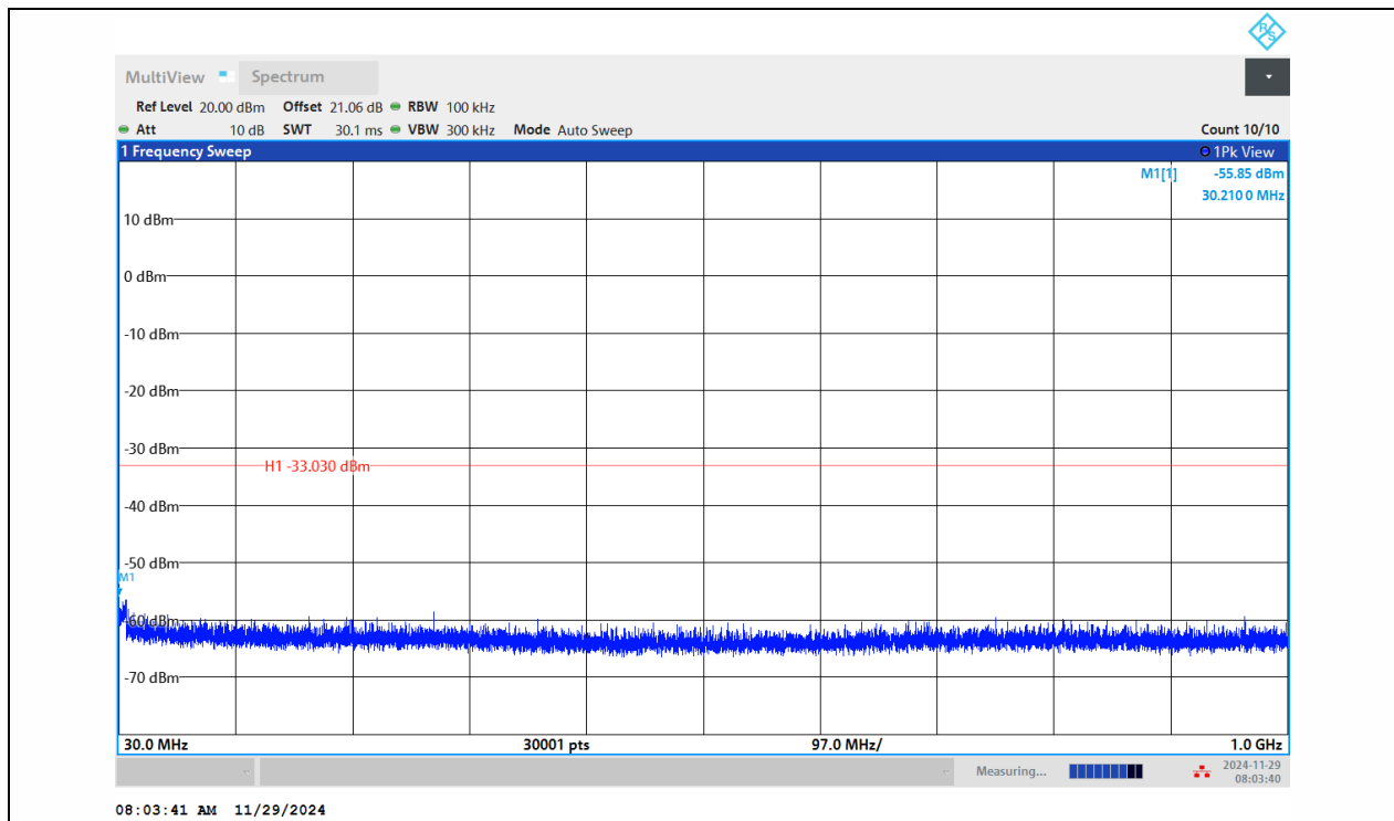
11N40MIMO-Ant1-2437-30~1000-PASS
