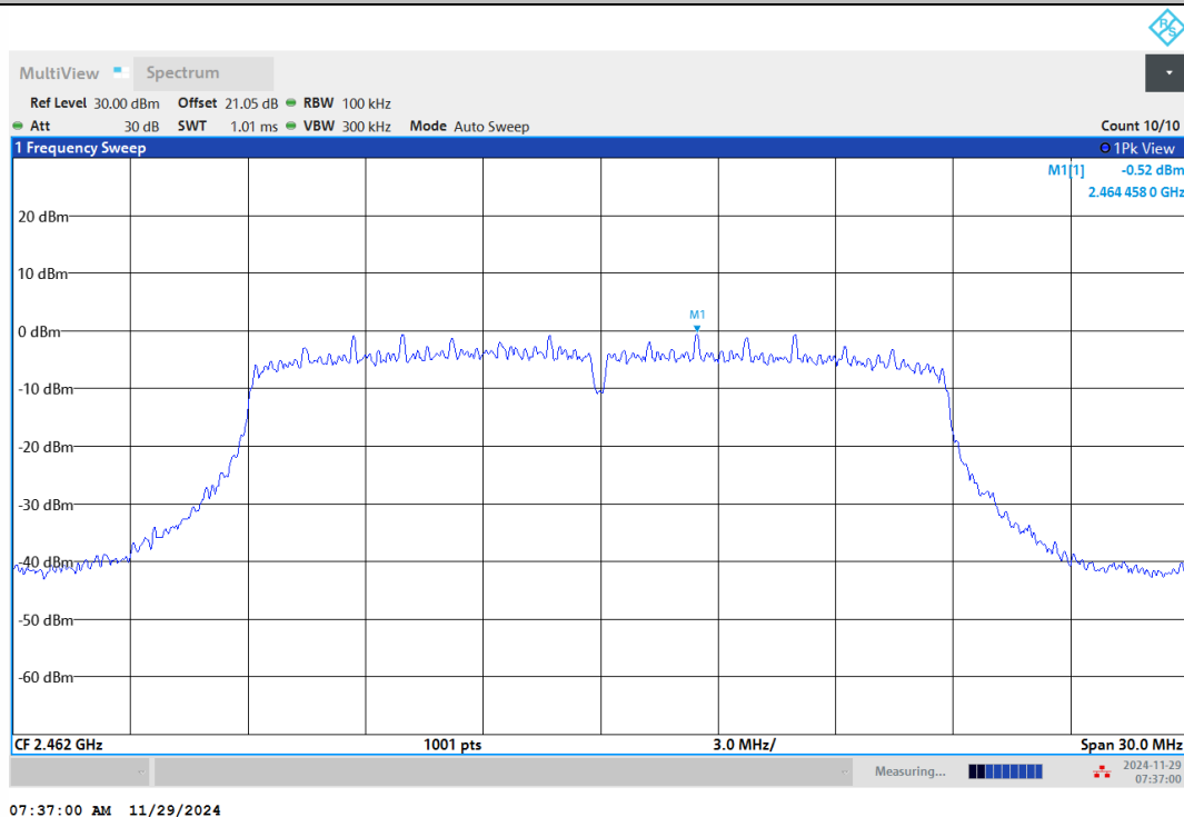
11N20MIMO-Ant2-2462-0-Reference-PASS
