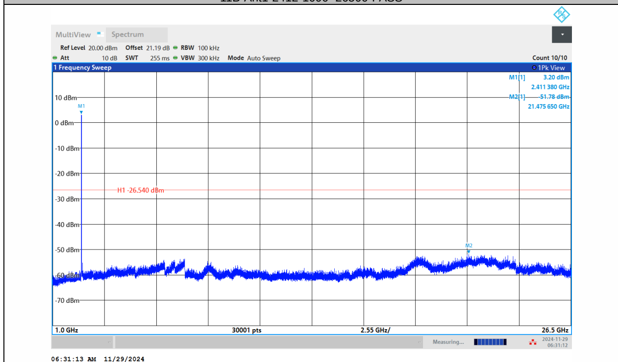
11B-Ant2-2412-1000~26500-PASS
