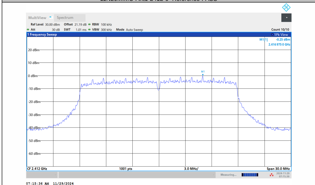
11N20MIMO-Ant2-2412-0-Reference-PASS
