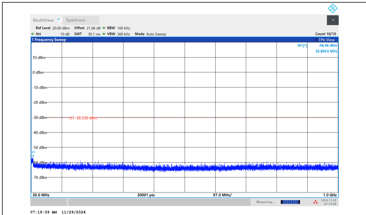
11N20MIMO-Ant1-2437-30~1000-PASS
