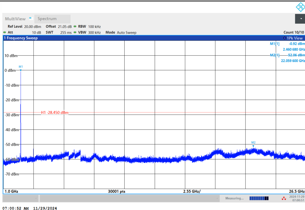
11G-Ant2-2462-1000~26500-PASS
