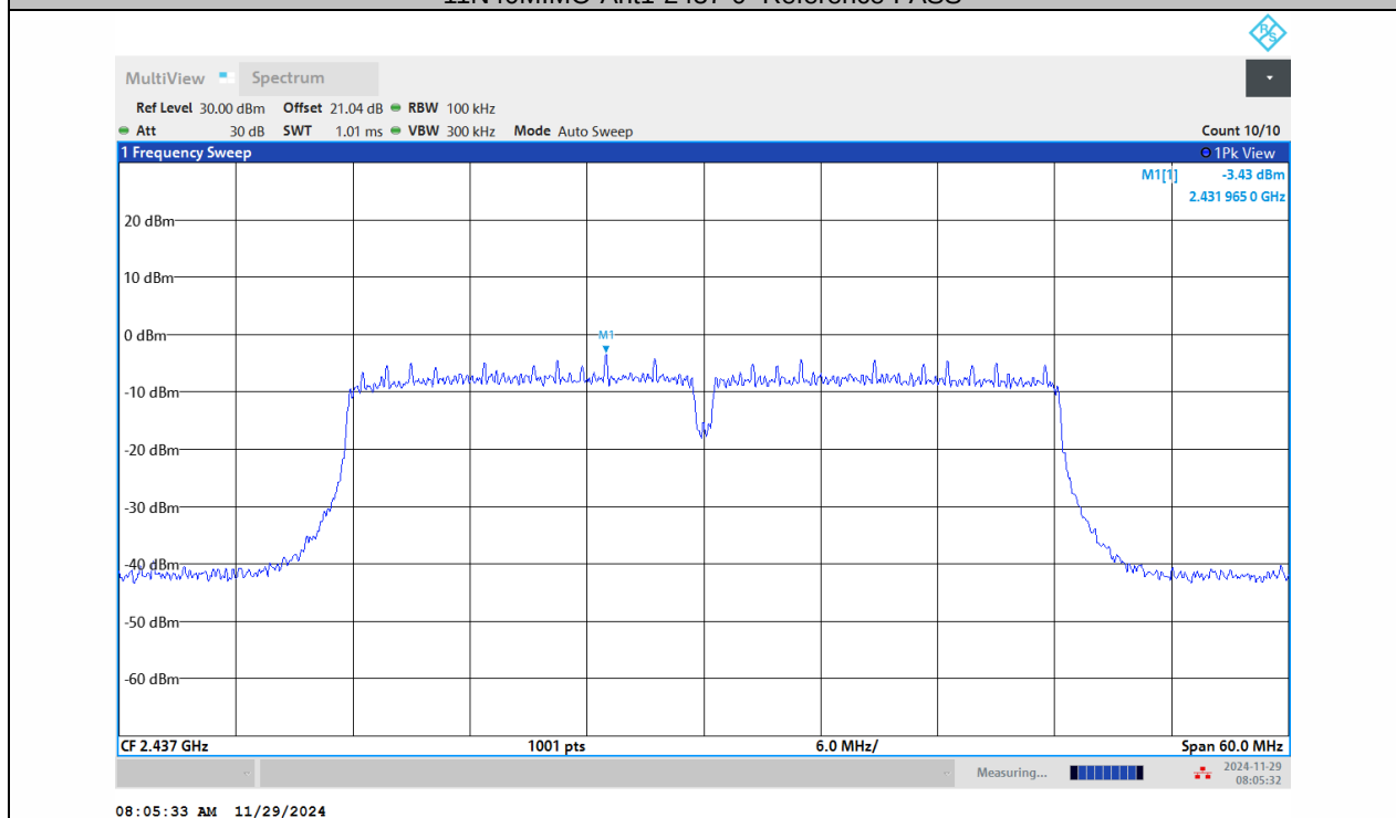
11N40MIMO-Ant2-2437-0-Reference-PASS
