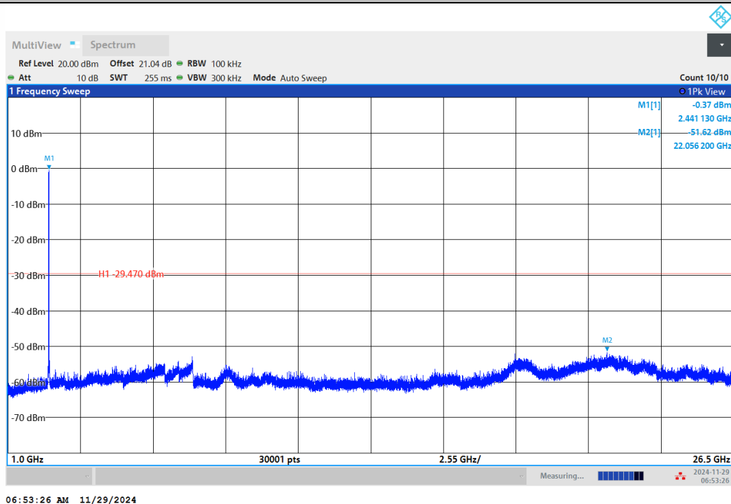
11G-Ant2-2437-1000~26500-PASS
