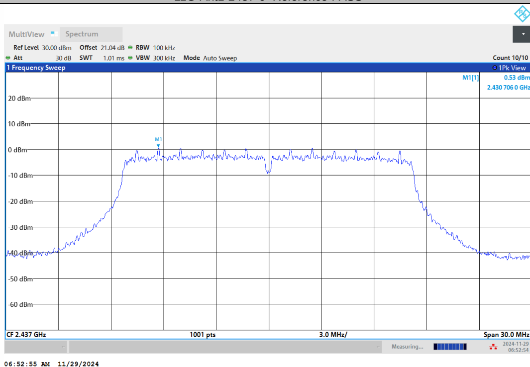
11G-Ant2-2437-0~Reference-PASS
