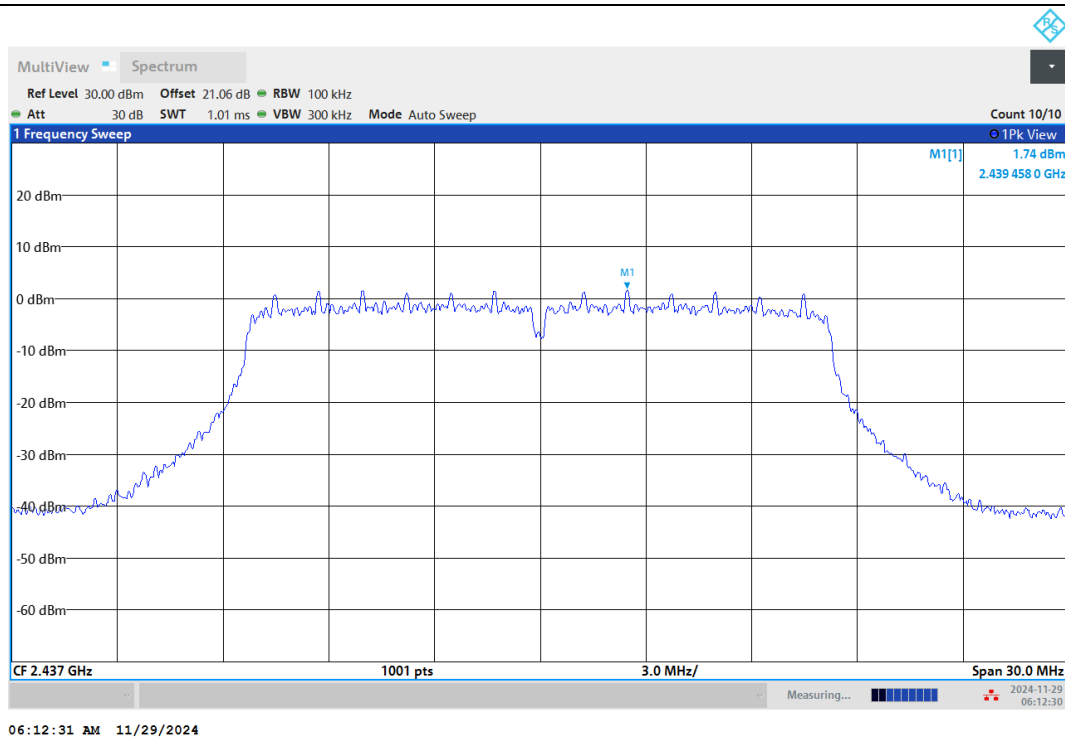
11G-Ant1-2437-0~Reference-PASS
