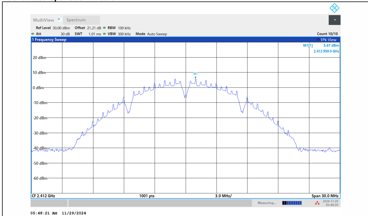
11B-Ant1-2412-0-Reference-PASS
