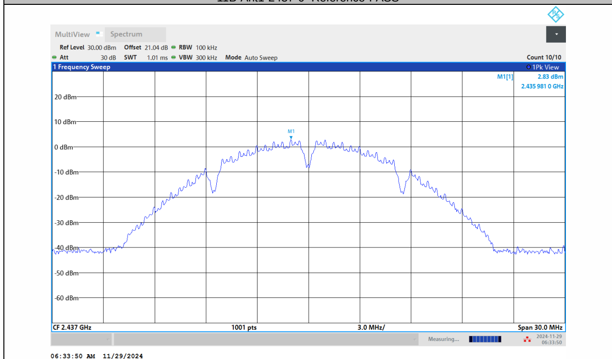
11B-Ant2-2437-0-Reference-PASS
