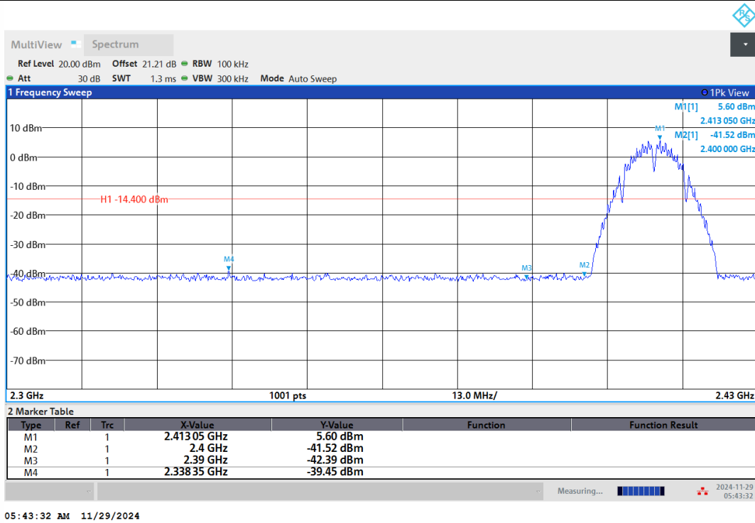
11B-Ant1-2412-PASS
