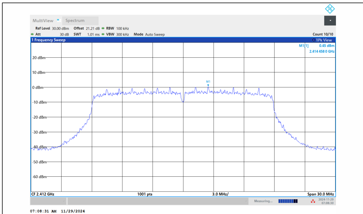
11N20MIMO-Ant1-2412-0-Reference-PASS
