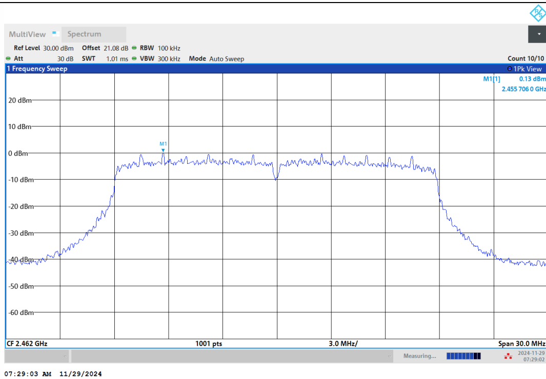
11N20MIMO-Ant1-2462-0-Reference-PASS
