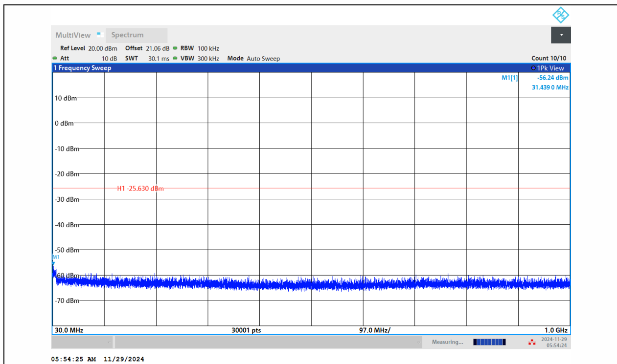
11B-Ant1-2437-30~1000-PASS
