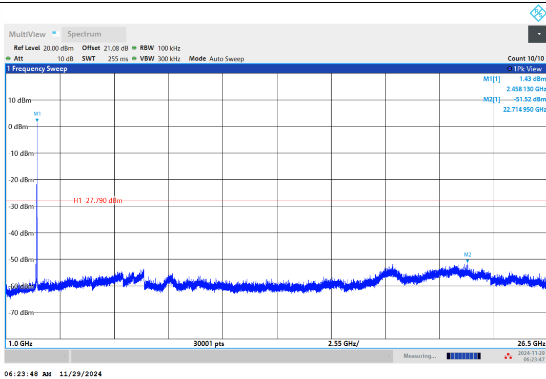
11G-Ant1-2462-1000~26500-PASS
