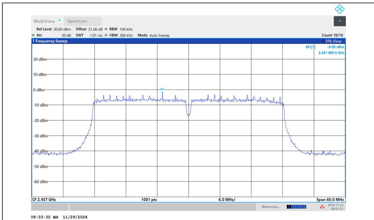
11N40MIMO-Ant1-2437-0-Reference-PASS
