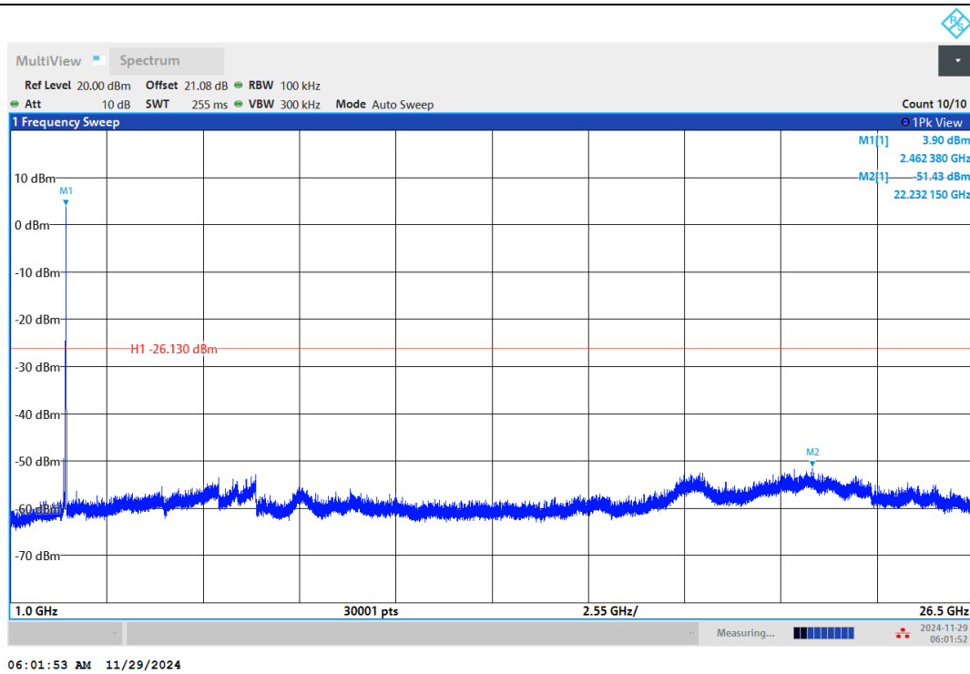
11B-Ant1-2462-1000~26500-PASS
