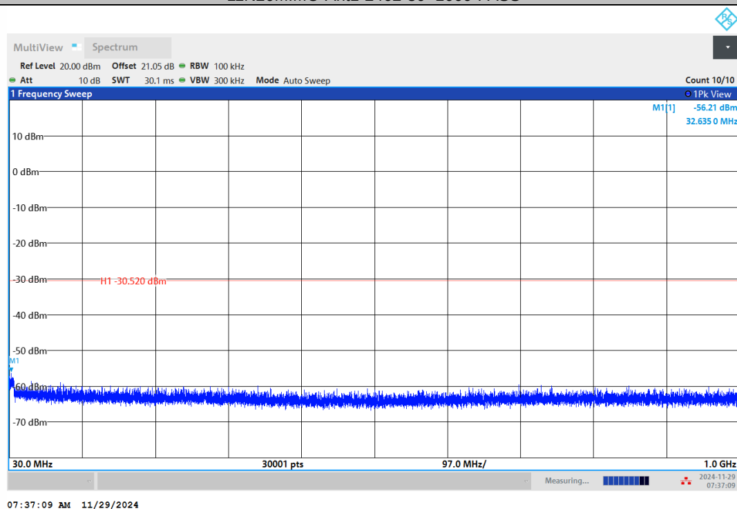
11N20MIMO-Ant2-2462-30~1000-PASS
