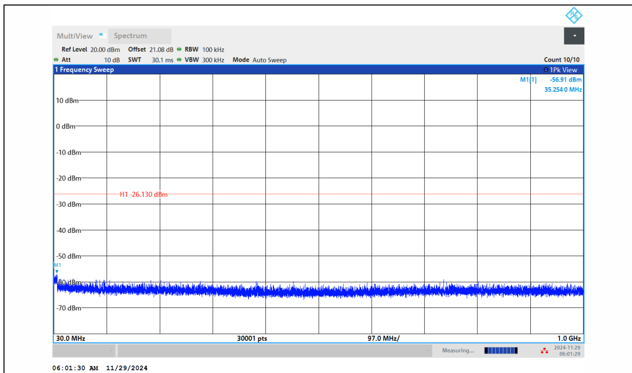
11B-Ant1-2462-30~1000-PASS
