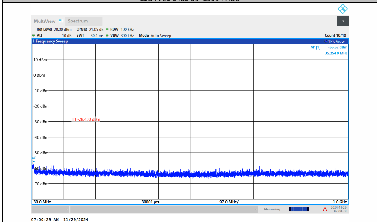
11G-Ant2-2462-30~1000-PASS
