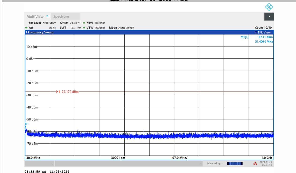
11B-Ant2-2437-30~1000-PASS
