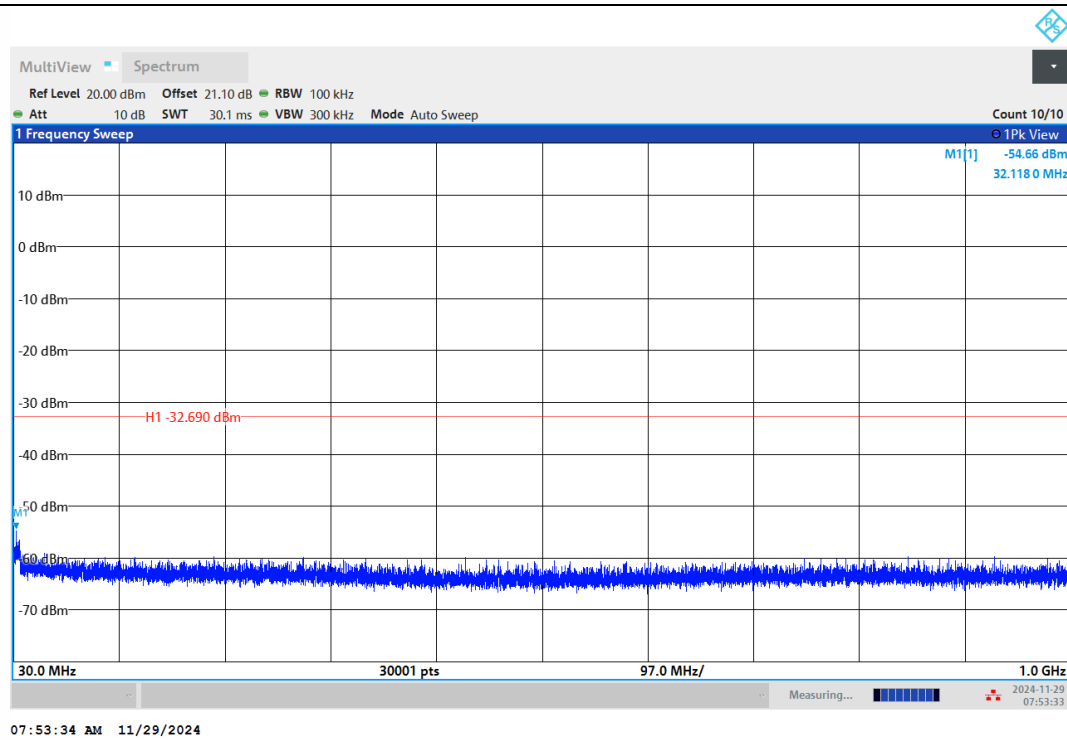
11N40MIMO-Ant1-2422-30~1000-PASS
