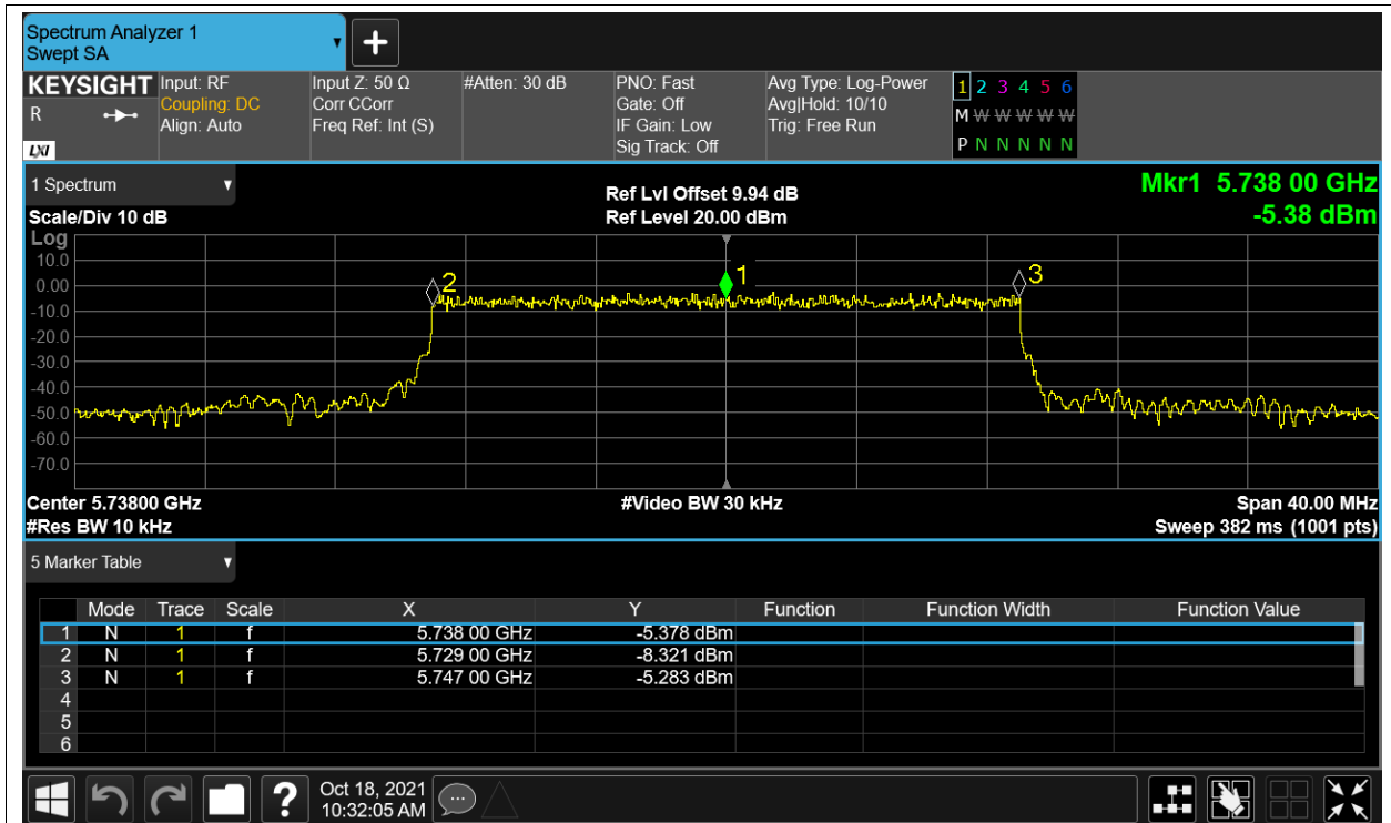
Freq. Stability LVLTLT 5.8G-20M-16QAM 5738MHz Ant1
