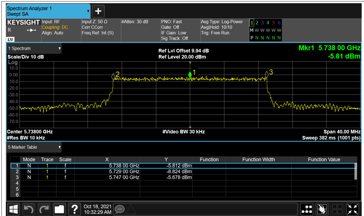
Freq. Stability HVLT 5.8G-20M-16QAM 5738MHz Ant1
