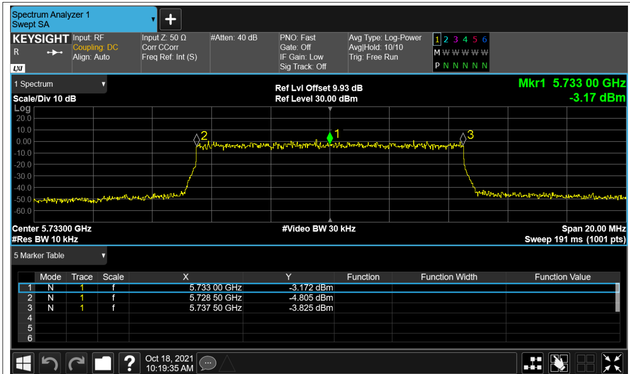
Freq. Stability HVL 5.8G-10M-16QAM 5733MHz Ant1
