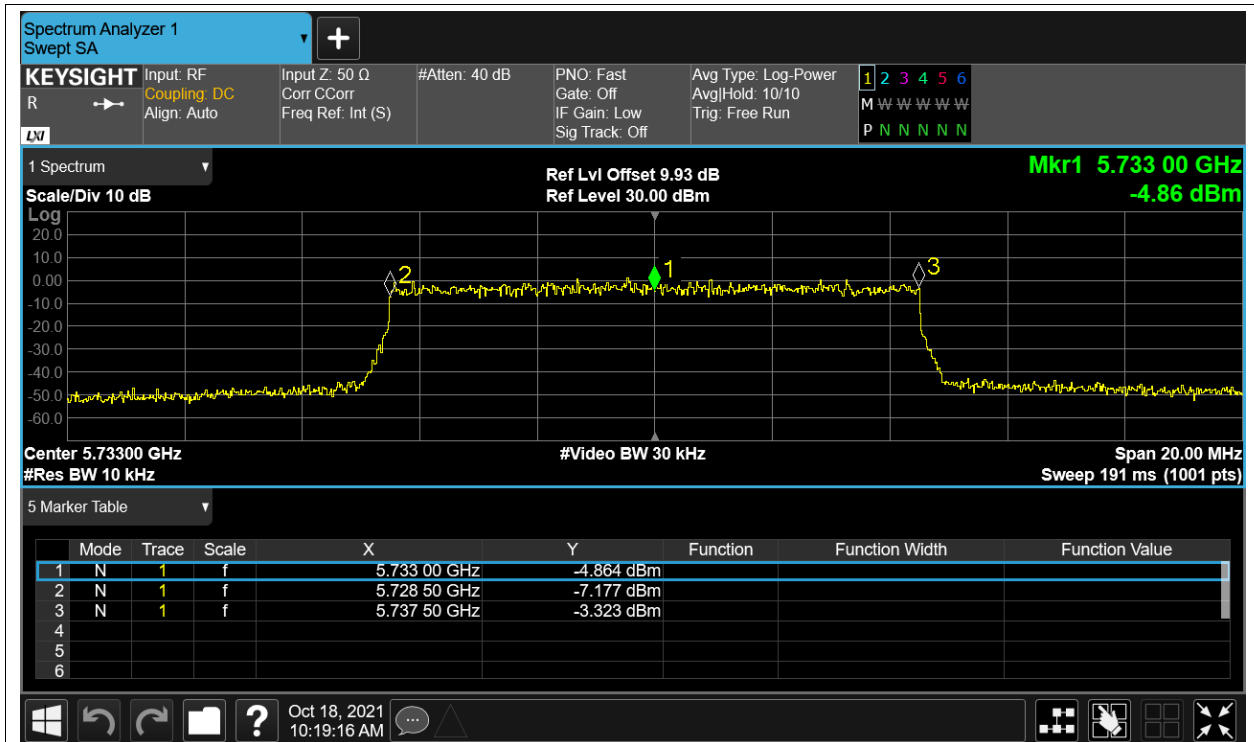
Freq. Stability LVLTLT 5.8G-10M-16QAM 5733MHz Ant1
