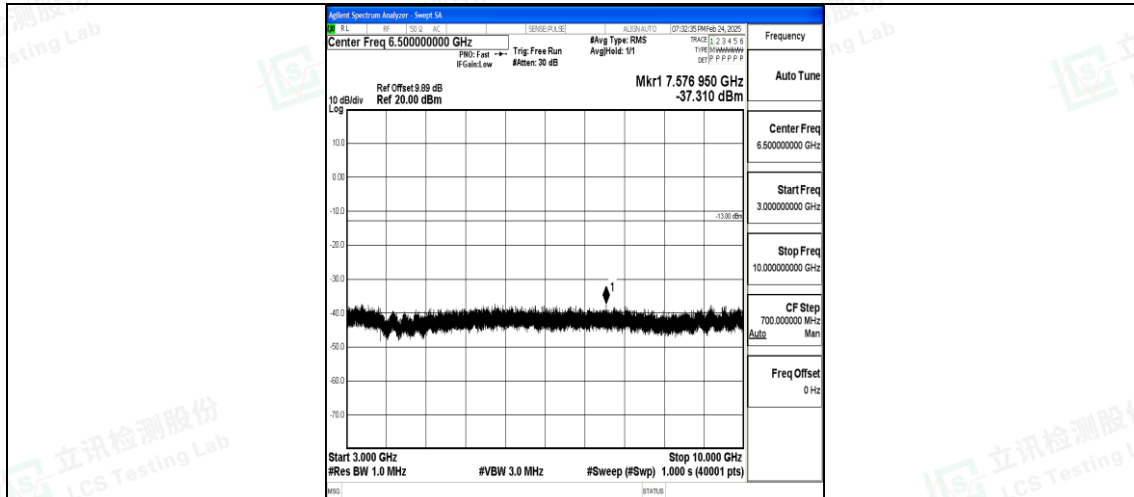
Band5_1.4MHz_QPSK_20525_1RB#0_3000~10000_3000~10000
