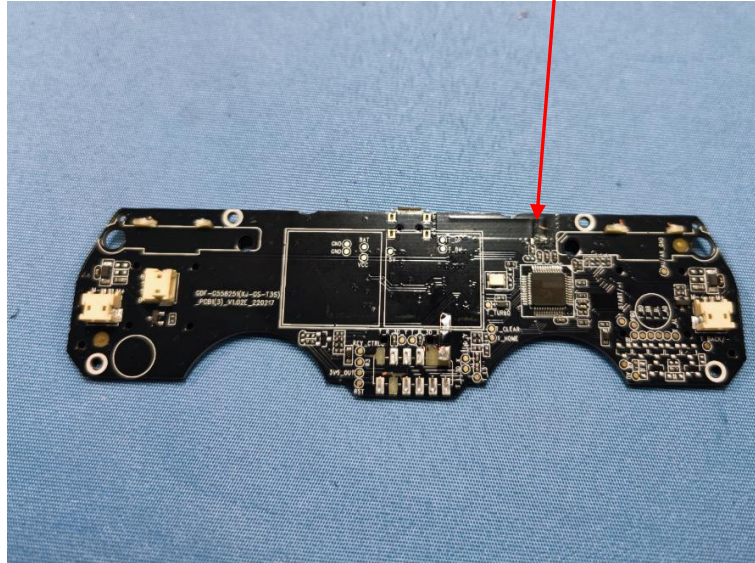
PCB Antenna
