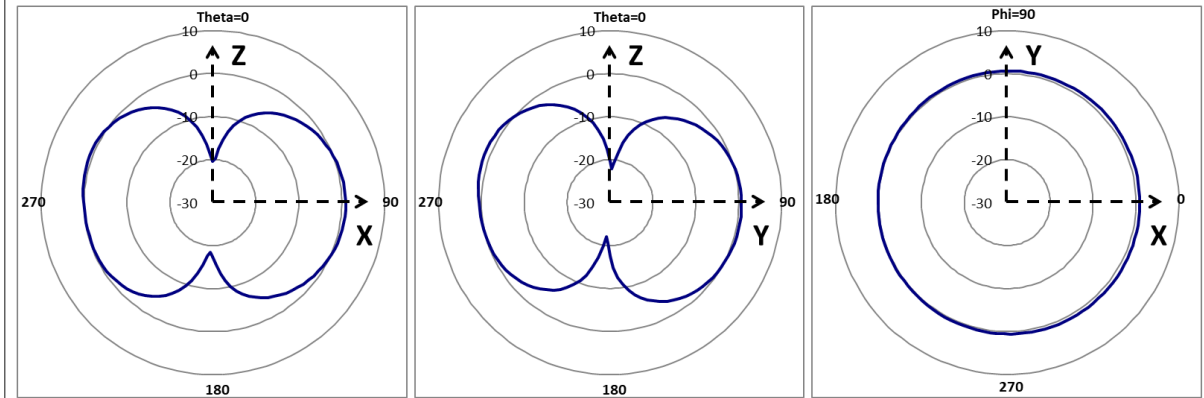
2G Radiation Pattern
