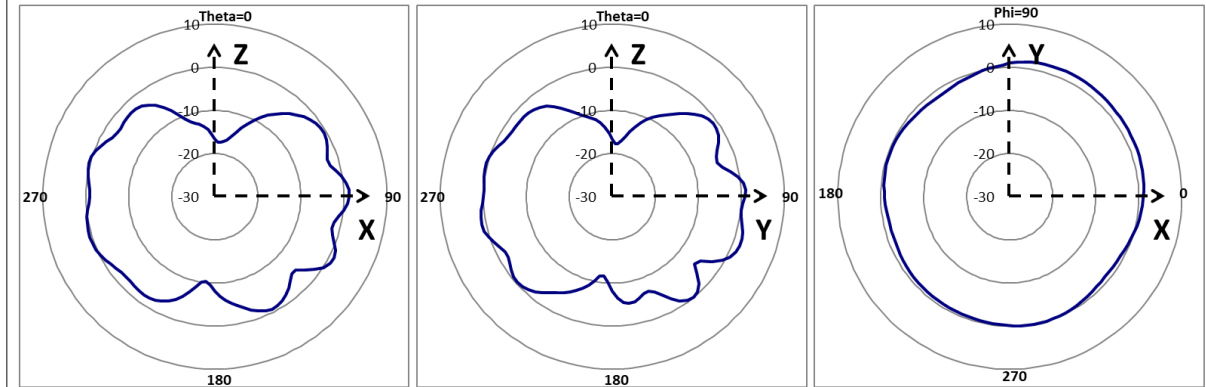
6G Radiation Pattern
