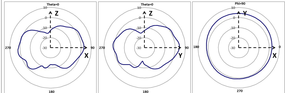
5G Radiation Pattern
