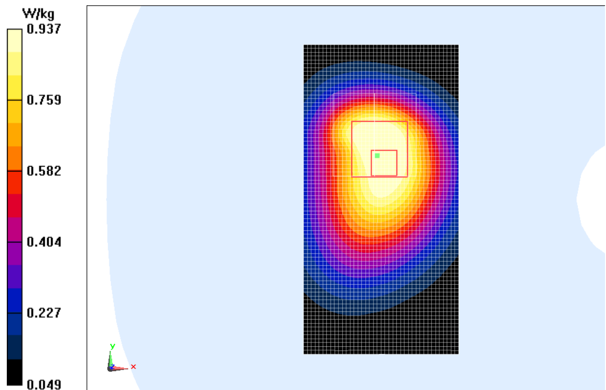
Fig.2 850 MHz CH128
