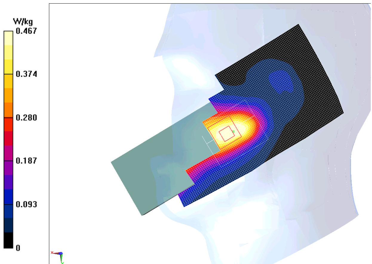
Fig.3 1900 MHz CH512
