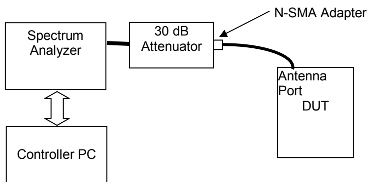
Figure E.6-1 - Setup Drawing
