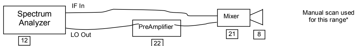
Figure H.6-2 - Setup Drawing ( \geq 26.5 GHz)
