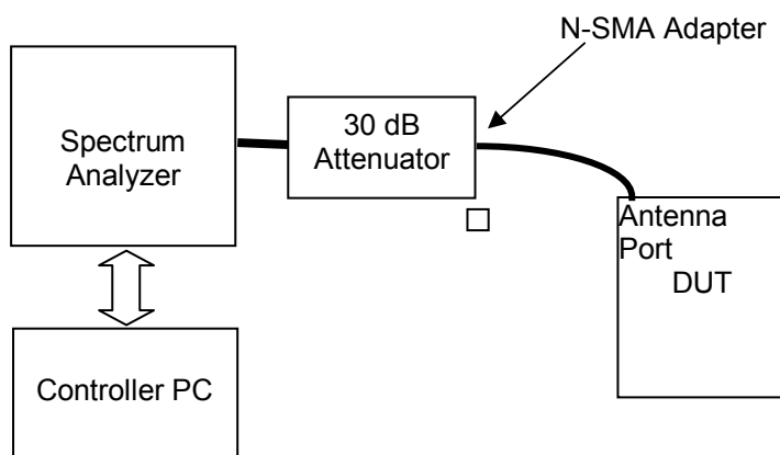
Figure I.6-1 - Setup Drawing
