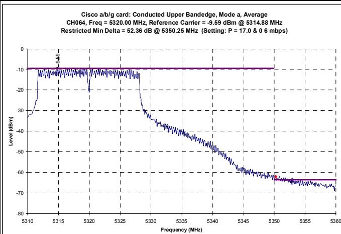
Channel 64 Mode a - Conducted Average Band-edge Plots
