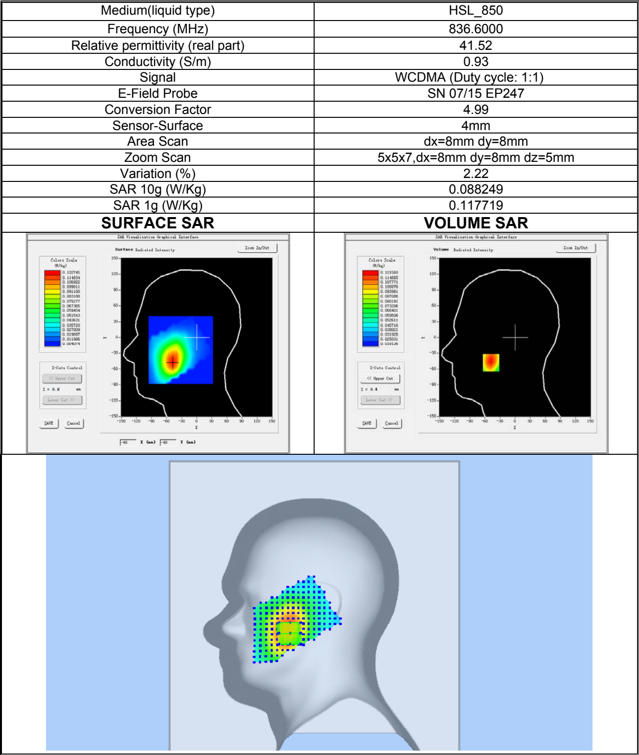
Plot 5: WCDMA BAND V, Mid channel (Right Head Cheek) Product Description: Mobile Computing Device Test Date: 2020-04-14
