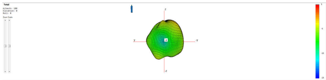
A7 (Frequency=5800MHz)
