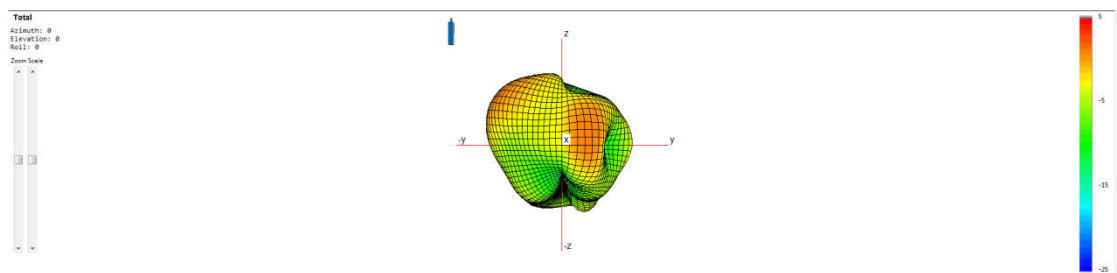
A7 (Frequency=6475MHz)
