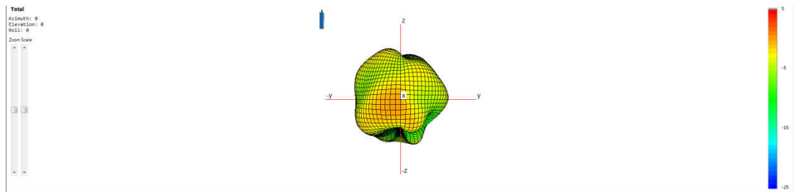
A7 (Frequency=5800MHz)
