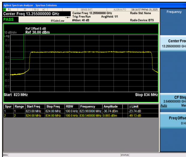
Band5_10MHz_QPSK_20450_50RB#0
