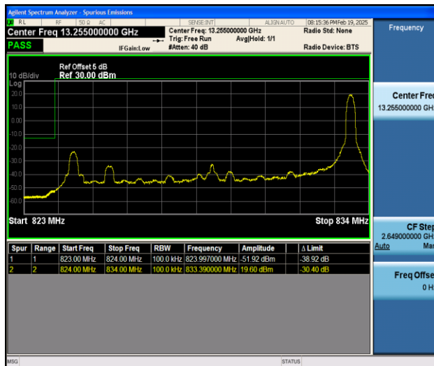
Band5_10MHz_QPSK_20450_1RB#49
