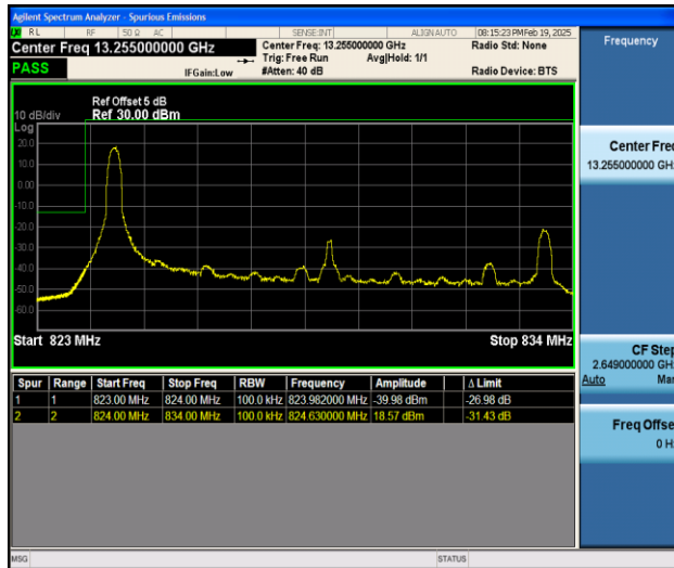
Band5_10MHz_16QAM_20450_1RB#0
