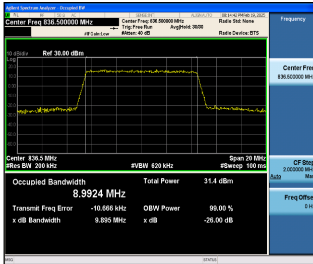
Band5-10MHz-QPSK-20525-50RB#0-PASS
