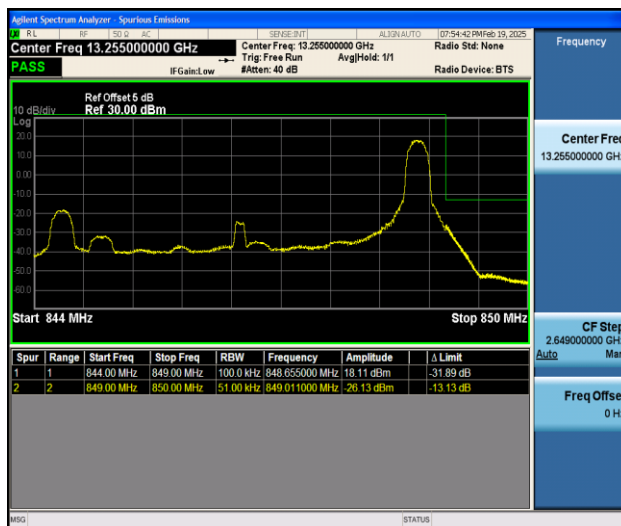
Band5_5MHz_QPSK_20625_1RB#24
