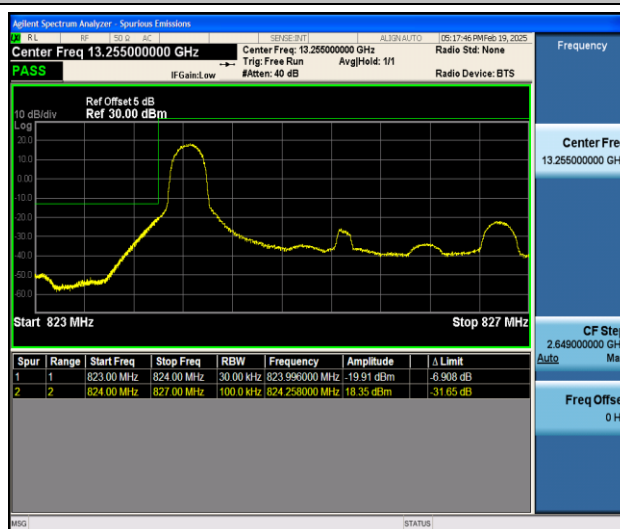
Band5_3MHz_16QAM_20415_1RB#0
