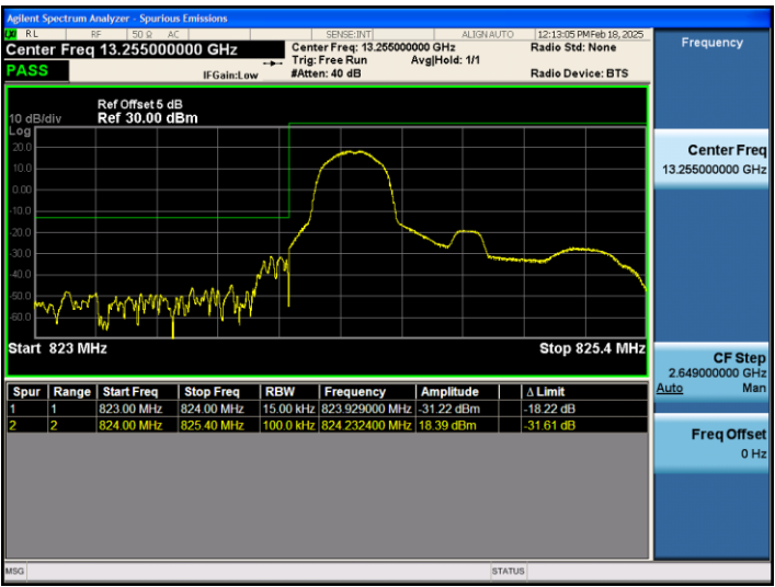
Band5_1.4MHz_QPSK_20407_1RB#0
