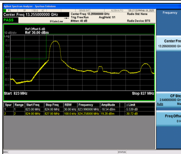
Band5_3MHz_QPSK_20415_1RB#0
