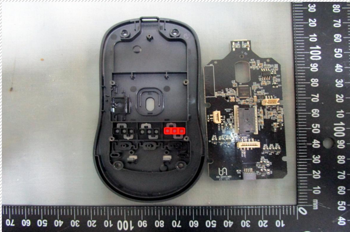
< PCB-F >
