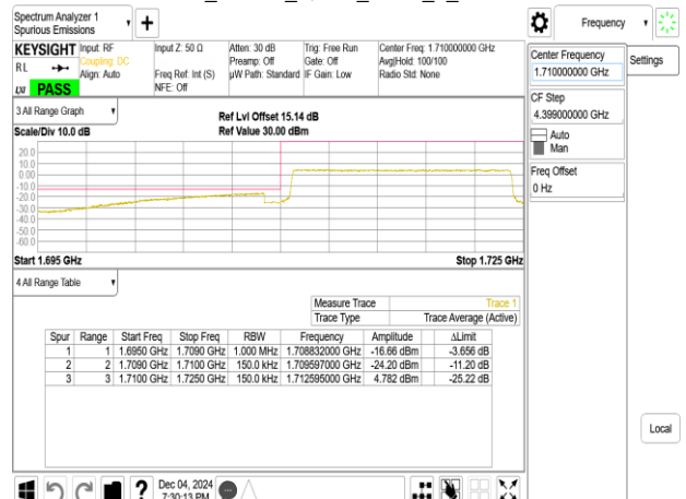
Band4_15MHz_QPSK_RB75_0_CH20025
