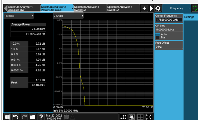
HSUPA CH 1513 (1752.6MHz)
