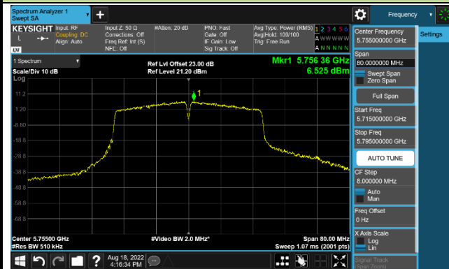
802.11ac-VHT80 Power Spectral Density - Ant 3
