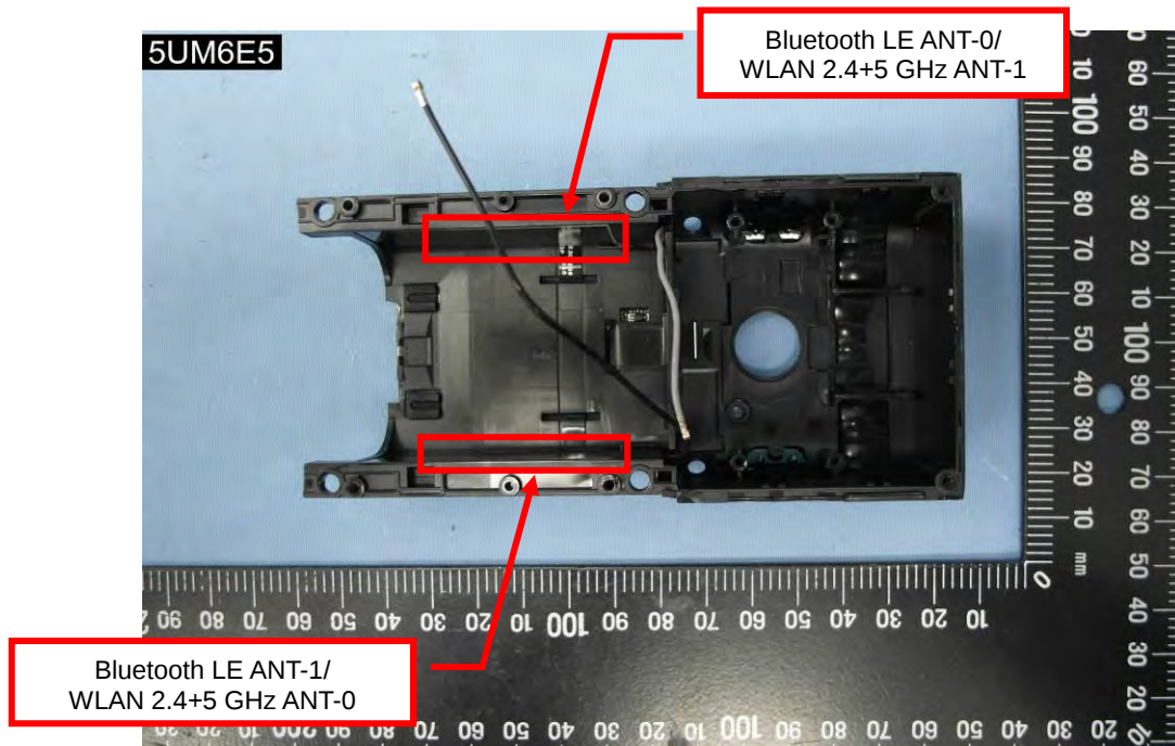
EUT Photo (34)
