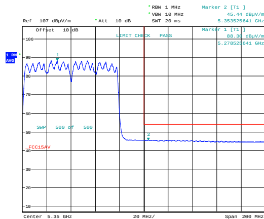
Band Edge, 5350 MHz, Ch058, 802.11ac MCS0 MIMO, Av, Max
