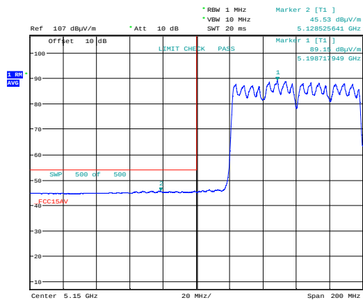
Band Edge, 5150 MHz, Ch042, 802.11ac MCS0 MIMO, Av, Max
