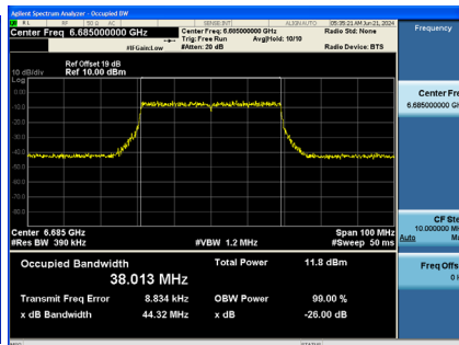
CH147 26 dB Bandwidth
