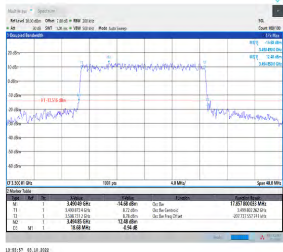
1-N78-3450-3550--30-20-M-3-DFT-16QAM-Outer_Fu II-50@0-Ant1-17.858-18.680-≤20-PASS
