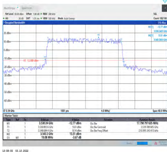
1-N78-3450-3550--30-20-H-1-DFT-QPSK-Outer_Full -50@0-Ant1-17.791-19.080-<20-PASS
