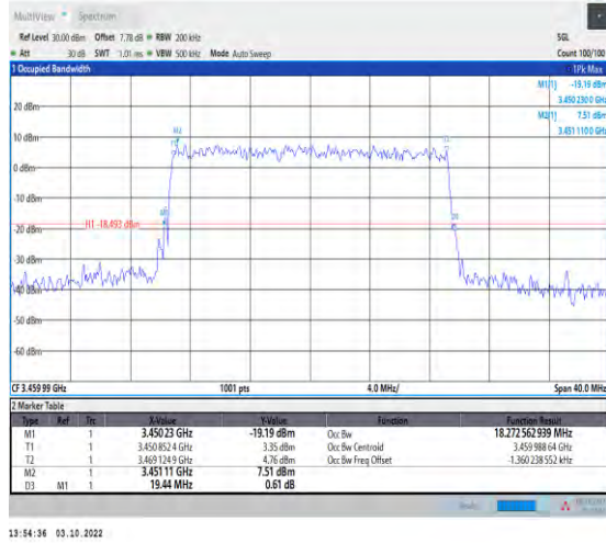
1-N78-3450-3550--30-20-L-9-CP-256QAM-Outer_Fu II-51@0-Ant1-18.273-19.440-≤20-PASS
