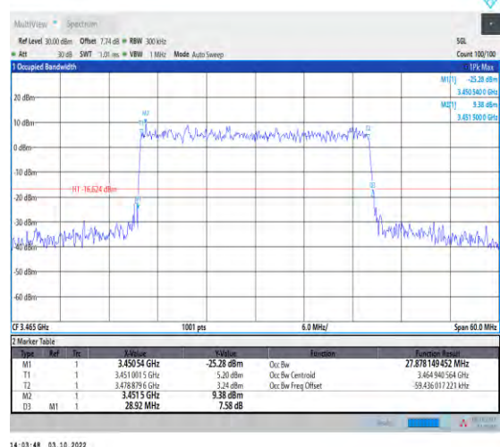
1-N78-3450-3550--30-30-L-9-CP-256QAM-Outer_Full-78@0-Ant1-27.878-28.920-≤30-PASS
