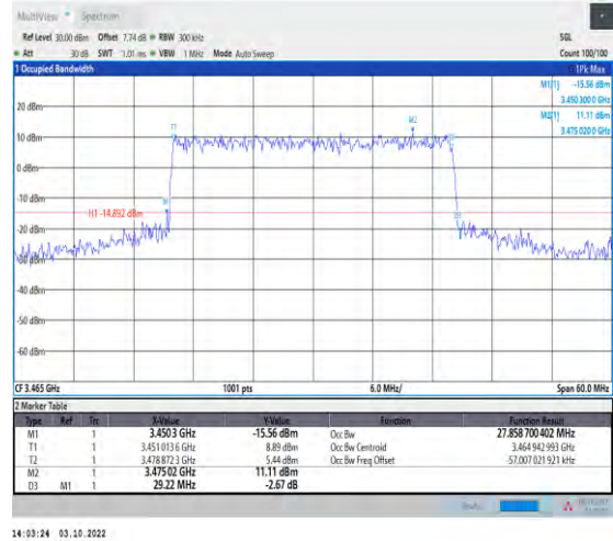
1-N78-3450-3550--30-30-L-7-CP-16QAM-Outer_Full-78@0-Ant1-27.859-29.220-≤30-PASS
