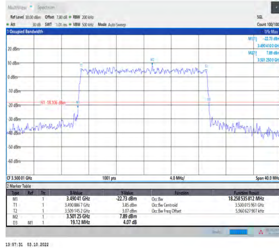
1-N78-3450-3550--30-20-M-9-CP-256QAM-Outer_F ull-51@0-Ant1-18.259-19.120-<20-PASS
