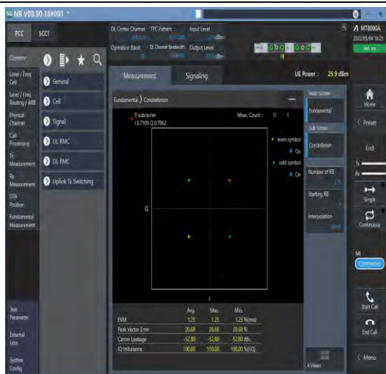
1-N78-3450-3550--30-100-M-1-DFT-PI2BPSK-Outer_Full-270@0-Ant1-see graph-PASS
