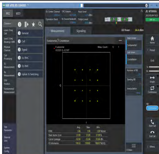
1-N78-3450-3550--30-100-M-3-DFT-16QAM-Outer_Full-270@0-Ant1-see graph-PASS
