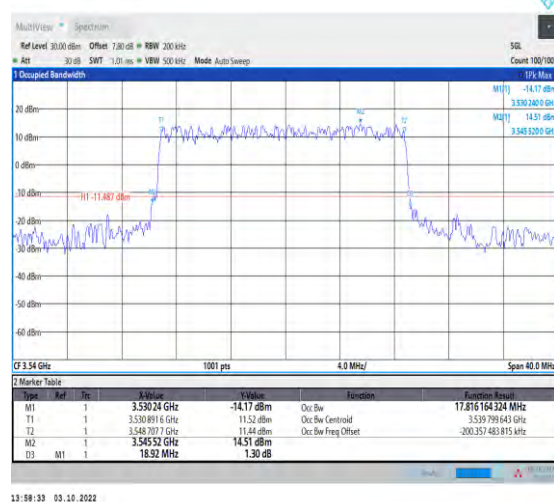
1-N78-3450-3550--30-20-H-2-DFT-PI2BPSK-Outer_ Full-50@0-Ant1-17.816-18.920-<20-PASS
