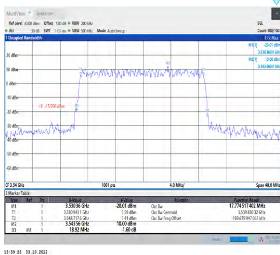
1-N78-3450-3550--30-20-H-5-DFT-256QAM-Outer_Full-50@0-Ant1-17.775-18.920-≤20-PASS
