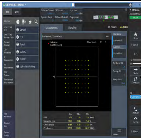
1-N78-3450-3550--30-100-M-4-DFT-64QAM-Outer_Full-270@0-Ant1-see graph-PASS
