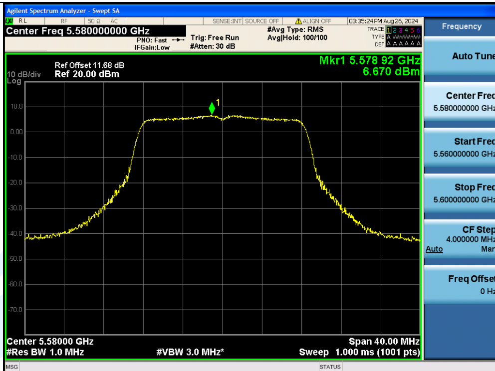
11A-Ant3-5580-PASS
