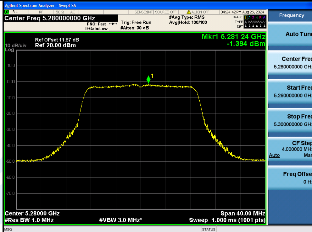
11AC20MIMO-Ant3-5280-PASS
