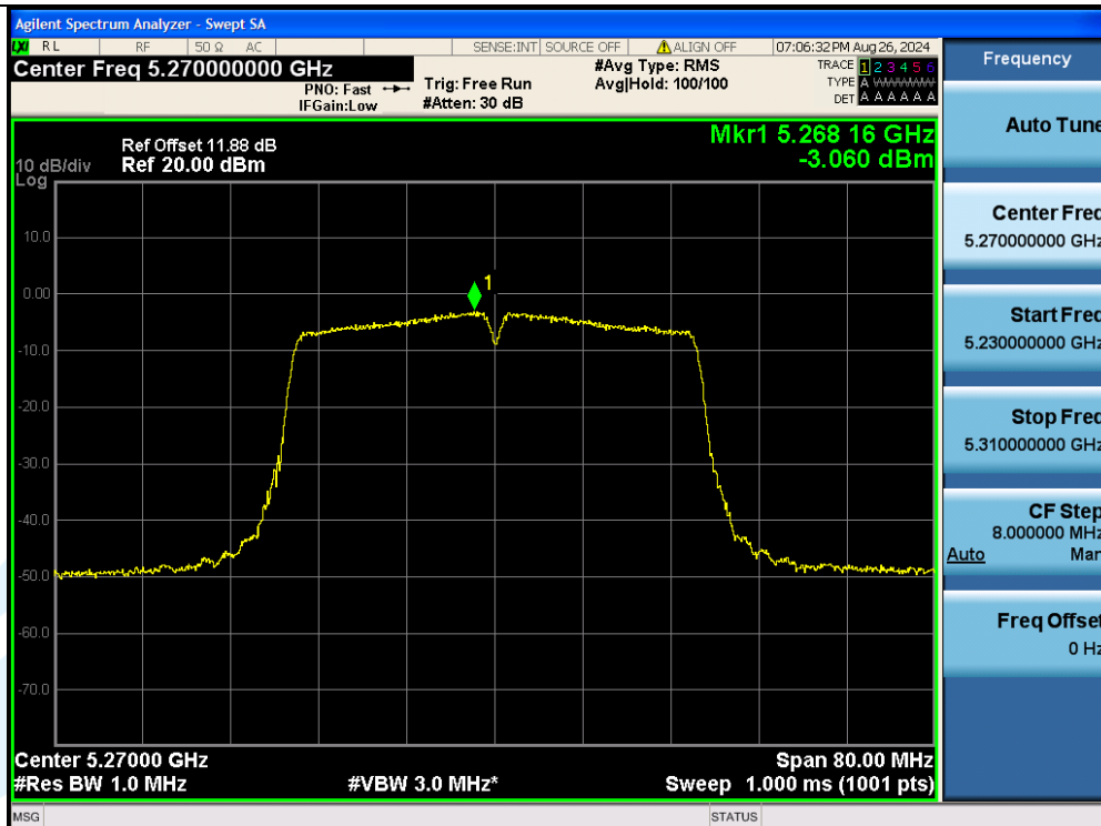
11N40MIMO-Ant2-5270-PASS
