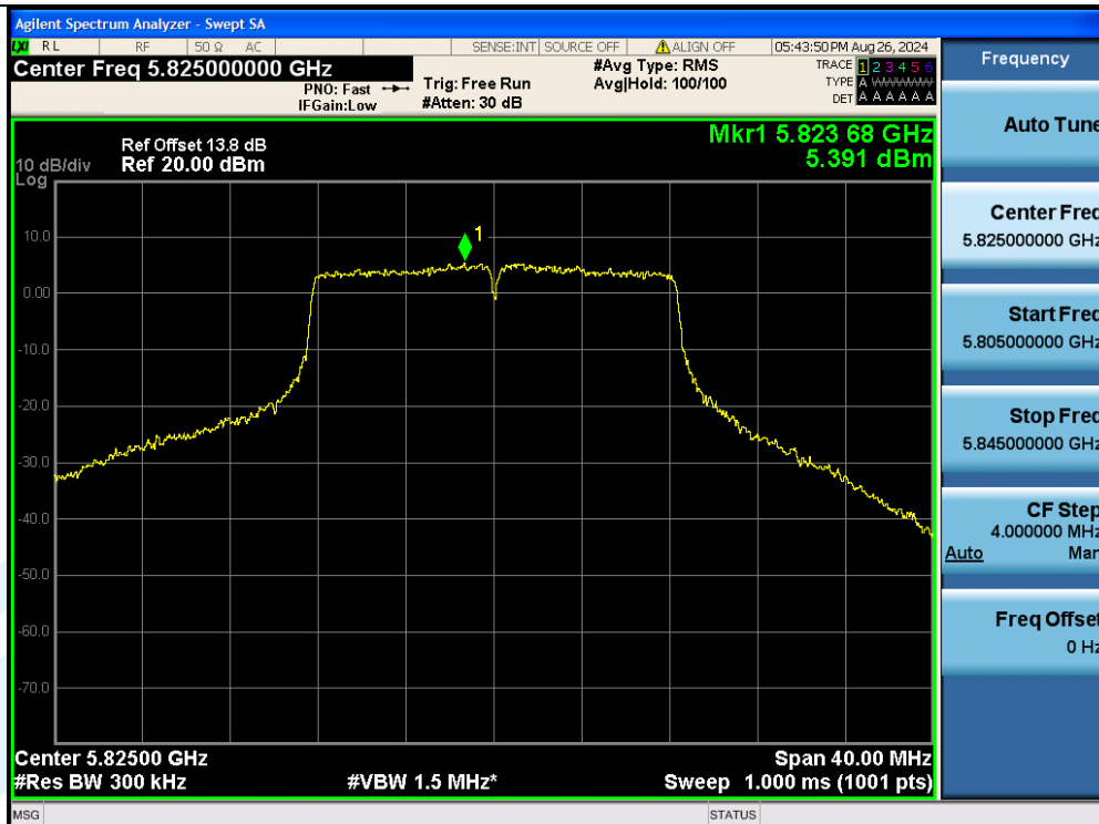
11A-Ant2-5825-PASS
