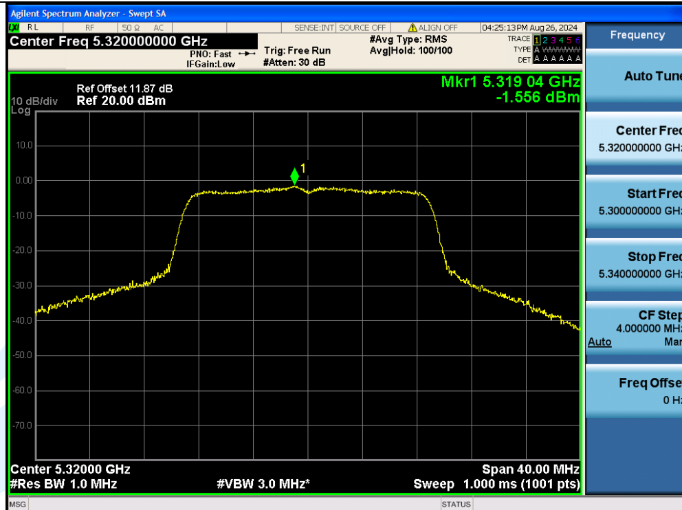
11AC20MIMO-Ant3-5320-PASS
