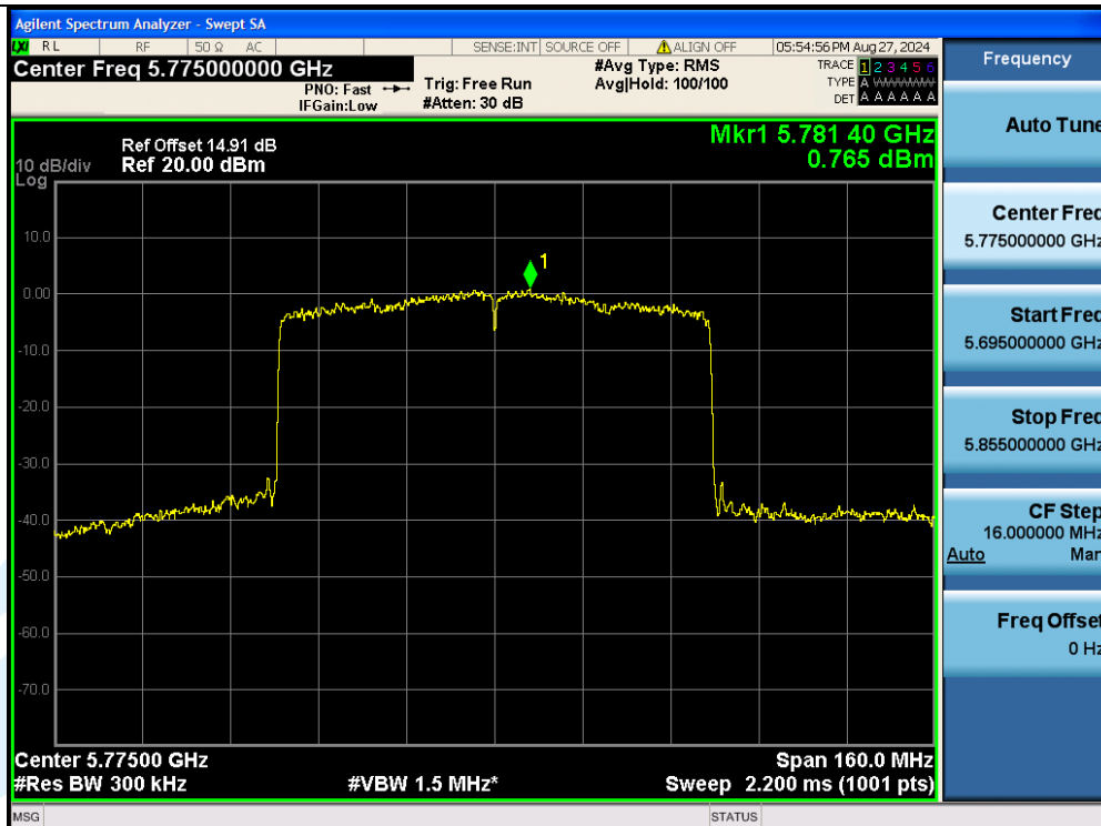
11AX80MIMO-Ant3-5775-PASS
