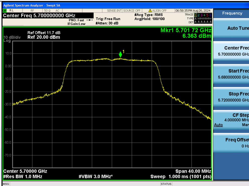
11N20MIMO-Ant2-5700-PASS
