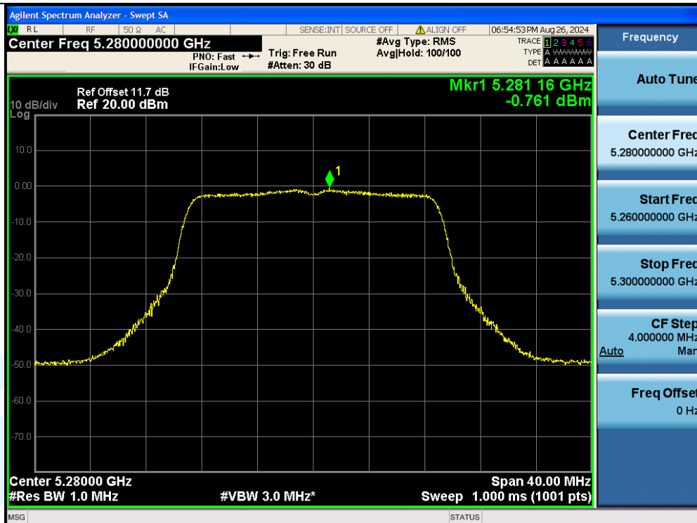
11N20MIMO-Ant2-5280-PASS
