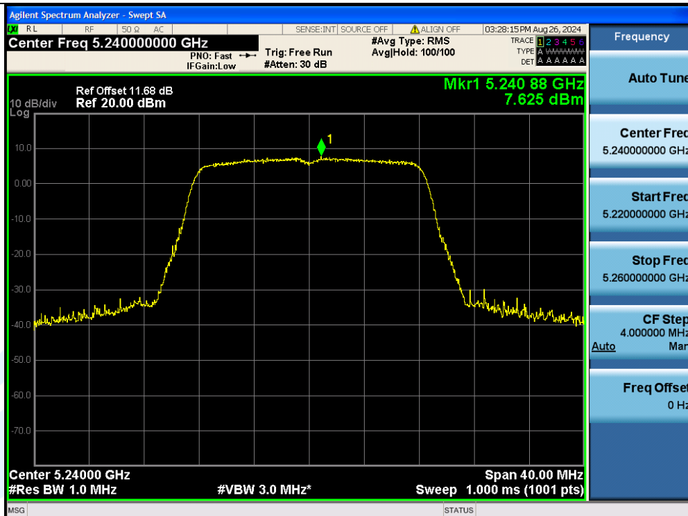
11A-Ant3-5240-PASS
