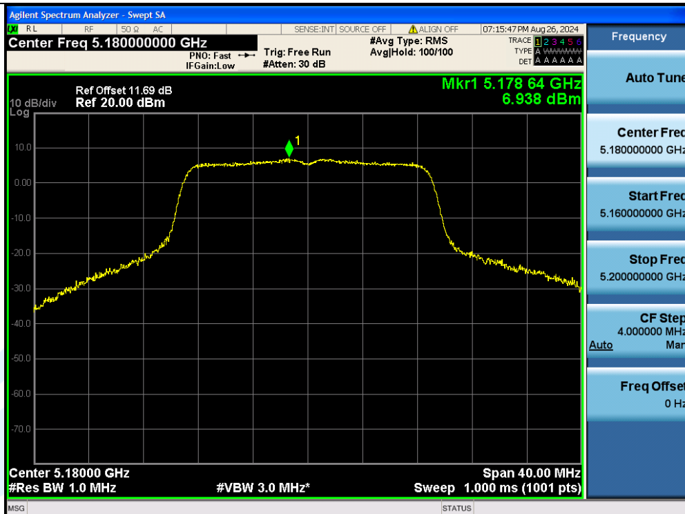
11AC20MIMO-Ant2-5180-PASS
