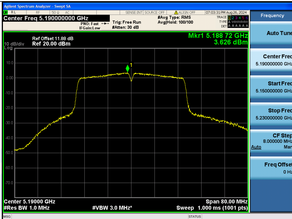
11N40MIMO-Ant2-5190-PASS
