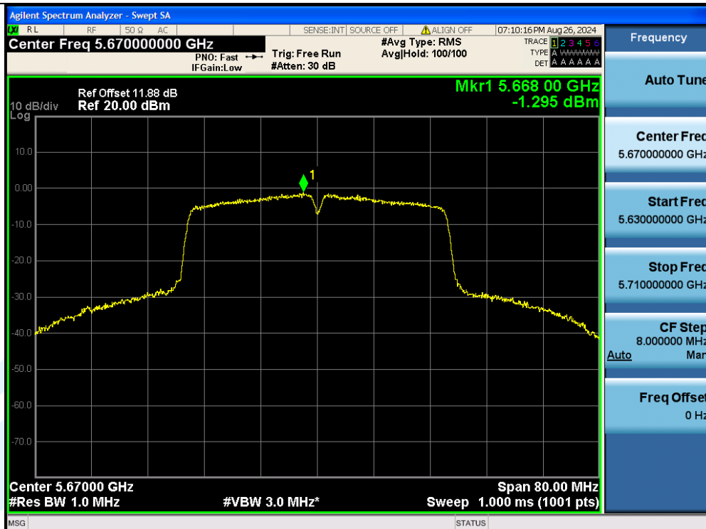
11N40MIMO-Ant2-5670-PASS
