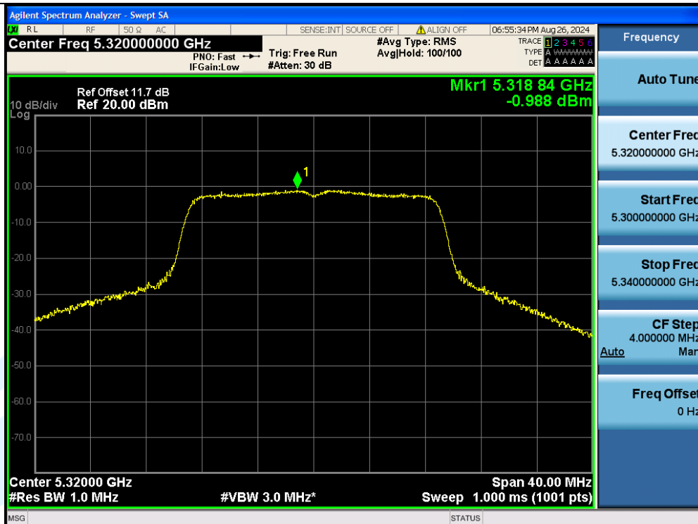
11N20MIMO-Ant2-5320-PASS
