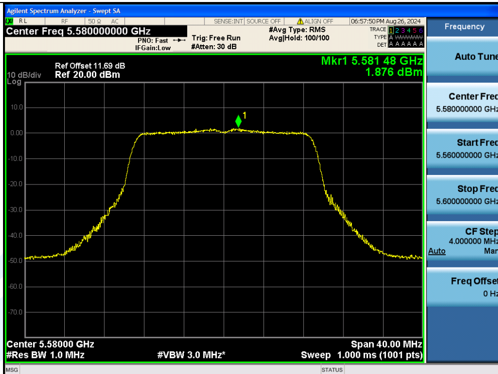
11N20MIMO-Ant2-5580-PASS
