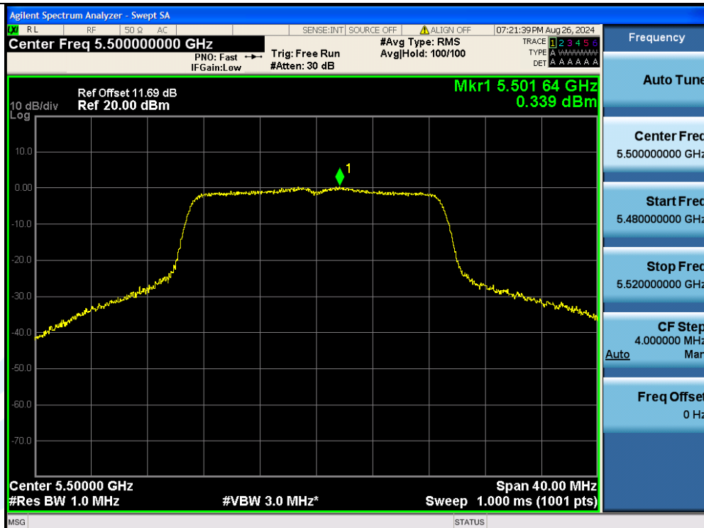
11AC20MIMO-Ant2-5500-PASS
