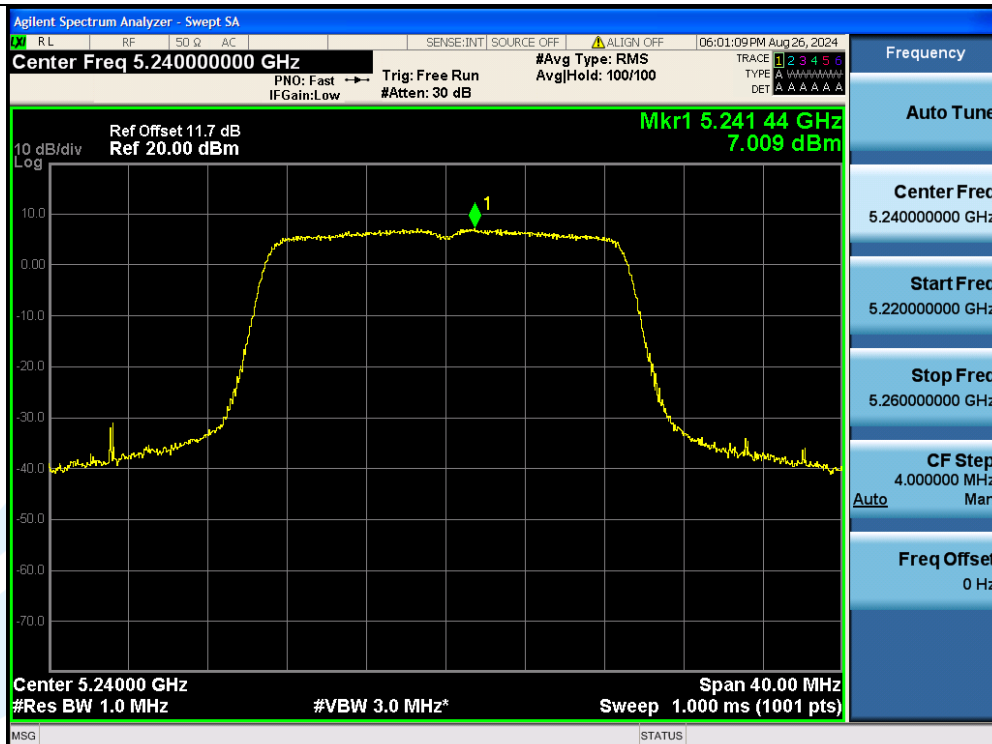
11N20MIMO-Ant2-5240-PASS
