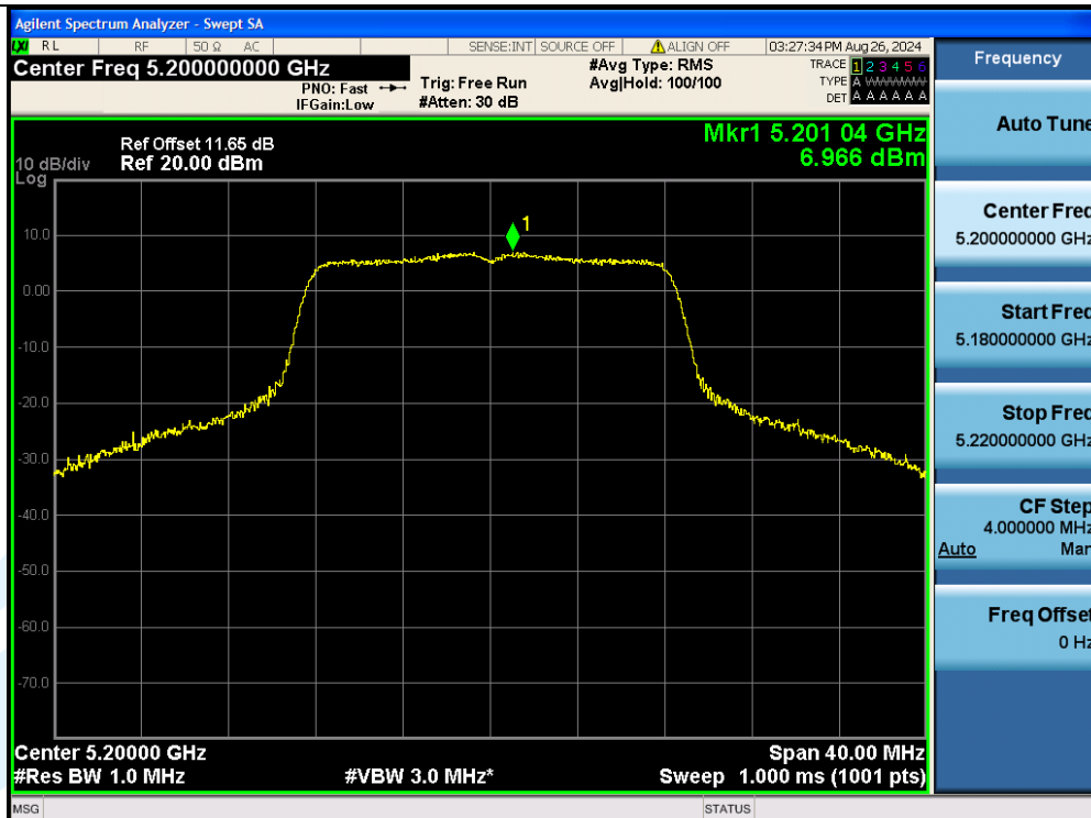
11A-Ant3-5200-PASS
