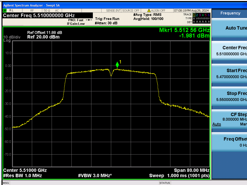
11N40MIMO-Ant2-5510-PASS
