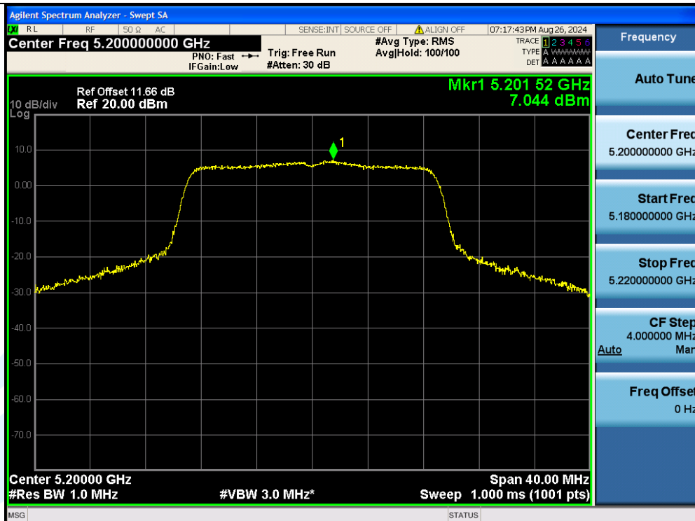
11AC20MIMO-Ant2-5200-PASS
