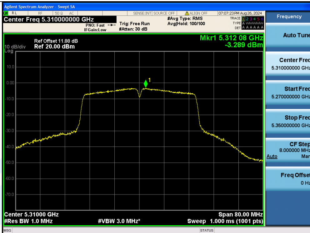
11N40MIMO-Ant2-5310-PASS
