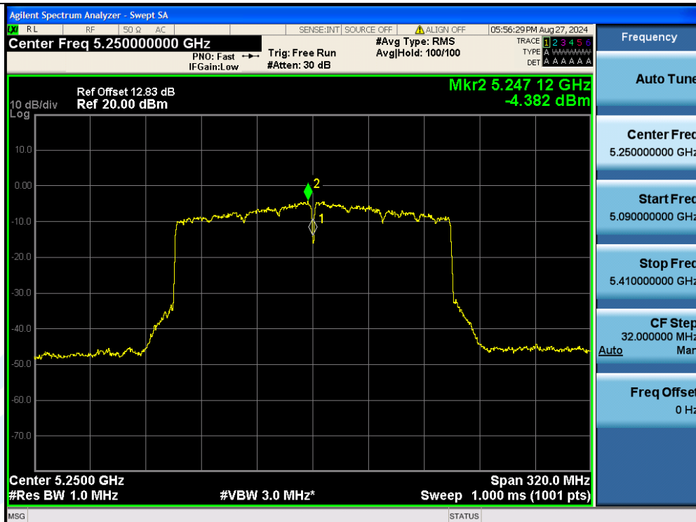
11AX160MIMO-Ant3-5250_UNII-1-PASS
