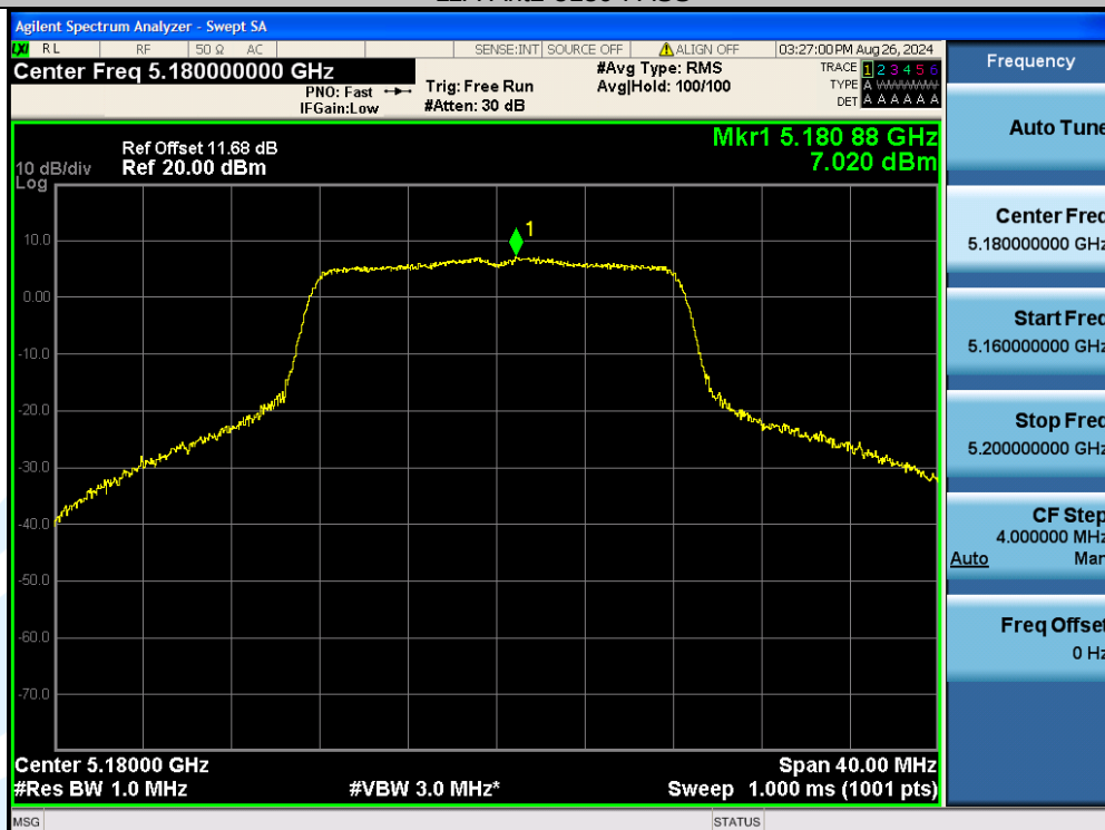
11A-Ant3-5180-PASS
