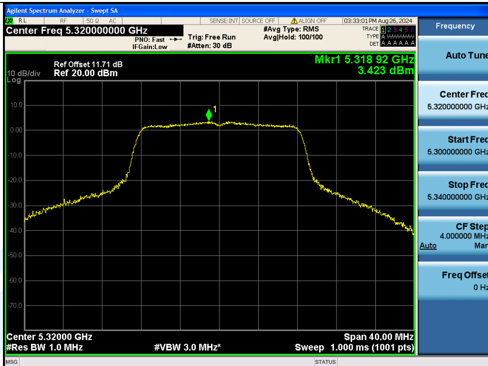
11A-Ant3-5320-PASS
