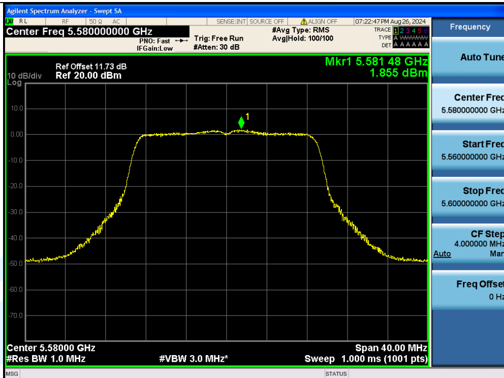
11AC20MIMO-Ant2-5580-PASS
