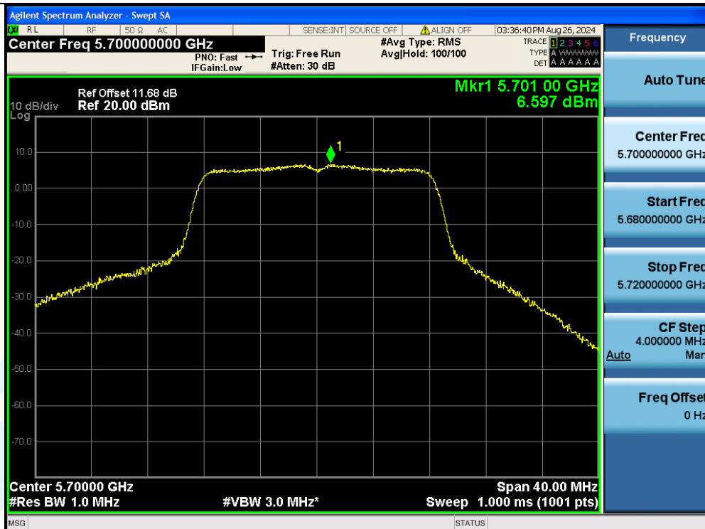
11A-Ant3-5700-PASS
