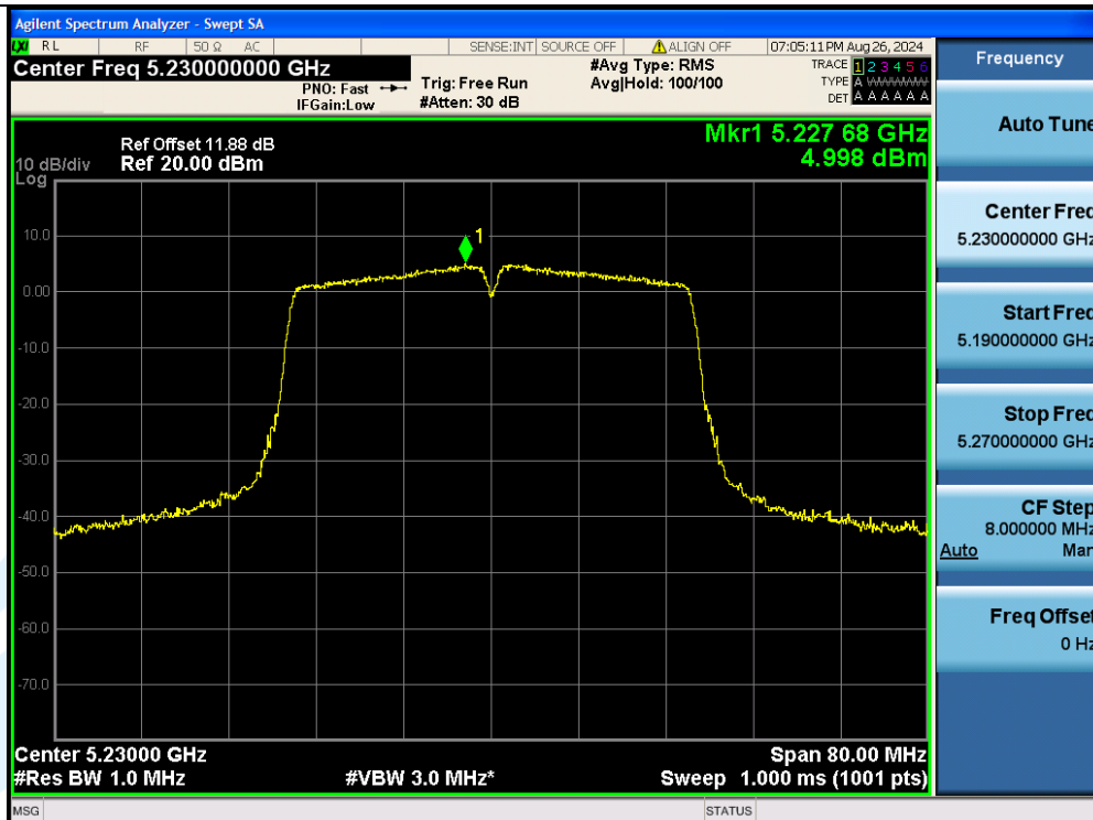
11N40MIMO-Ant2-5230-PASS
