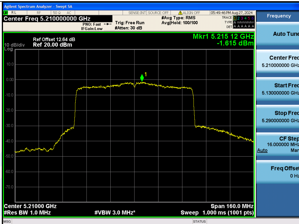
11AX80MIMO-Ant3-5210-PASS
