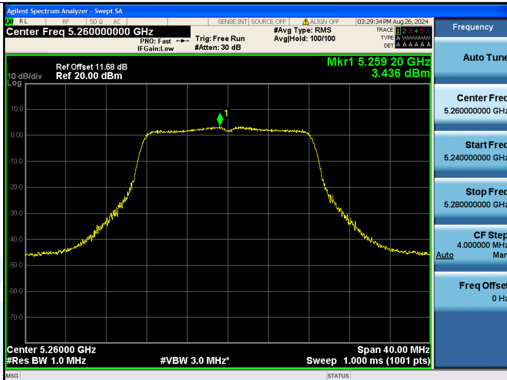
11A-Ant3-5260-PASS
