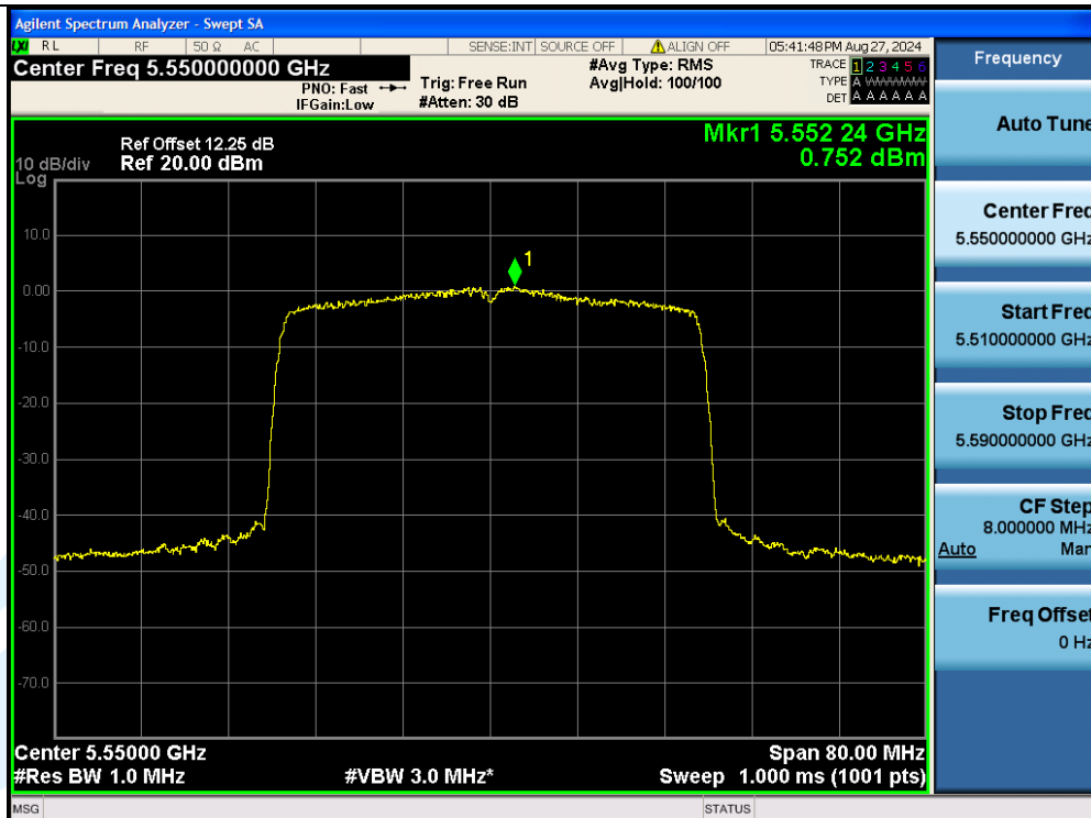
11AX40MIMO-Ant3-5550-PASS
