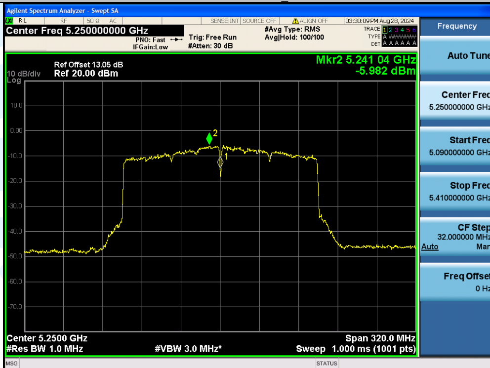
11AX160MIMO-Ant1-5250_UNII-2A-PASS
