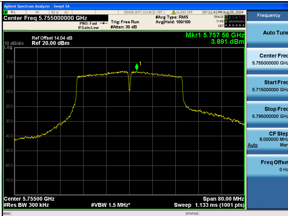
11N40MIMO-Ant2-5755-PASS
