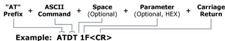
Figure A-1. Syntax for sending AT Commands
