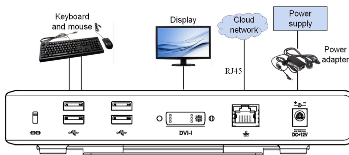
Figure 2-5 ZXCLoud iBOX CT220 Connections
