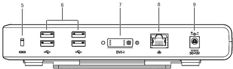
Figure 2-3 Back Panel
