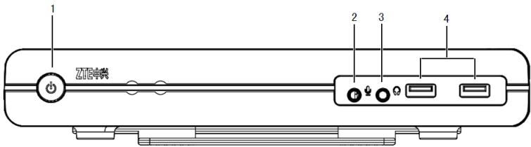
Figure 2-2 Front Panel
