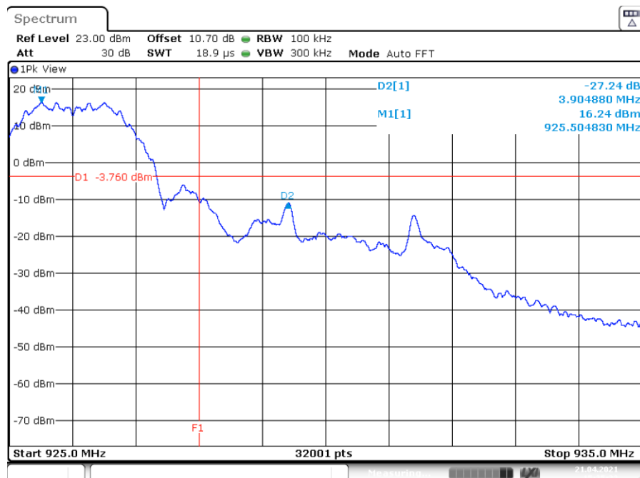
Figure 7.5.1.2-5: 926MHz Upper Band Edge
