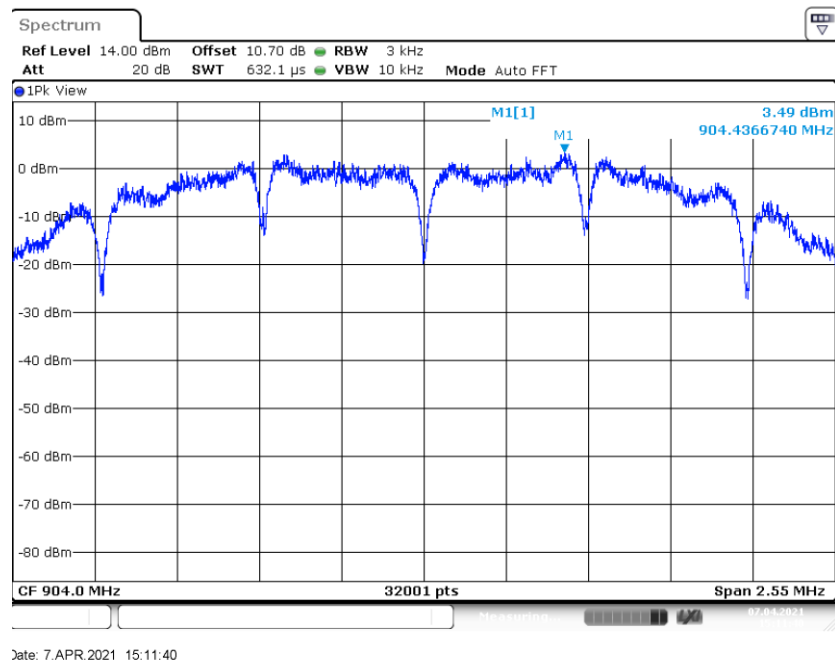
Figure 7.6.2-1: 904MHz LCH - PSD
