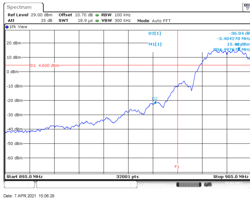
Figure 7.5.1.2-4: 904MHz Lower Band Edge
