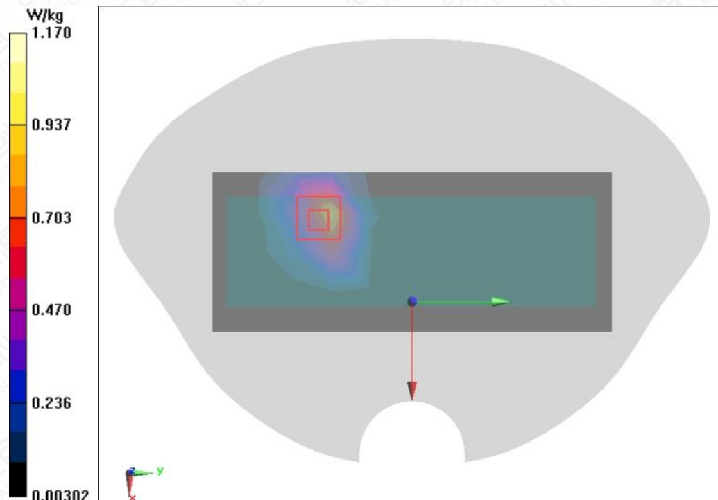
Figure A.1-15 LTE B7 20MHz 50RB 0offset Right Side Mode Middle 5mm
