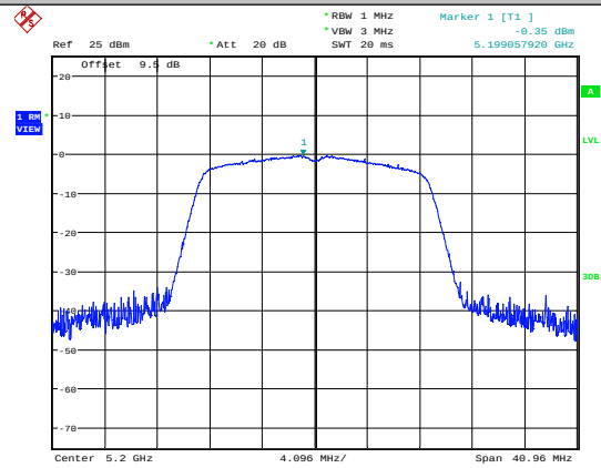
11AC20SISO-Ant1-5200
