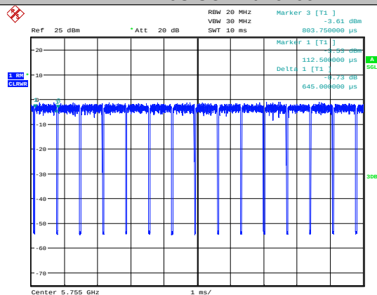
11N40SISO-Ant1-5755
