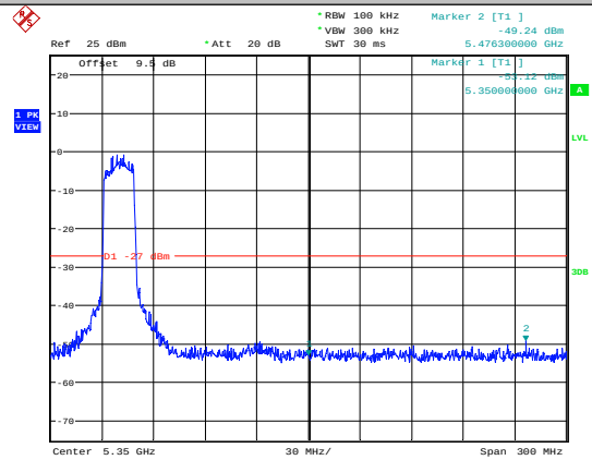
11AC20SISO-Ant1-5240
