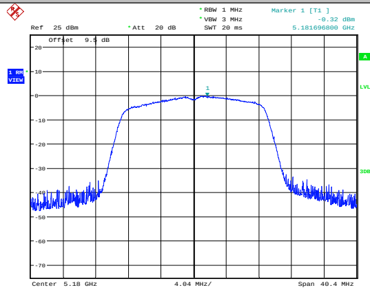
11AC20SISO-Ant1-5180
