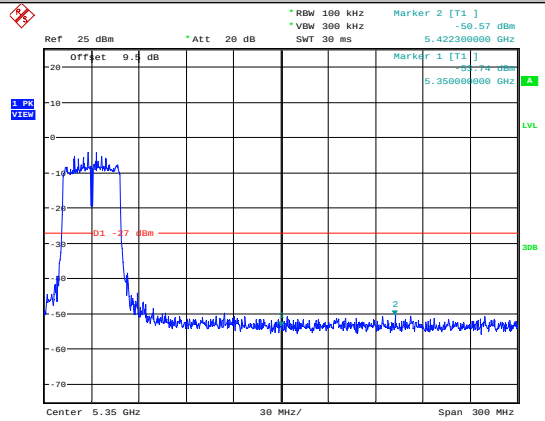
11N40SISO-Ant1-5230
