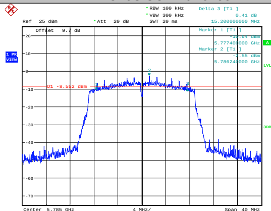
11AC20SISO-Ant1-5785
