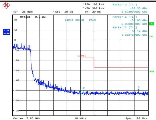
11N40SISO-Ant1-5795
