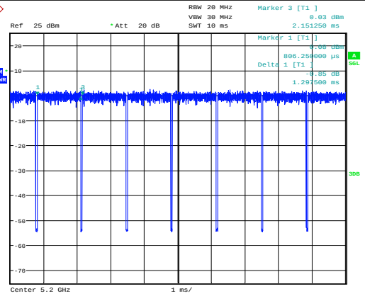
11N20SISO-Ant1-5200
