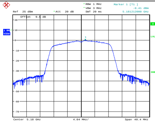
11N20SISO-Ant1-5180
