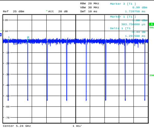
11N20SISO-Ant1-5240
