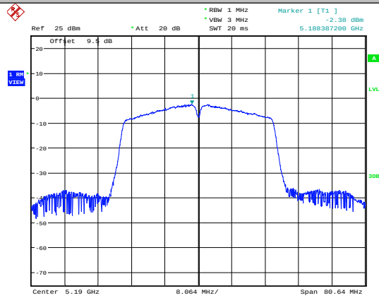
11N40SISO-Ant1-5190
