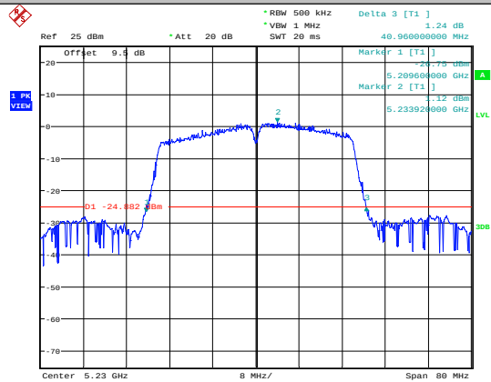
11N40SISO-Ant1-5230
