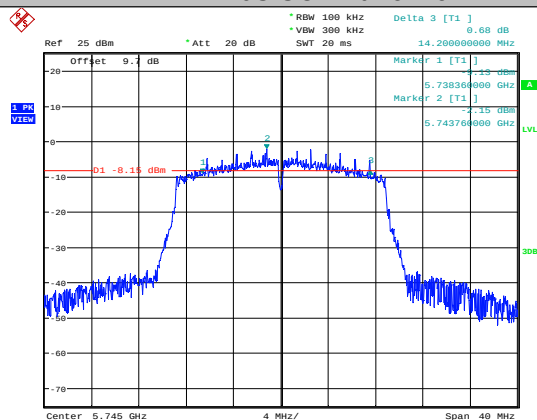
11N20SISO-Ant1-5745
