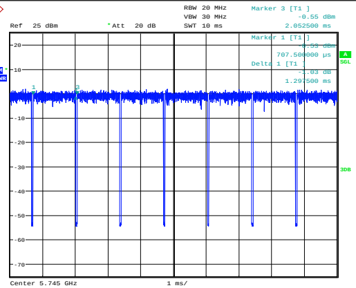
11N20SISO-Ant1-5745
