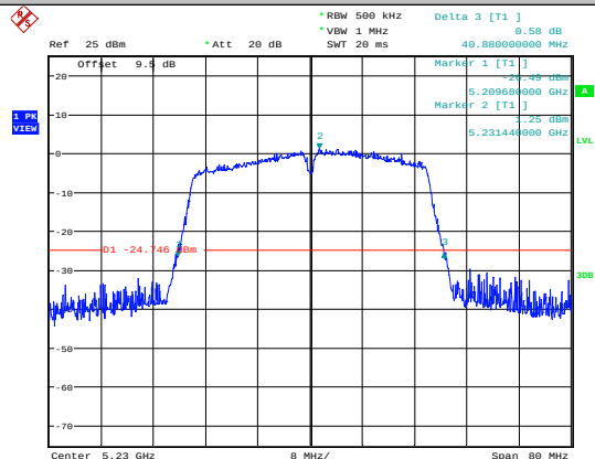
11AC40SISO-Ant1-5230
