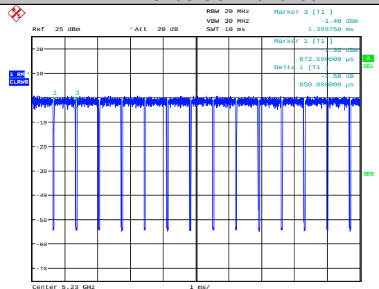
11AC40SISO-Ant1-5230
