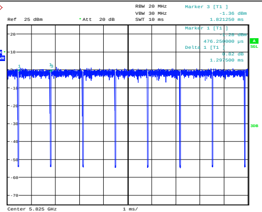
11N20SISO-Ant1-5825
