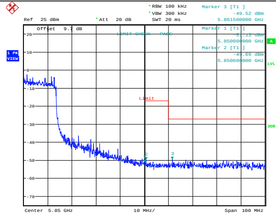
11AC40SISO-Ant1-5795
