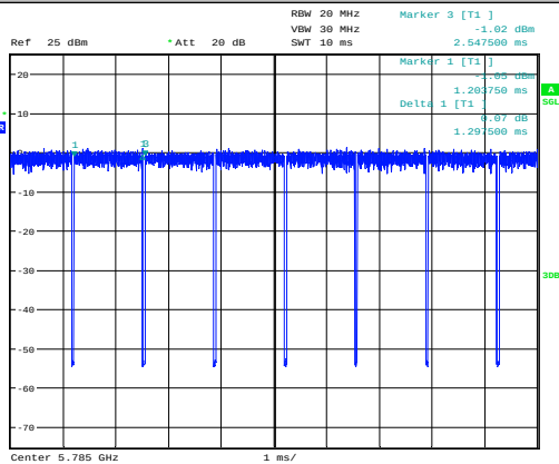
11N20SISO-Ant1-5785
