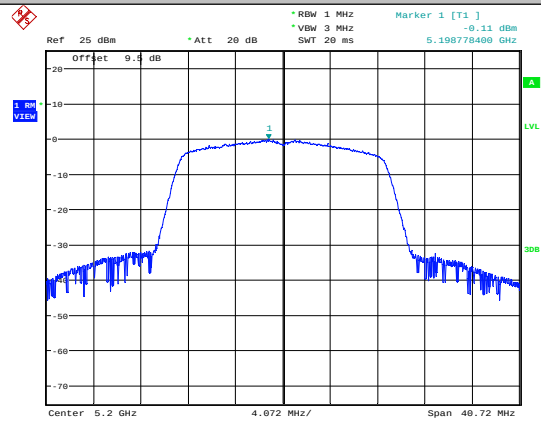
11N20SISO-Ant1-5200
