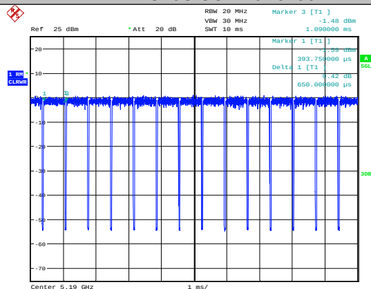
11AC40SISO-Ant1-5190
