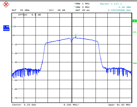
11N40SISO-Ant1-5230
