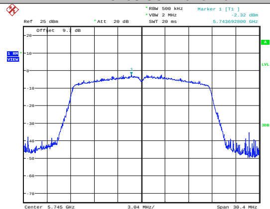
11AC20SISO-Ant1-5745
