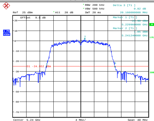
11N20SISO-Ant1-5240
