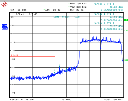
11N40SISO-Ant1-5755
