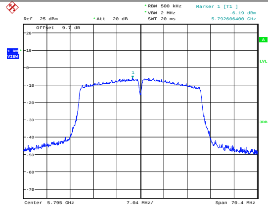
11AC40SISO-Ant1-5795
