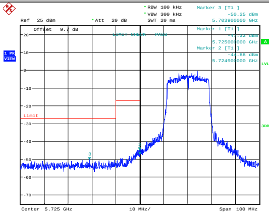
11N20SISO-Ant1-5745
