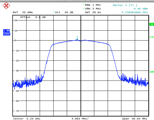
11AC20SISO-Ant1-5240
