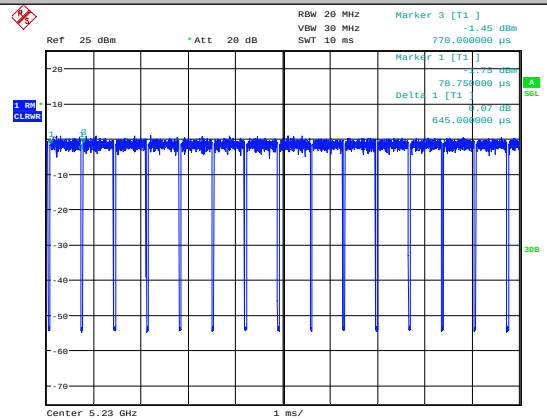
11N40SISO-Ant1-5230
