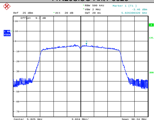
11N20SISO-Ant1-5825
