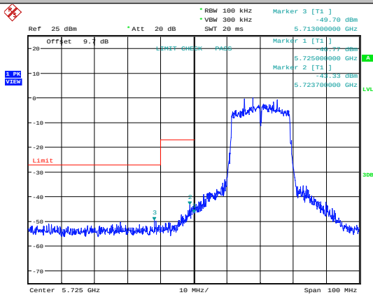
11AC20SISO-Ant1-5745
