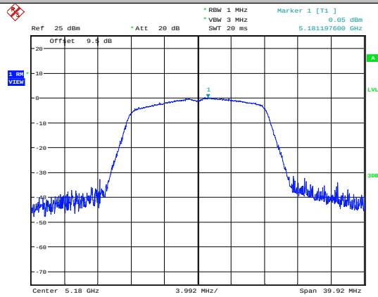
11A-Ant1-5180
