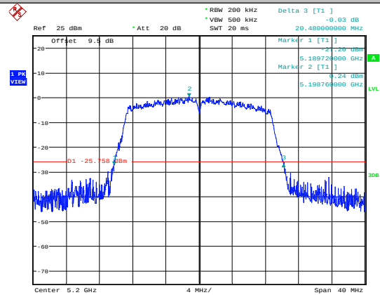
11AC20SISO-Ant1-5200
