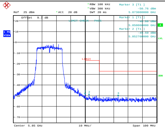
11N20SISO-Ant1-5825
