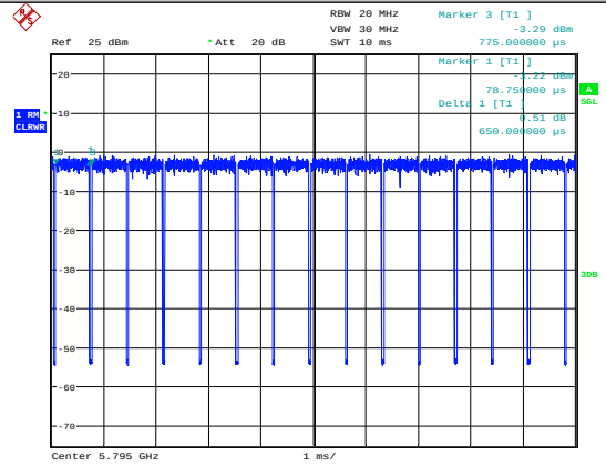
11AC40SISO-Ant1-5795
