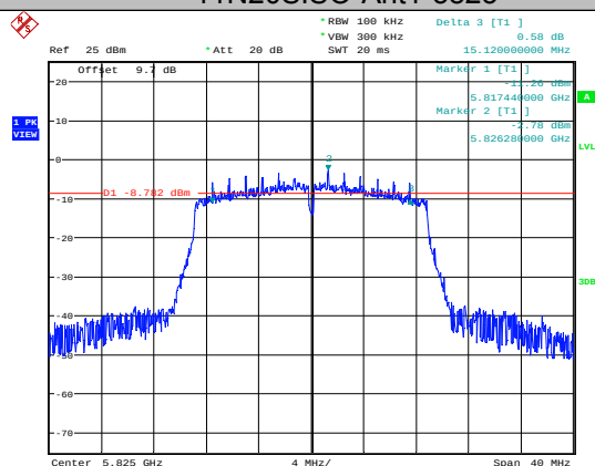
11N20SISO-Ant1-5825
