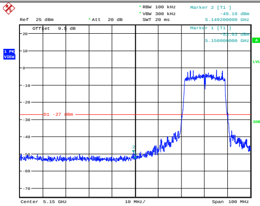
11AC20SISO-Ant1-5180
