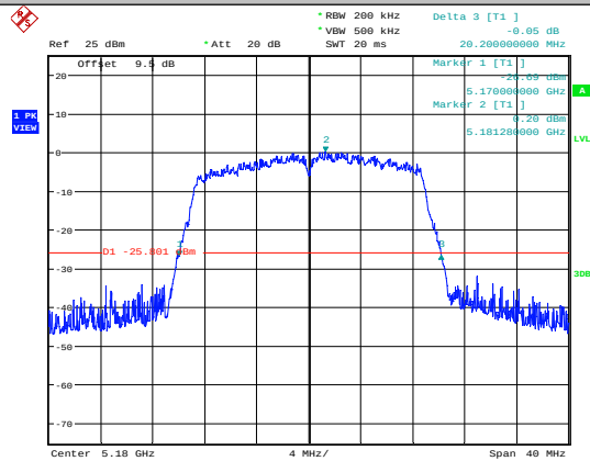
11AC20SISO-Ant1-5180
