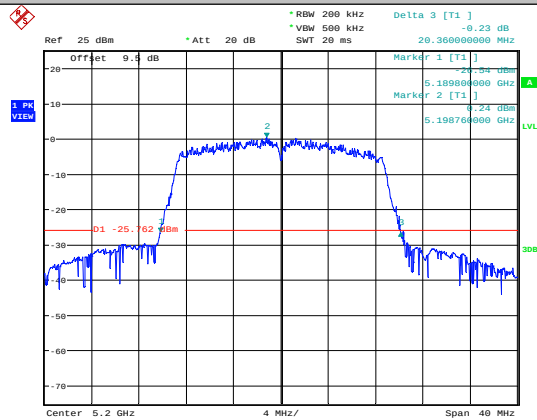
11N20SISO-Ant1-5200
