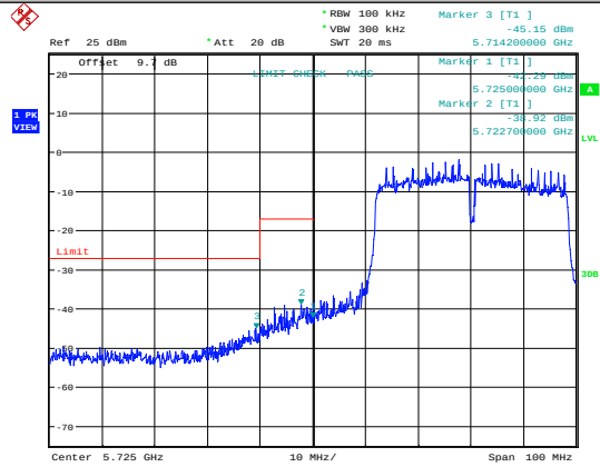
11AC40SISO-Ant1-5755
