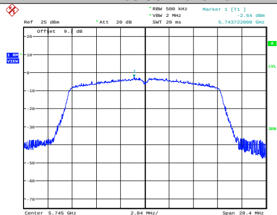
11N20SISO-Ant1-5745
