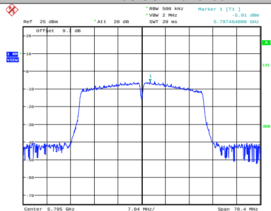
11N40SISO-Ant1-5795
