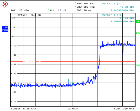
11N40SISO-Ant1-5190
