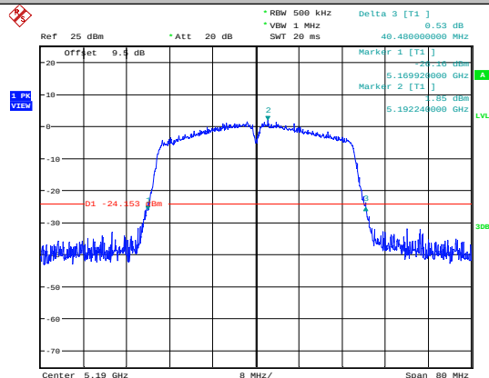
11AC40SISO-Ant1-5190
