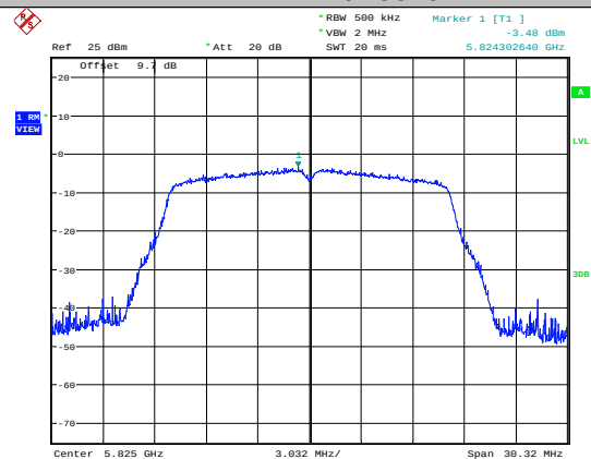
11A-Ant1-5825
