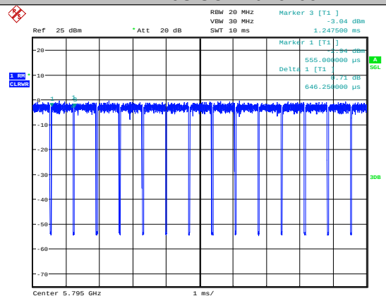
11N40SISO-Ant1-5795
