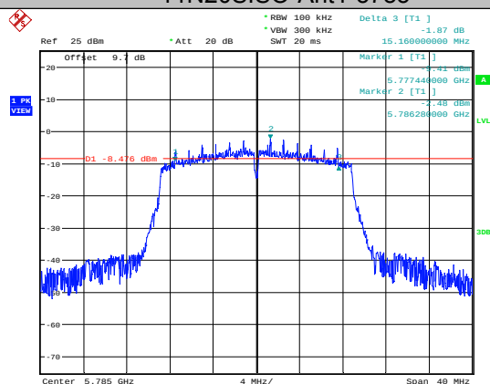
11N20SISO-Ant1-5785
