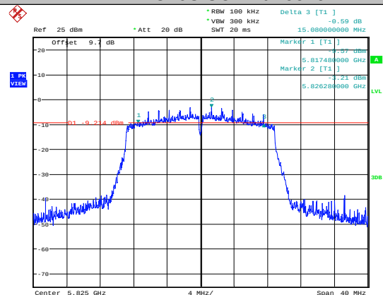
11AC20SISO-Ant1-5825
