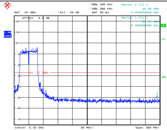
11AC40SISO-Ant1-5230
