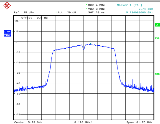
11AC40SISO-Ant1-5230
