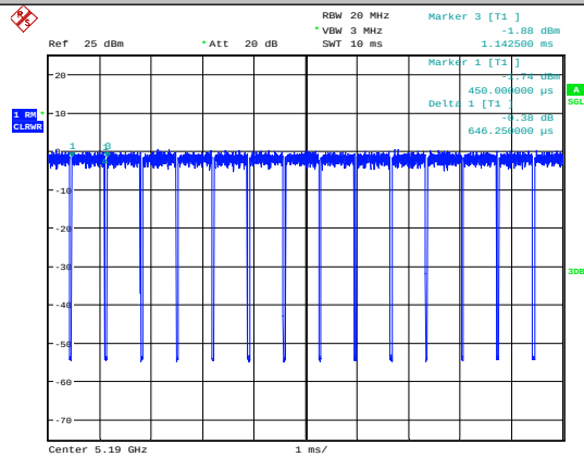
11N40SISO-Ant1-5190
