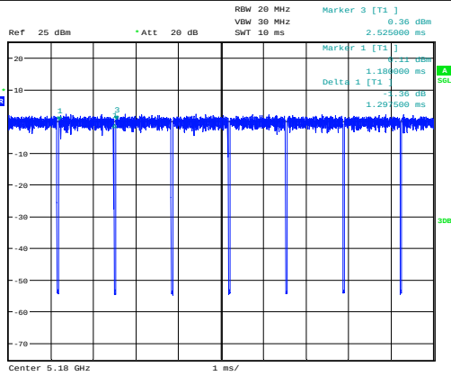
11N20SISO-Ant1-5180
