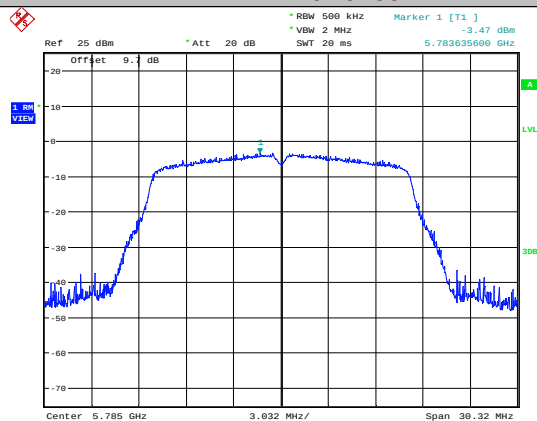
11A-Ant1-5785
