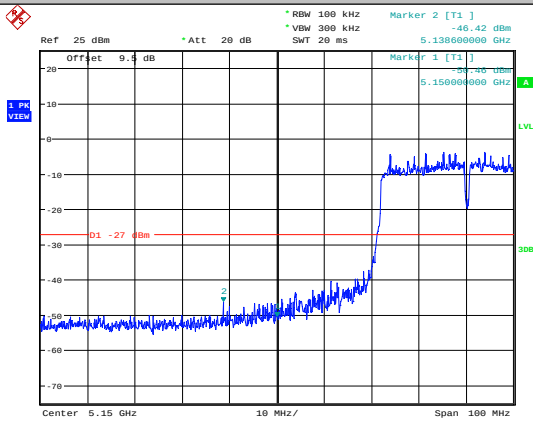
11AC40SISO-Ant1-5190
