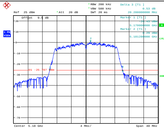
11N20SISO-Ant1-5180
