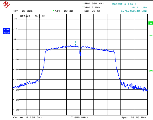
11AC40SISO-Ant1-5755
