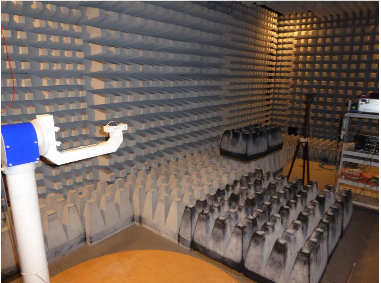
172289_E3_06.jpg: Test setup fully anechoic chamber
