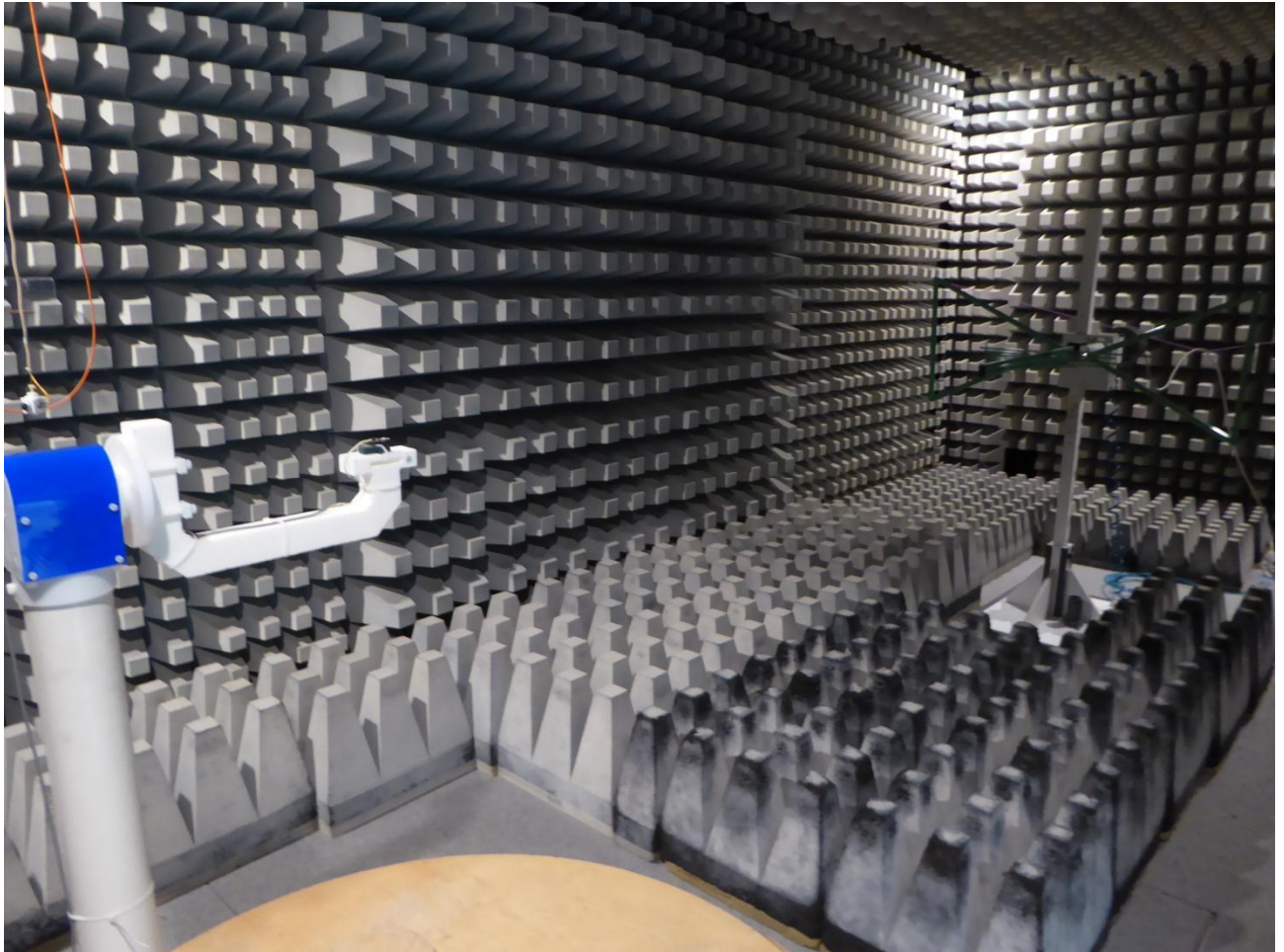
172289_E3_03.jpg: Test setup fully anechoic chamber (preliminary measurement)
