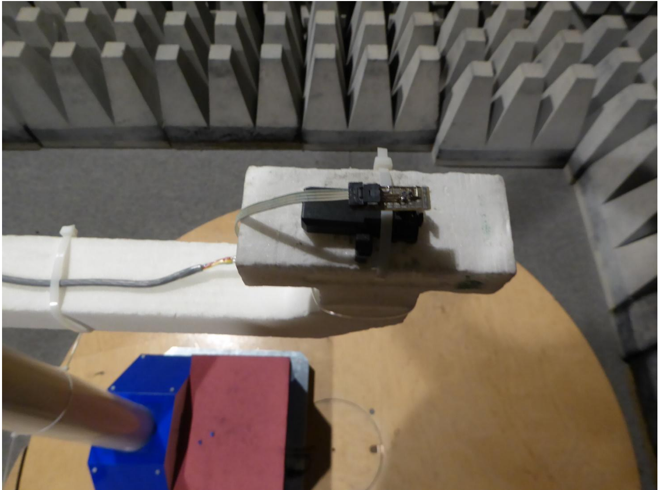
172289_E3_01.jpg: Test setup Test setup fully anechoic chamber
