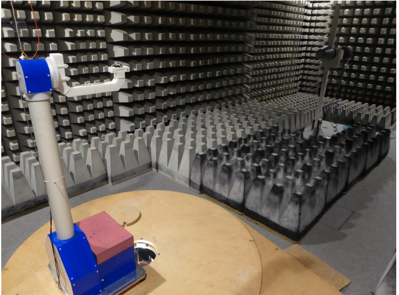
172289_E3_04.jpg: Test setup fully anechoic chamber
