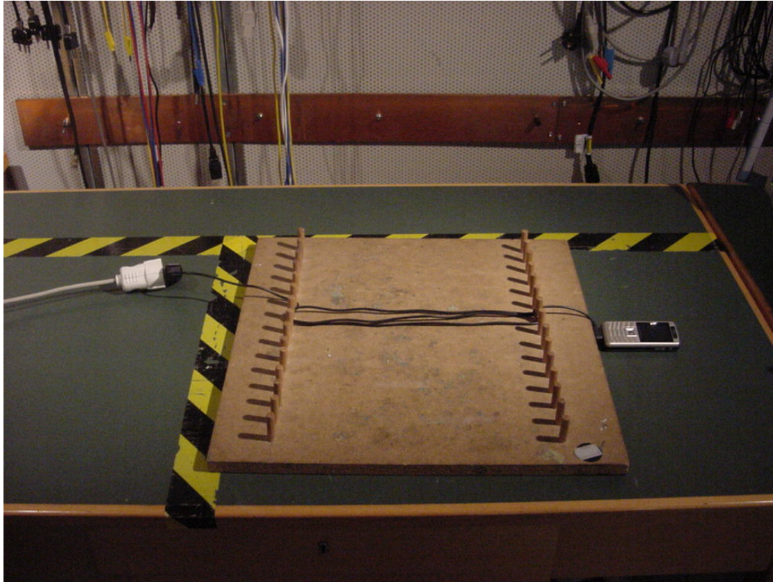
Photo 2: Conducted Emissions
