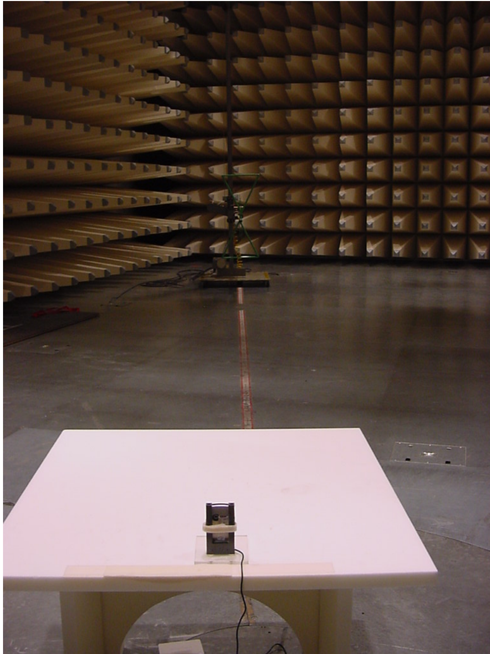
Photo 1: Radiated Emissions
