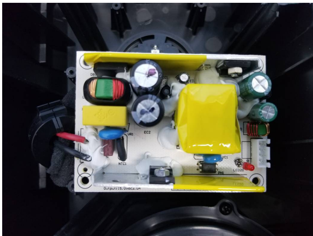
Photo 8 (2# Power board)
