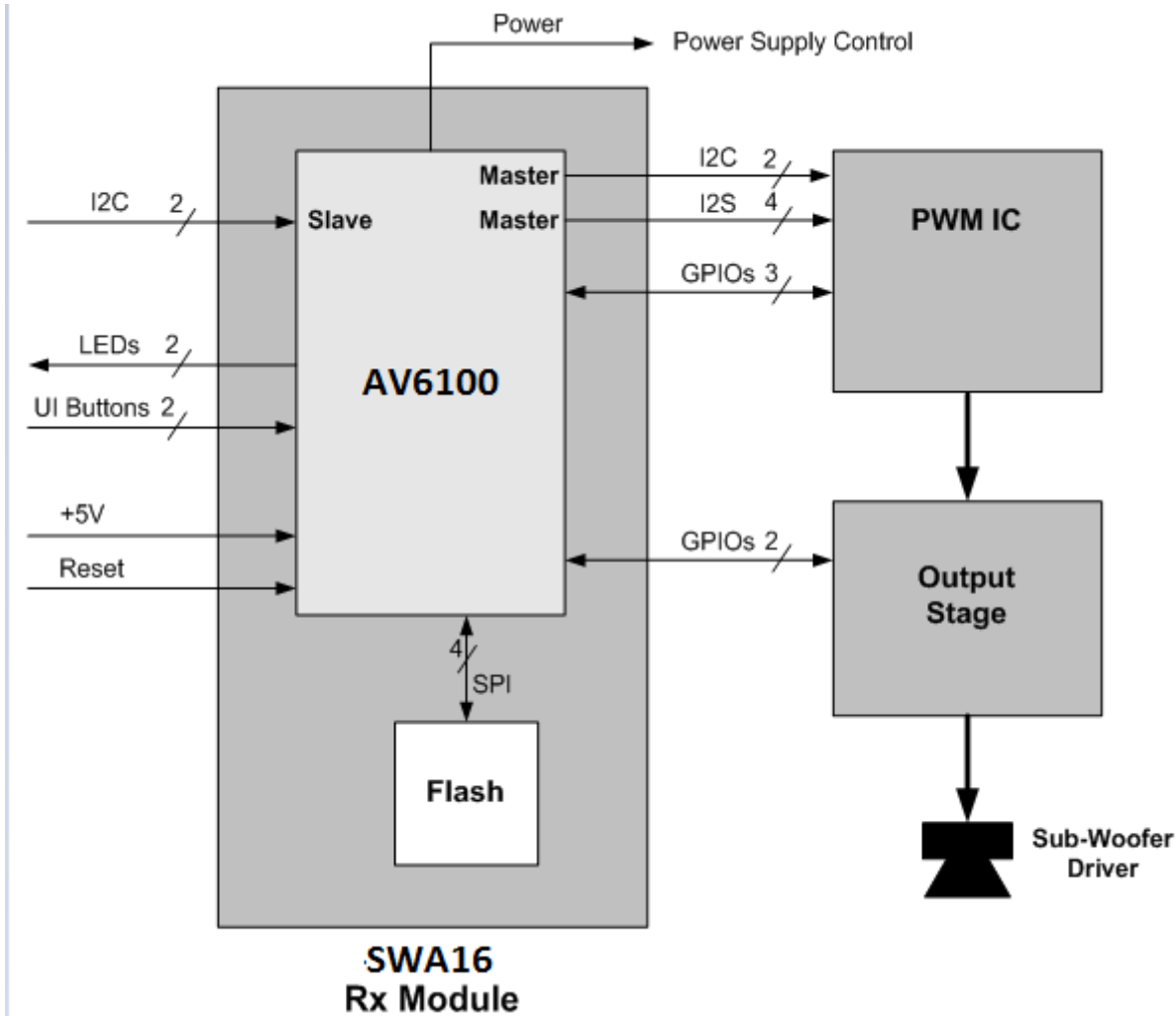
Figure 1: SWA16 RX Module Simple Sub-Woofer Implementation
