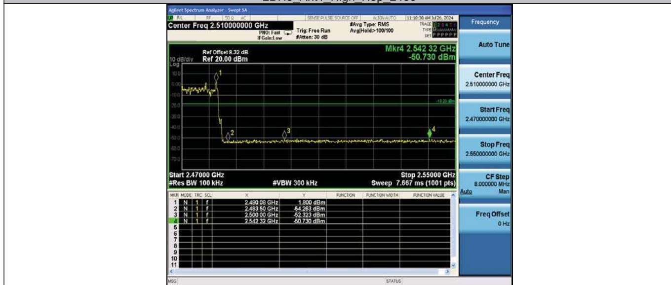
2DH5_Ant2_High_Hop_2480
