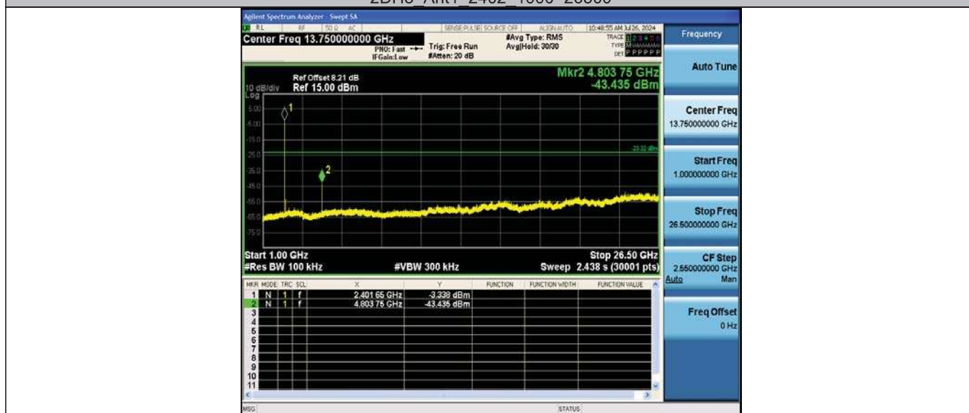
2DH5_Ant2_2402_0~Reference
