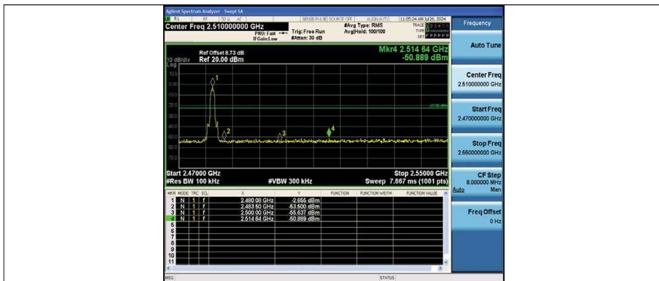
3DH5_Ant2_High_2480
