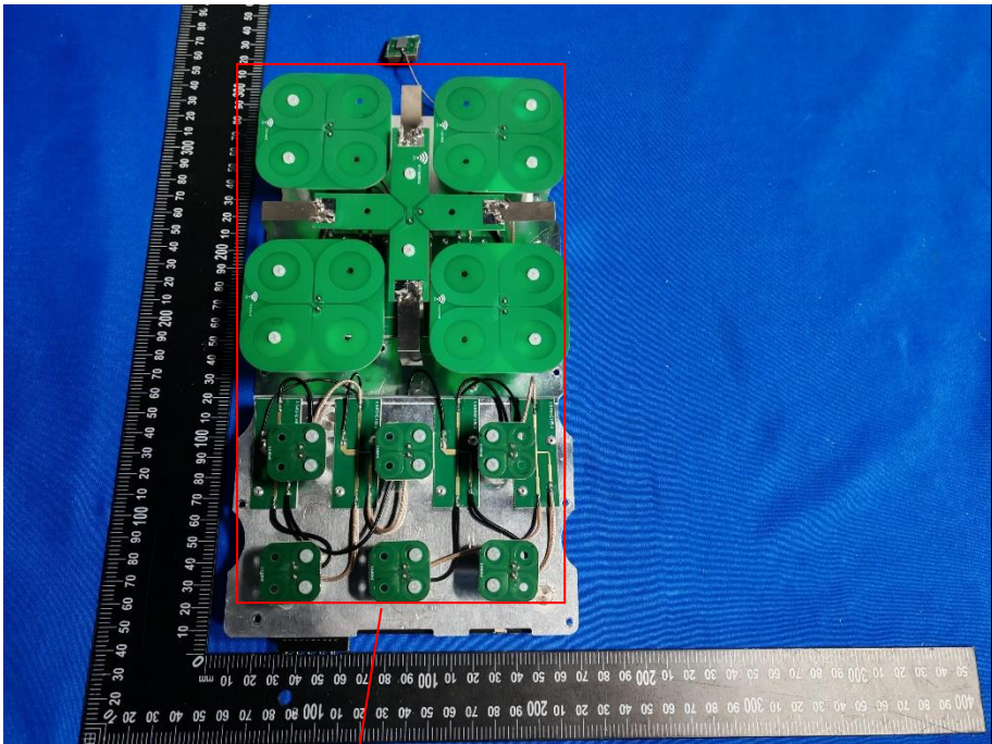
WCDMA/ LTE/NR5G Antenna
