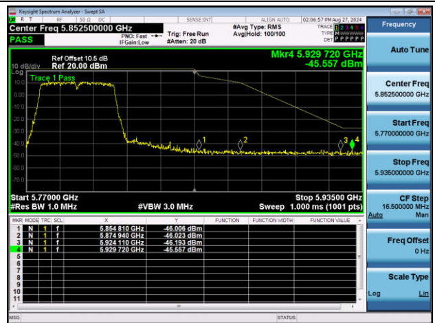
11N40SISO-Ant2-5795-PASS
