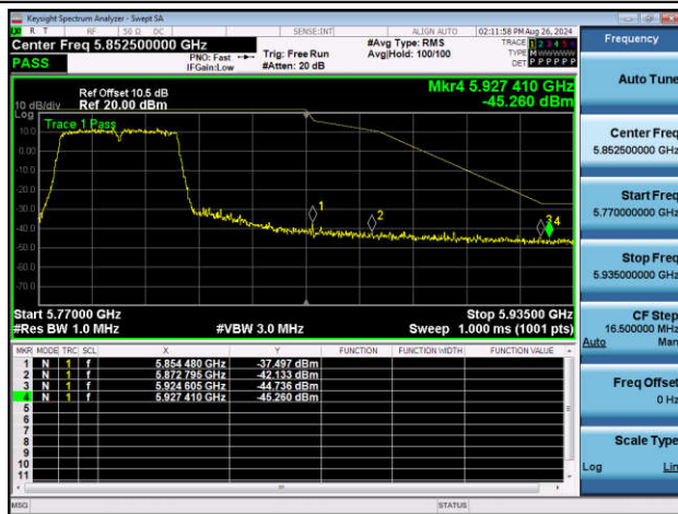
11N40SISO-Ant1-5795-PASS
