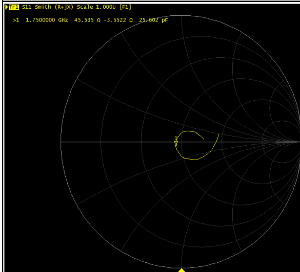
Impedance Test-Body
