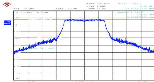
n20_5180MHz_Chain 0
