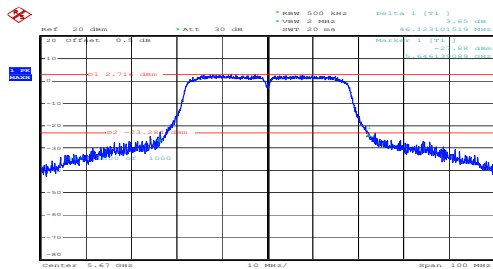
n40_5670MHz_Chain 0
