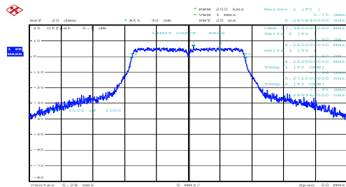
n20_5280MHz_Chain 0
