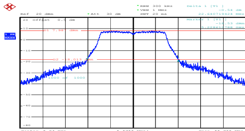
a_5240MHz_Chain 0
