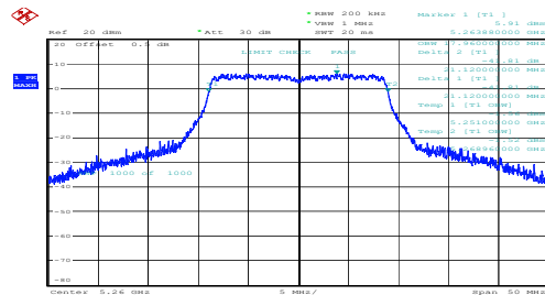
n20_5260MHz_Chain 0
