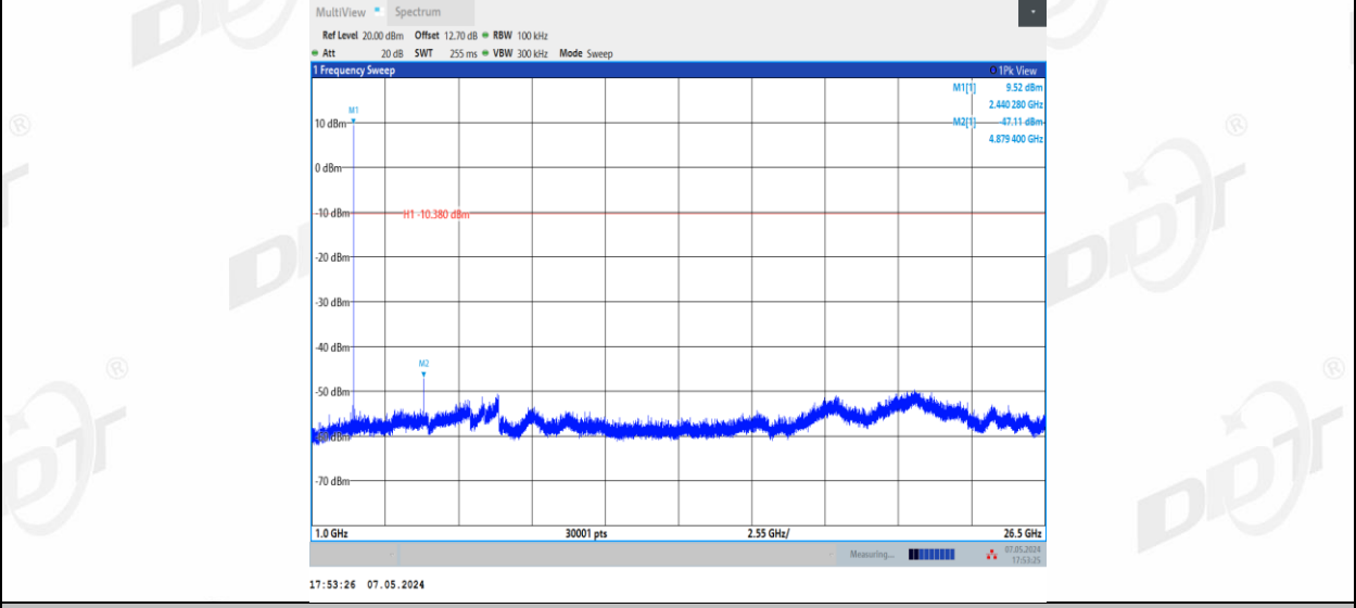
BLE_1M_Ant2_R_2440_0~Reference
