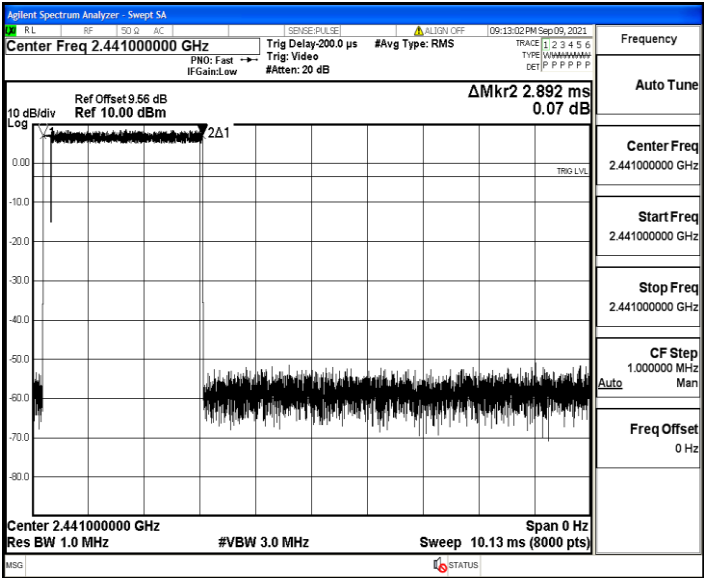
3DH5_Ant3_Hop
