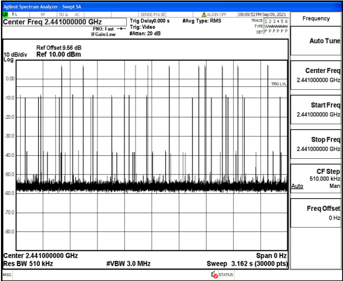
3DH5_Ant3_Hop
