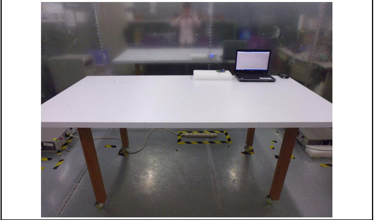
Conducted Emission Test (Chip Antenna)
