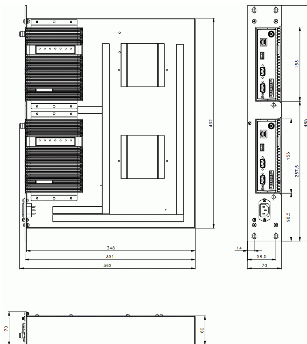
Fig. 4.29: 19" Rack shelf-double – dimensions
