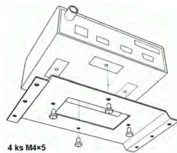
Fig. 6.7: Vertical lengthwise mounting to DIN rail
