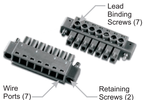
Fig. 4.9: Power and Control - cable plug
