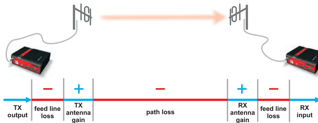
Fig. 3.2: Signal path
