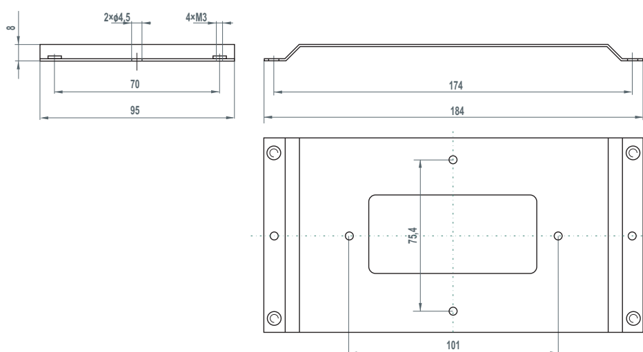
Fig. 4.25: Flat-bracket dimensions
