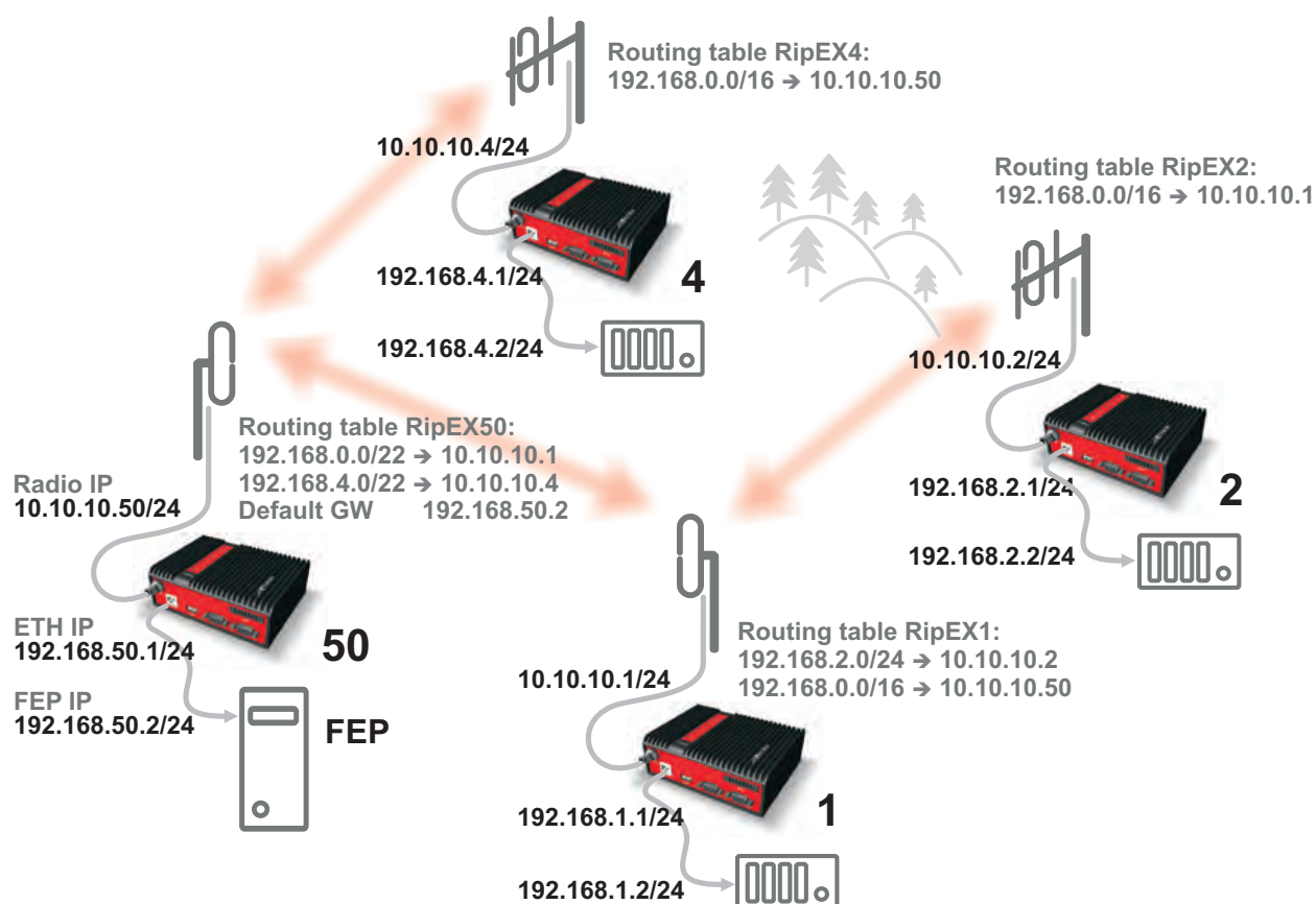
Fig. 2.3: Optimised addressing
