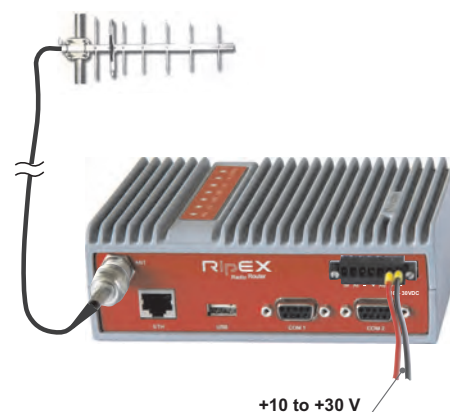
Fig. 6.9: 10–30 VDC Supplying
