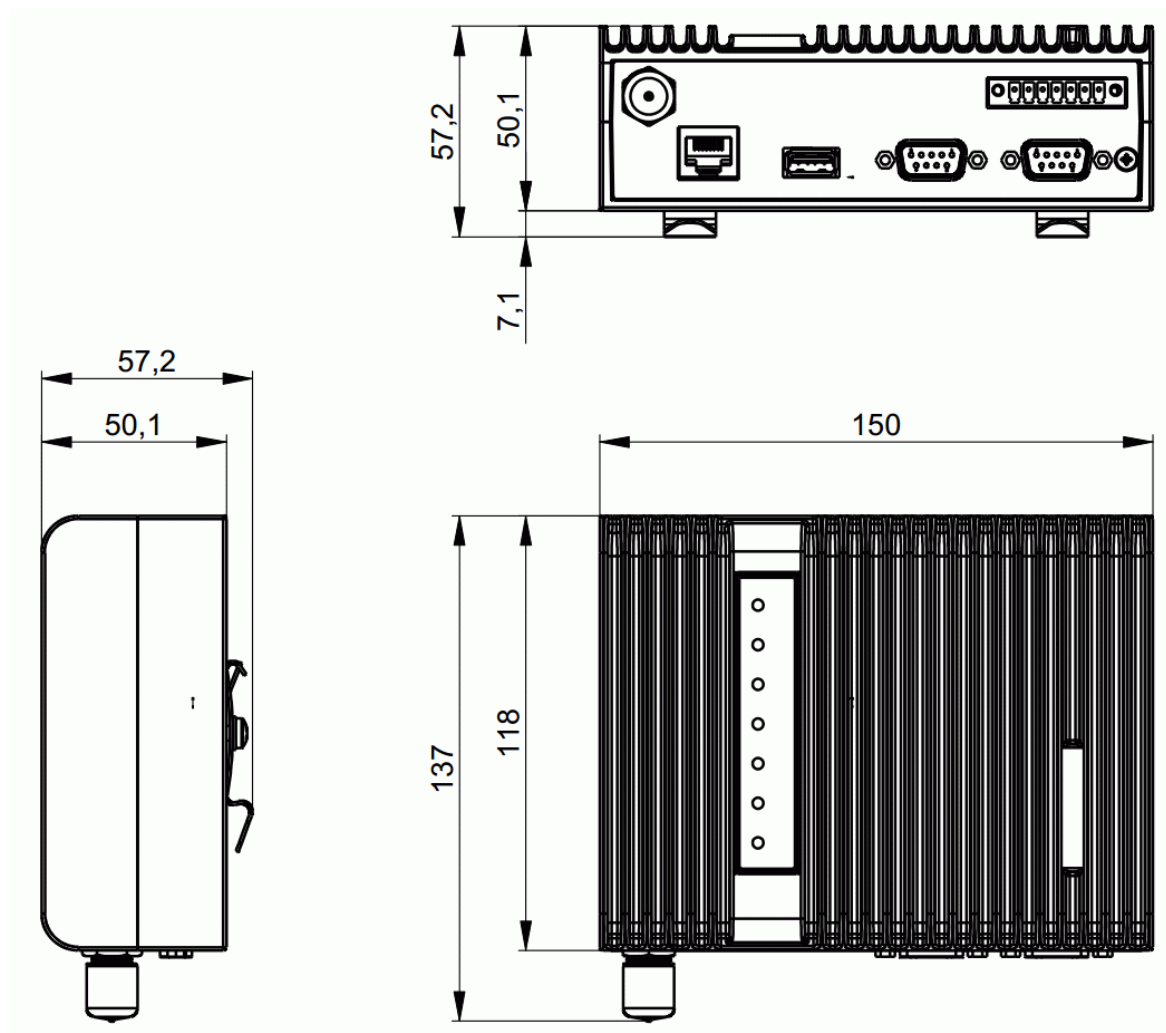
Fig. 4.1: RipEX dimensions
