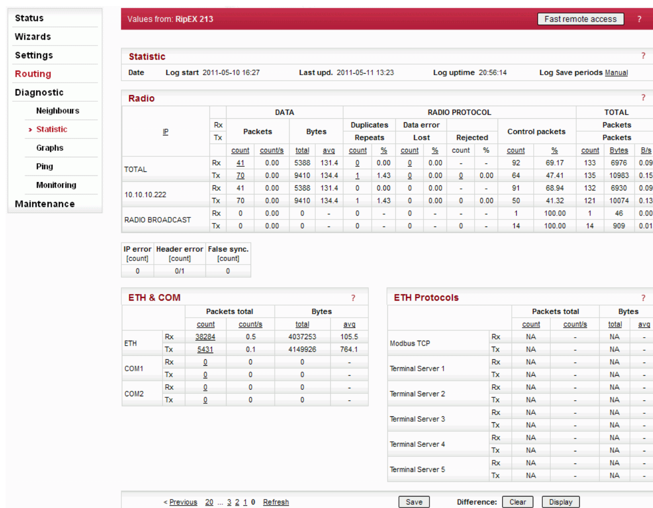
Fig. 7.11: Menu Statistic
