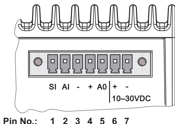
Fig. 4.8: Supply connector
