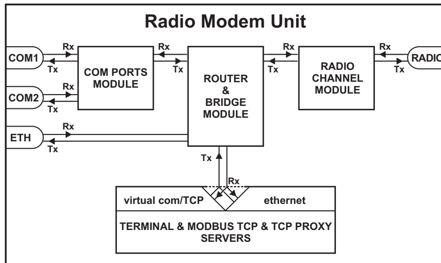
Fig. 7.15: Monitoring
