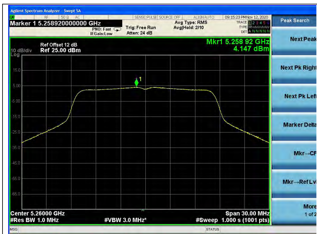
(Channel 52, 5260MHz, 802.11a, ANT2)
