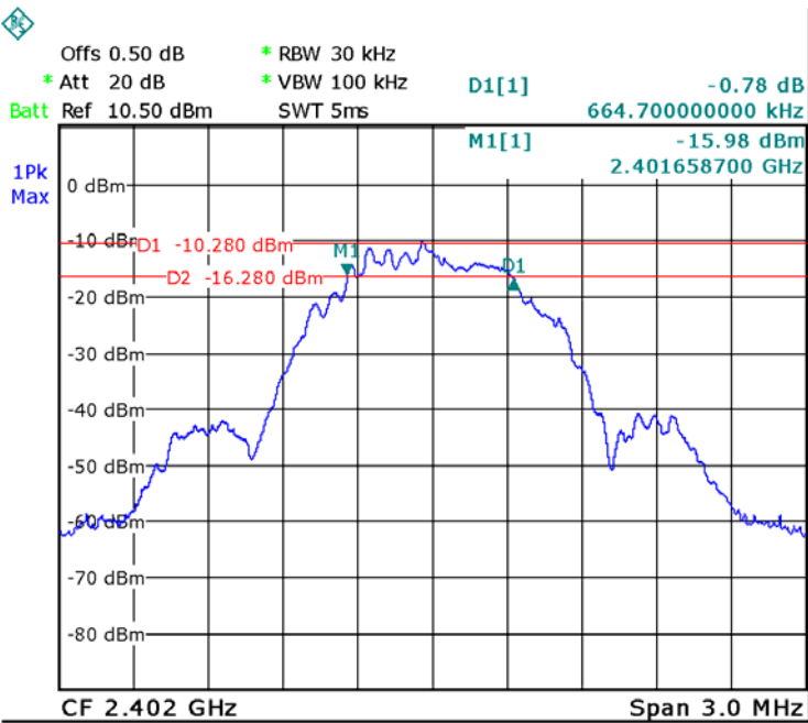
Mode: TX BT BLE channel 1
