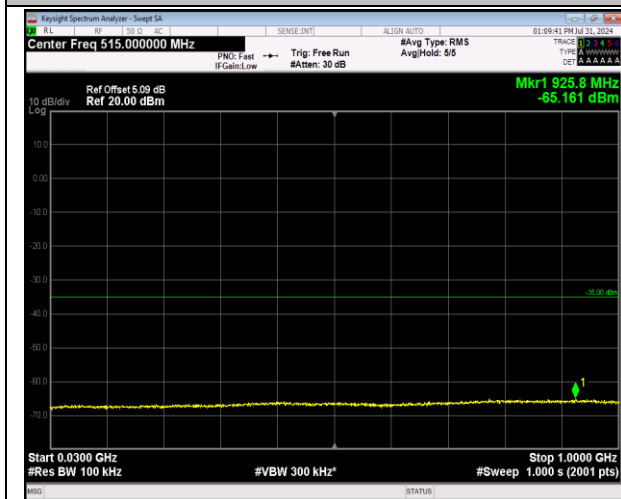
7-7-20MHz-10MHz-64QAM-64QAM-21251-21395-100R B#0-50RB#0-30~1000MHz-PASS
