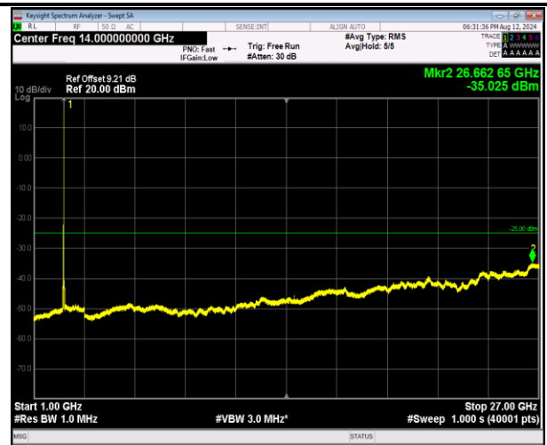
7-7-20MHz-20MHz-16QAM-16QAM-21152-21350-1RB#9 9-0RB#0-1000~27000MHz-PASS
