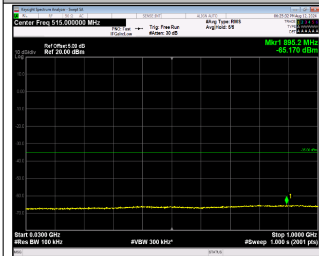
7-7-20MHz-20MHz-QPSK-QPSK-21001-21199-1RB#99-0 ORB#0-30~1000MHz-PASS
