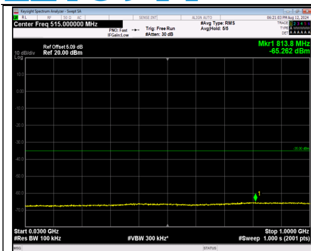
7-7-20MHz-20MHz-16QAM-16QAM-20850-21048-1RB# 99-0RB#0-30~1000MHz-PASS
