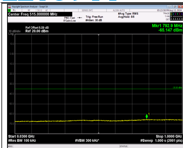
7-7-20MHz-10MHz-16QAM-16QAM-21051-21195-1RB# 99-0RB#0-30~1000MHz-PASS
