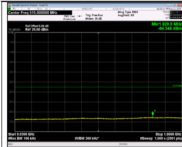
7-7-20MHz-20MHz-16QAM-16QAM-21001-21199-1RB# 99-0RB#0-30~1000MHz-PASS
