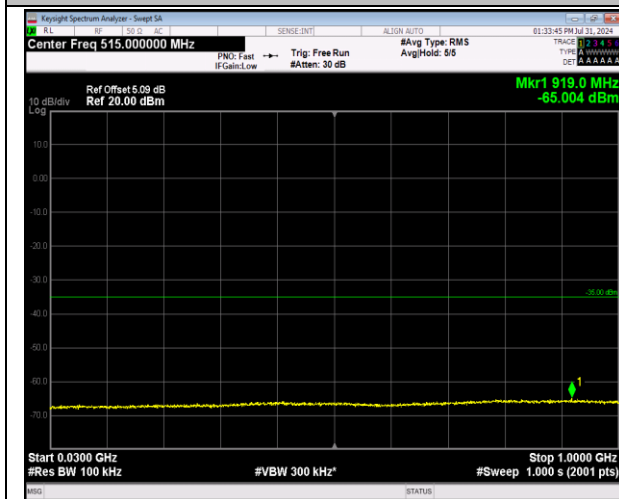
7-7-20MHz-20MHz-64QAM-64QAM-21001-21199-1RB# 0-0RB#0-30~1000MHz-PASS
