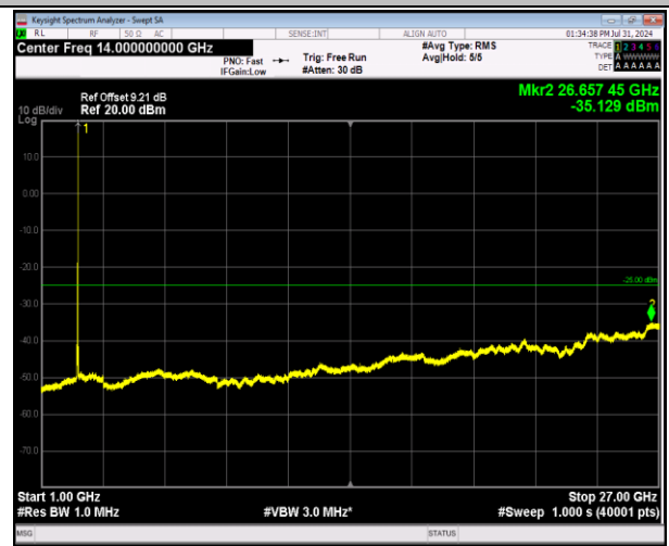
7-7-20MHz-20MHz-64QAM-64QAM-21001-21199-1RB#9 9-0RB#0-1000~27000MHz-PASS
