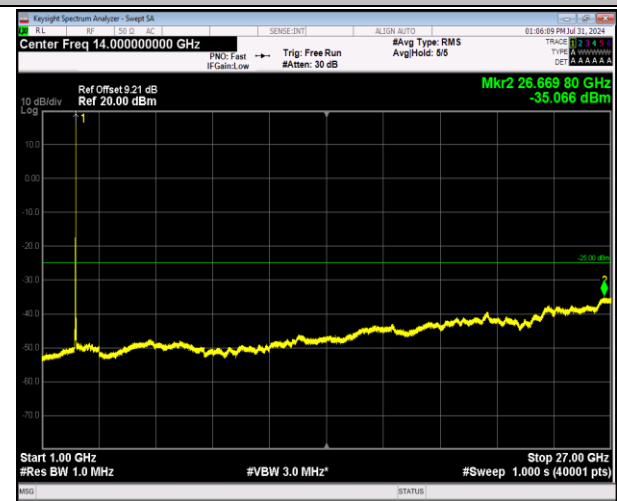
7-7-20MHz-10MHz-64QAM-64QAM-21051-21195-1RB#9 9-0RB#0-1000~27000MHz-PASS
