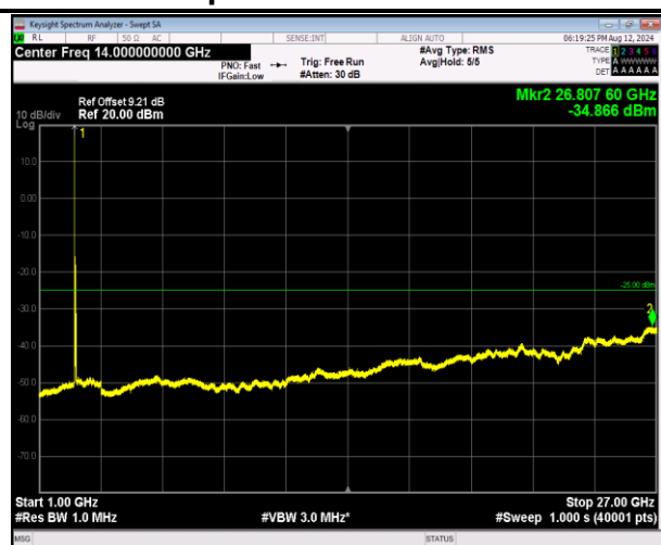
7-7-20MHz-20MHz-QPSK-QPSK-20850-21048-1RB#0-0 RB#0-1000~27000MHz-PASS
