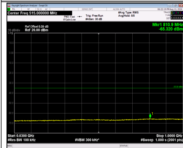
7-7-20MHz-20MHz-16QAM-16QAM-20850-21048-1RB# 0-1RB#99-30~1000MHz-PASS
