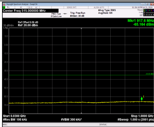
7-7-20MHz-20MHz-64QAM-64QAM-21152-21350-1RB# 0-0RB#0-30~1000MHz-PASS
