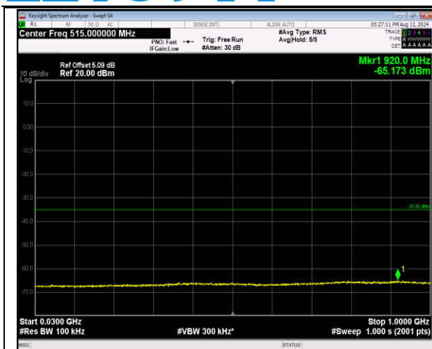
7-7-20MHz-10MHz-QPSK-QPSK-21251-21395-1RB#0-0 RB#0-30~1000MHz-PASS
