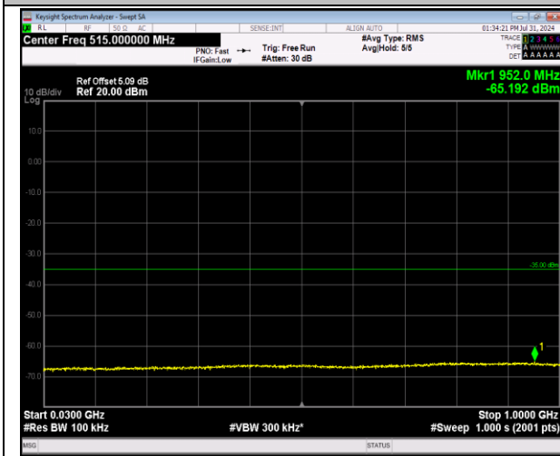
7-7-20MHz-20MHz-64QAM-64QAM-21001-21199-1RB# 99-0RB#0-30~1000MHz-PASS
