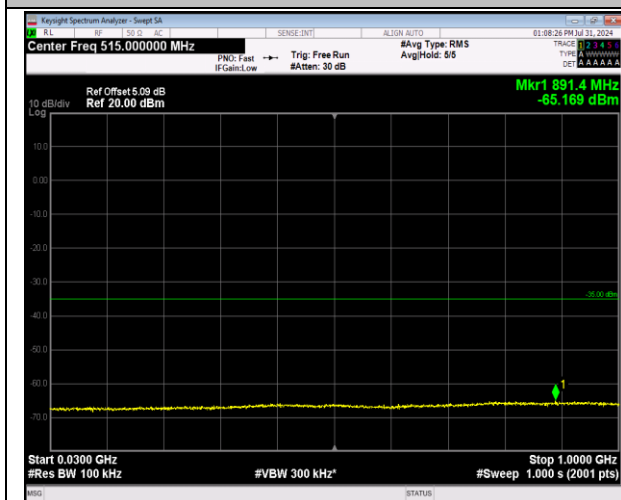
7-7-20MHz-10MHz-64QAM-64QAM-21251-21395-1RB# 99-0RB#0-30~1000MHz-PASS
