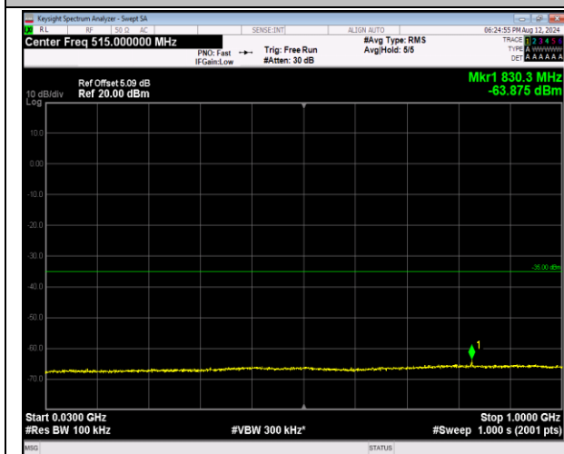
7-7-20MHz-20MHz-16QAM-16QAM-21001-21199-1RB#0 0-0RB#0-30~1000MHz-PASS
