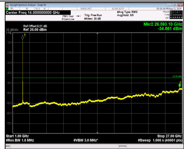
7-7-20MHz-10MHz-16QAM-16QAM-21251-21395-1RB#0 -1RB#49-1000~27000MHz-PASS
