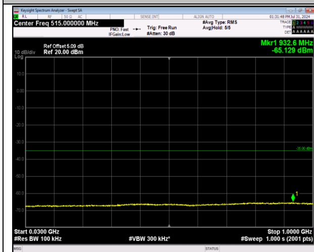
7-7-20MHz-20MHz-64QAM-64QAM-20850-21048-1RB# 99-0RB#0-30~1000MHz-PASS
