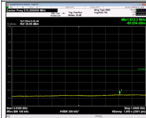
7-7-20MHz-20MHz-64QAM-64QAM-20850-21048-1RB# 0-0RB#0-30~1000MHz-PASS
