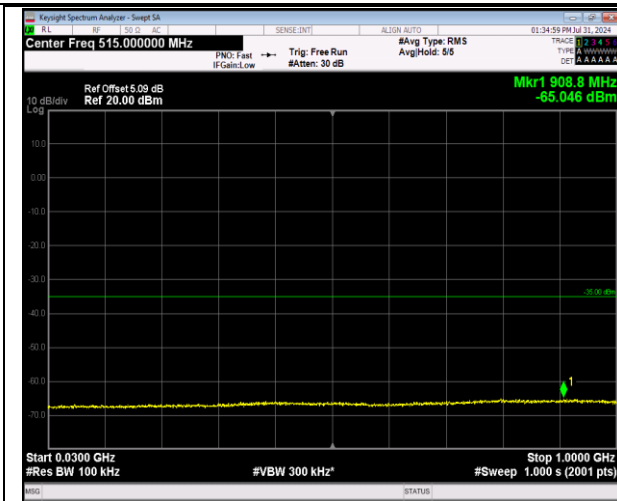
7-7-20MHz-20MHz-64QAM-64QAM-21001-21199-1RB# 0-1RB#99-30~1000MHz-PASS
