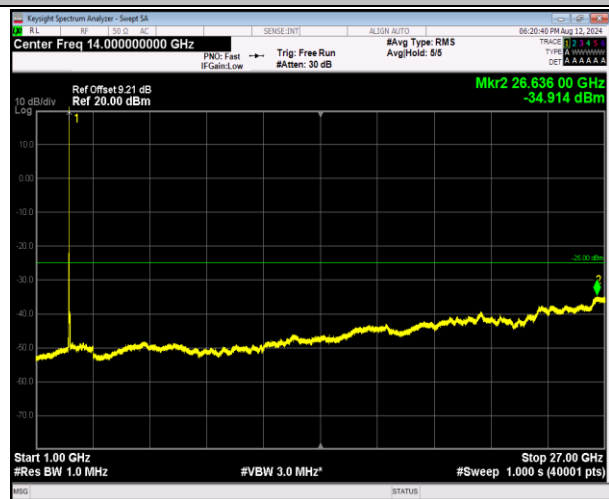
7-7-20MHz-20MHz-QPSK-QPSK-20850-21048-1RB#99-0 RB#0-1000~27000MHz-PASS
