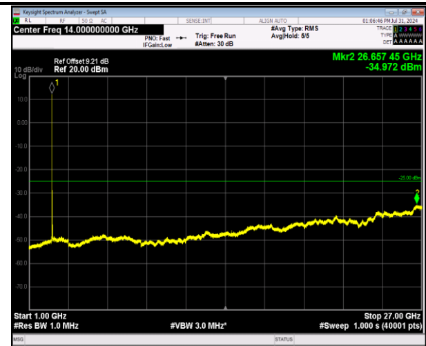
7-7-20MHz-10MHz-64QAM-64QAM-21051-21195-1RB#0- 1RB#49-1000~27000MHz-PASS
