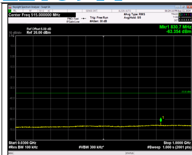
7-7-20MHz-20MHz-QPSK-QPSK-21001-21199-1RB#0-0 RB#0-30~1000MHz-PASS
