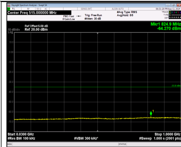
7-7-20MHz-20MHz-16QAM-16QAM-21152-21350-1RB# 99-0RB#0-30~1000MHz-PASS
