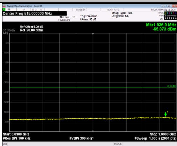
7-7-20MHz-10MHz-16QAM-16QAM-21051-21195-100R B#0-50RB#0-30~1000MHz-PASS
