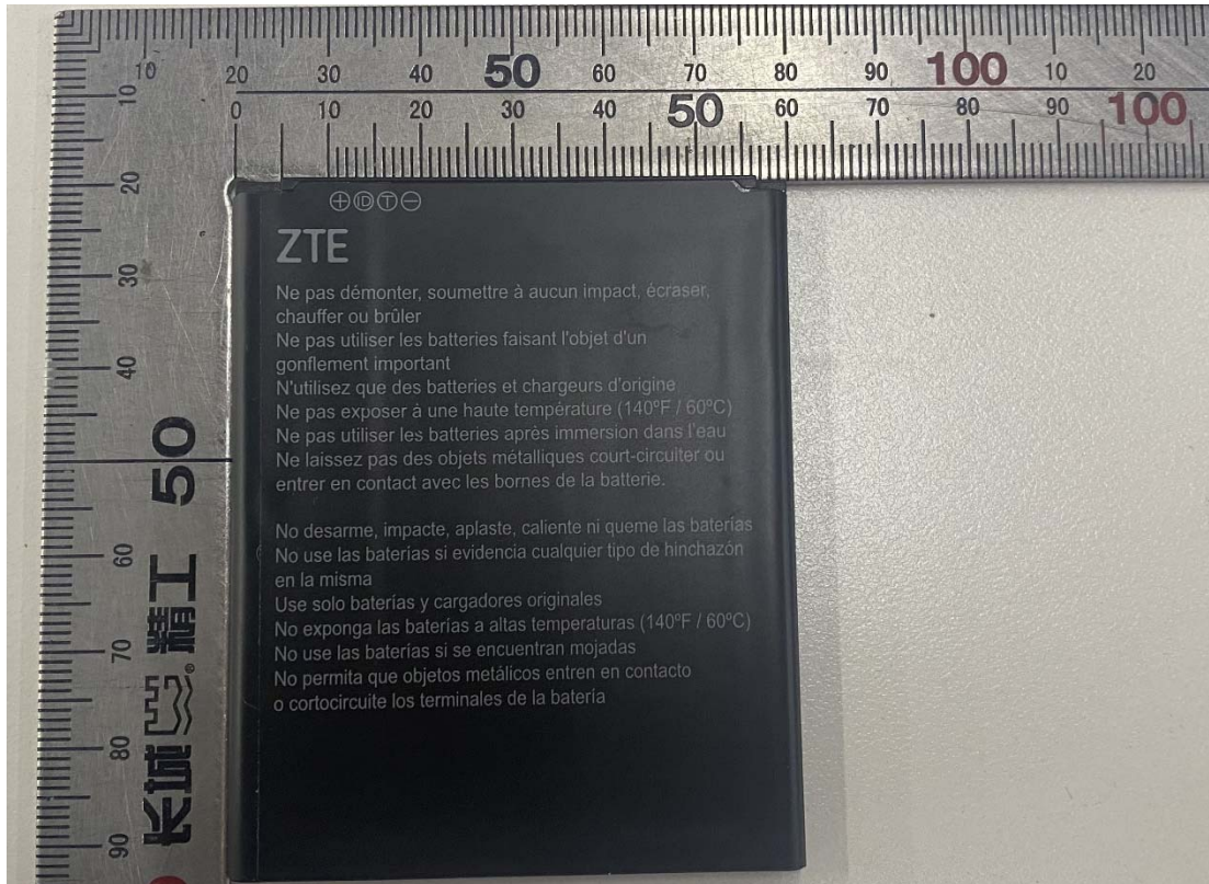
Battery View (LI3930T44P4h486074 made by Guangdong Fenghua New Energy Co.,Ltd.)
